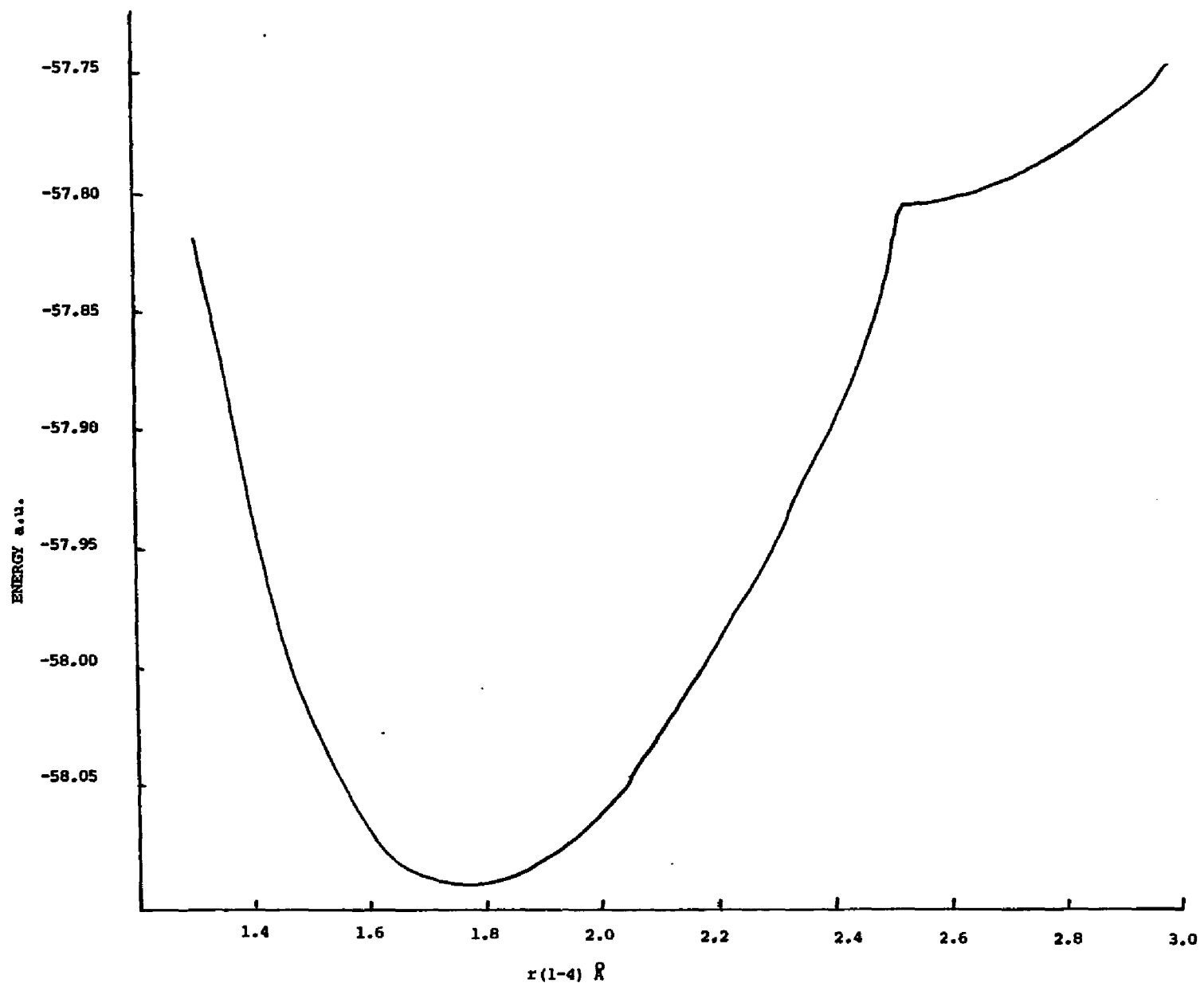
FIGURE 40. ENERGY SURFACE SEGMENT FOR B^{-2} , 44 ELECTRONS
