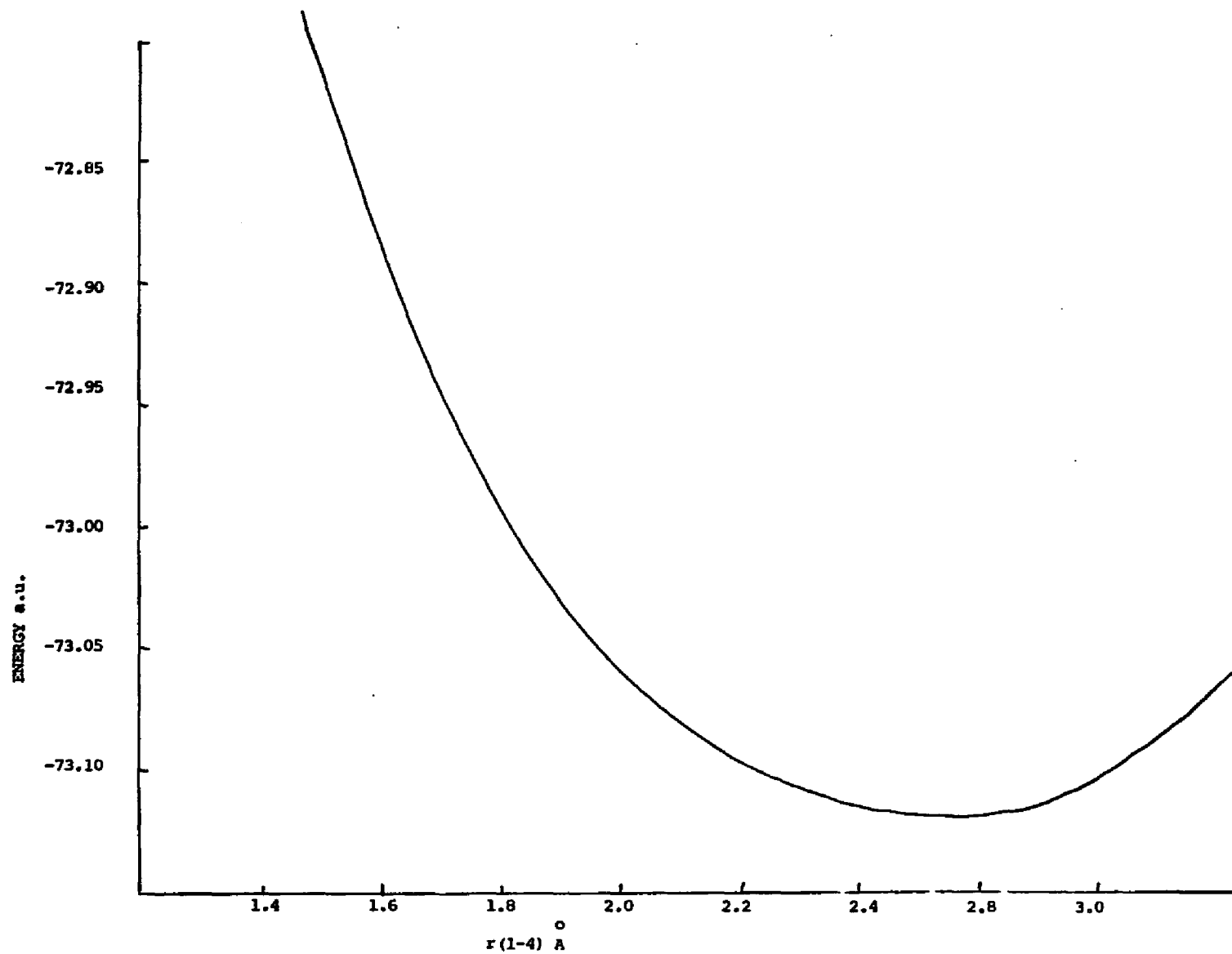
FIGURE 37. ENERGY SURFACE SEGMENT FOR N^0 , 46 ELECTRONS
