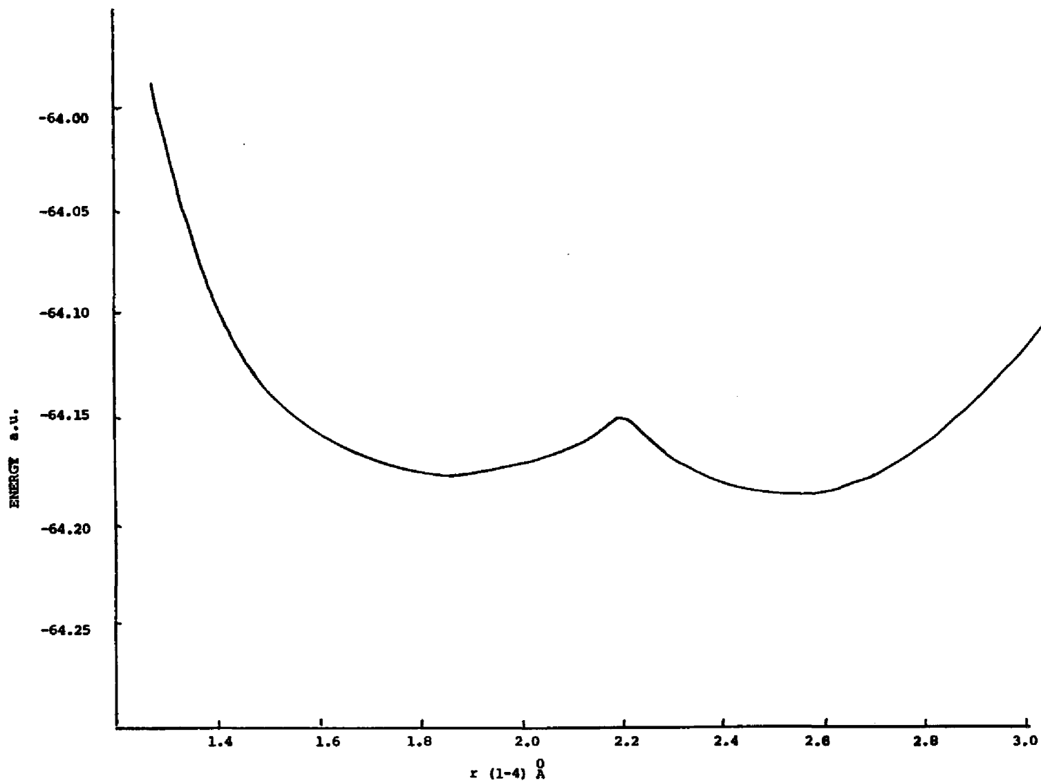
FIGURE 32. ENERGY SURFACE SEGMENT FOR C -1 , 45 ELECTRONS
