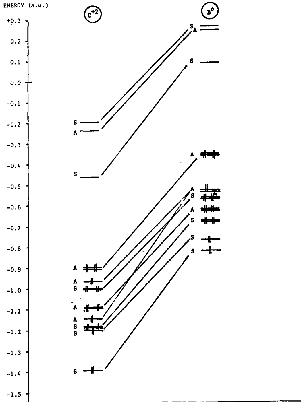
FIGURE 43. ENERGY LEVELS COMPARED FOR C^{+2} AND B^0
