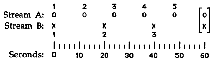
Figure 1.16 - The 5:3 polyrhythm with durations measured in seconds.
