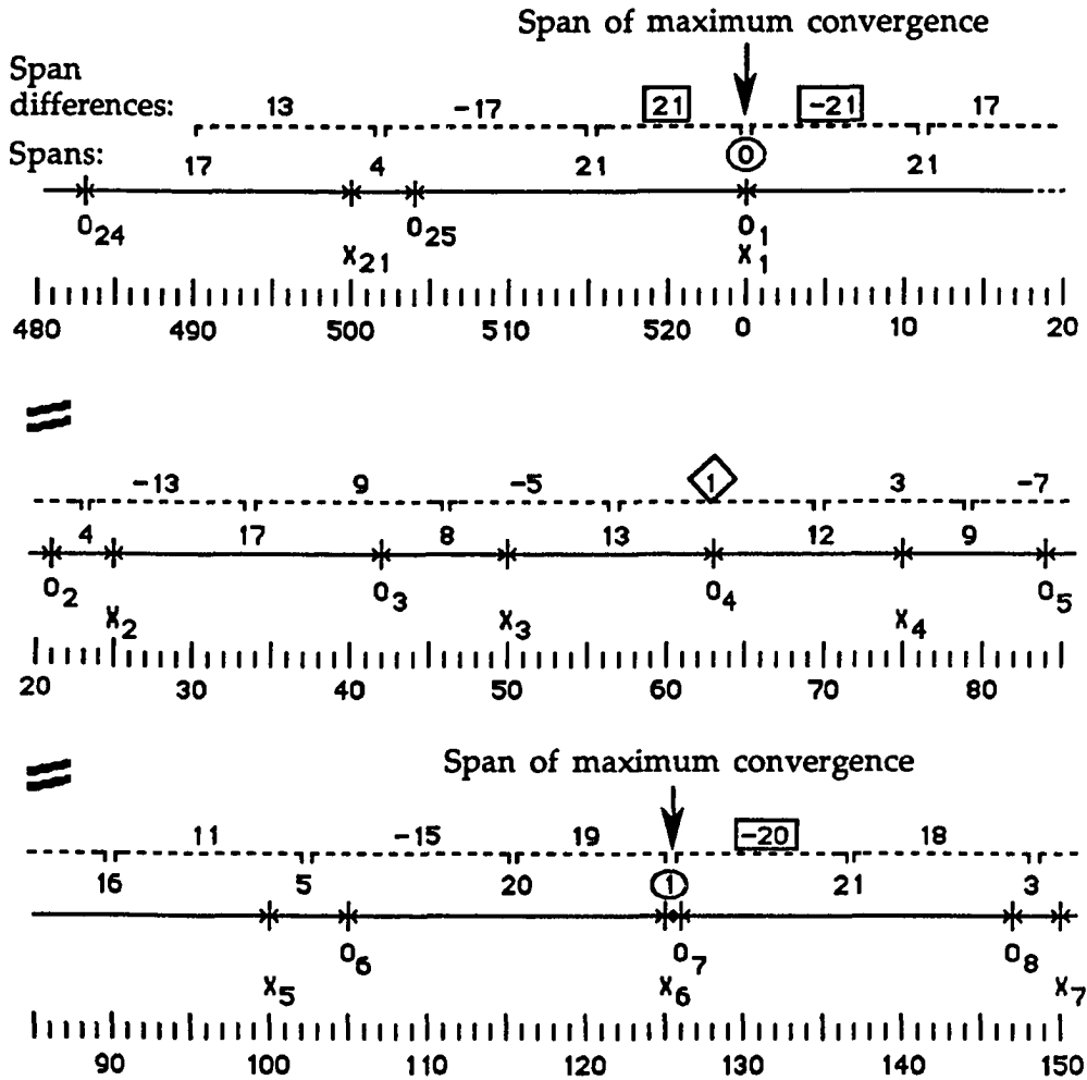
Figure 1.7 - Spans of maximum convergence for a 25:21 polyrhythm.
