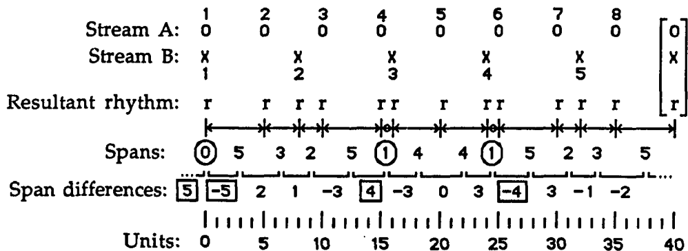
Figure 1.9 - Maximum span differences for a polyrhythm of 8:5
