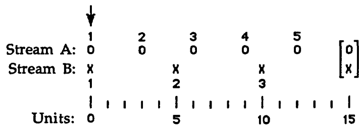
Figure 1.1 - A polyrhythm of 5:3.
