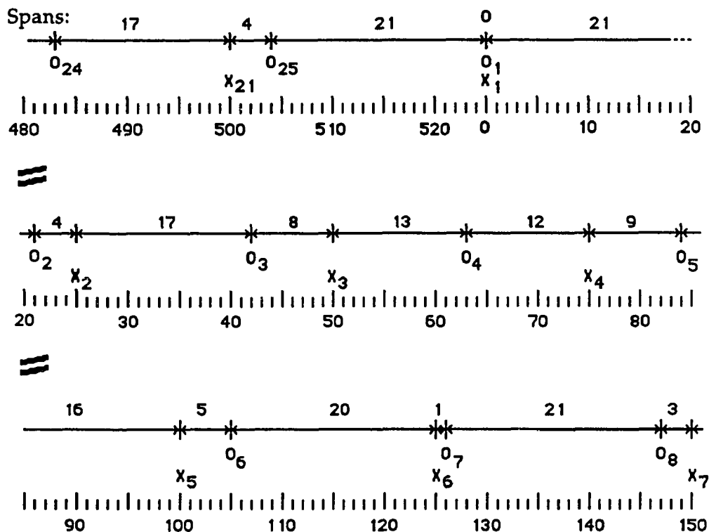
Figure 1.6 - A proximity cycle for the polyrhythm 25:21.
