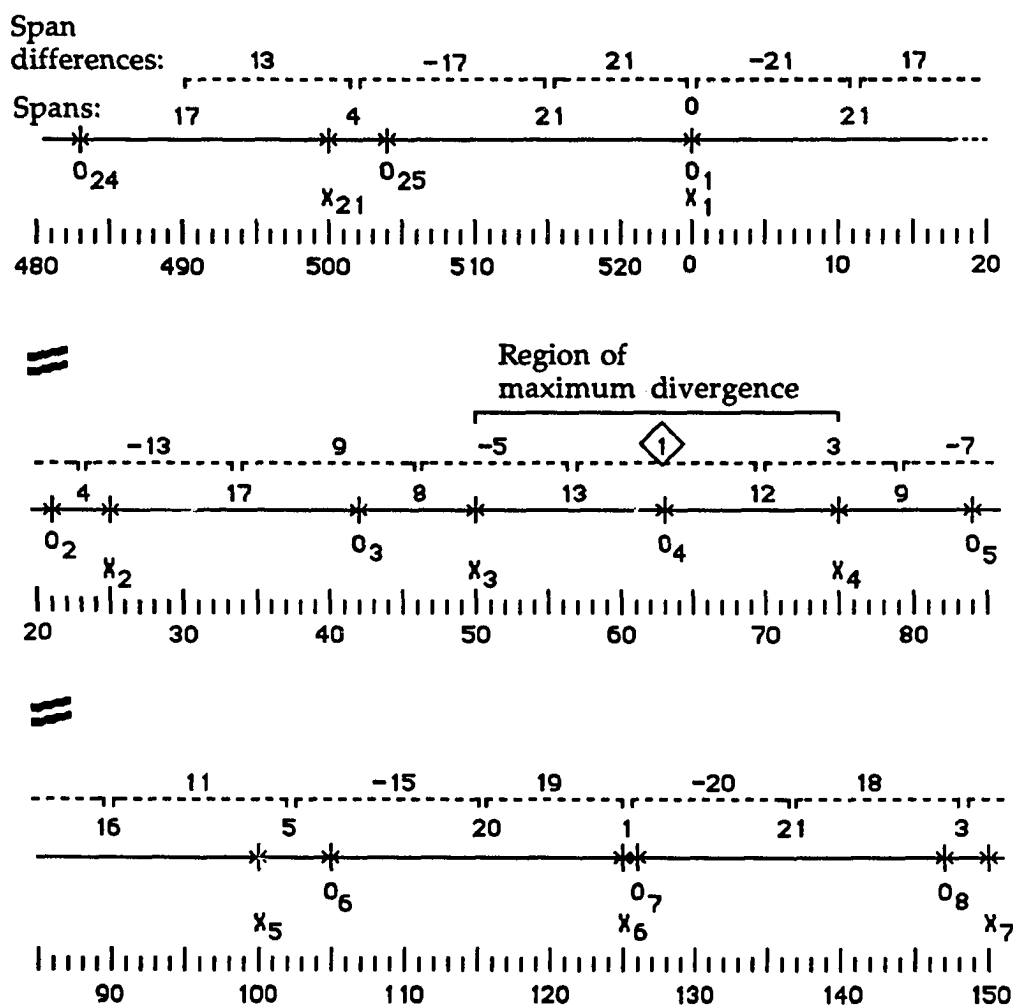
Figure 1.10 - Region of maximum divergence for a 25:21 polyrhythm.
