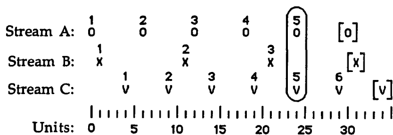
Figure 1.15 - The 5:3:6 polyrhythm re-written to be out of phase.
