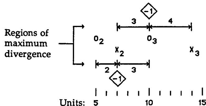
Figure 1.12 - A portion of the 7:5 polyrhythm showing overlapping regions of maximum divergence.
