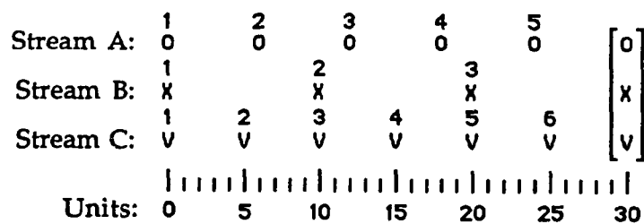
Figure 1.14 - A polyrhythm of 5:3:6 with partial coincidence points.
