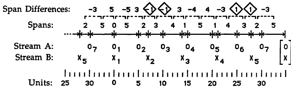
Figure 1.11 - Regions of maximum divergence in a polyrhythm of 7:5
