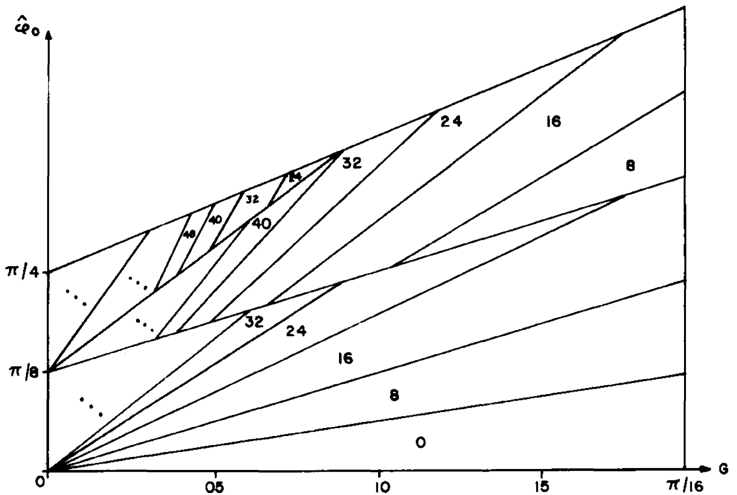
Fig. 3.3-1. The partitioning of the region of Eq. (3.3-1).
