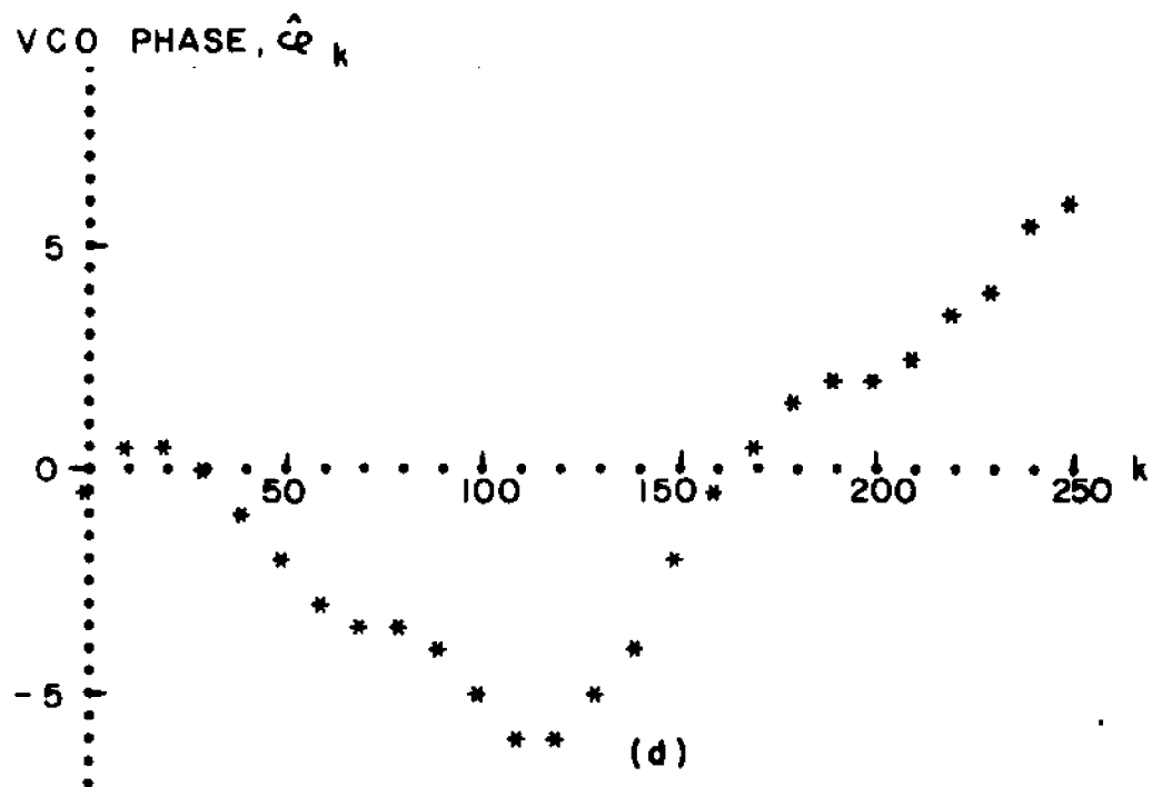
Fig. 4.3-9c,d. Second order DPLL response to constant offset modulation plus a spike of duration (c) 44 samples, (d) 46 samples.
