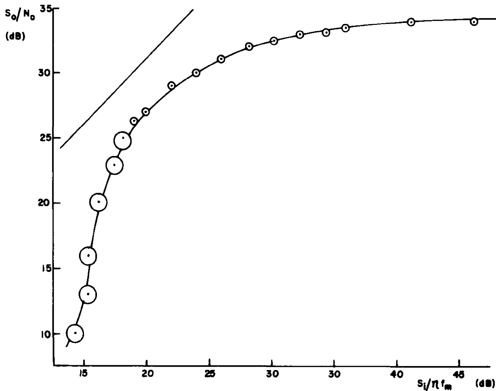
Fig. 4.6-7. Second order DPLL performance with sinusoidal modulation, \beta = 3 , and ten-bit arithmetic.
