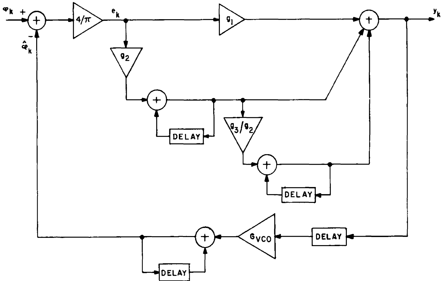
Fig. 5.2-1. The linearized model of the third order DPLL.
