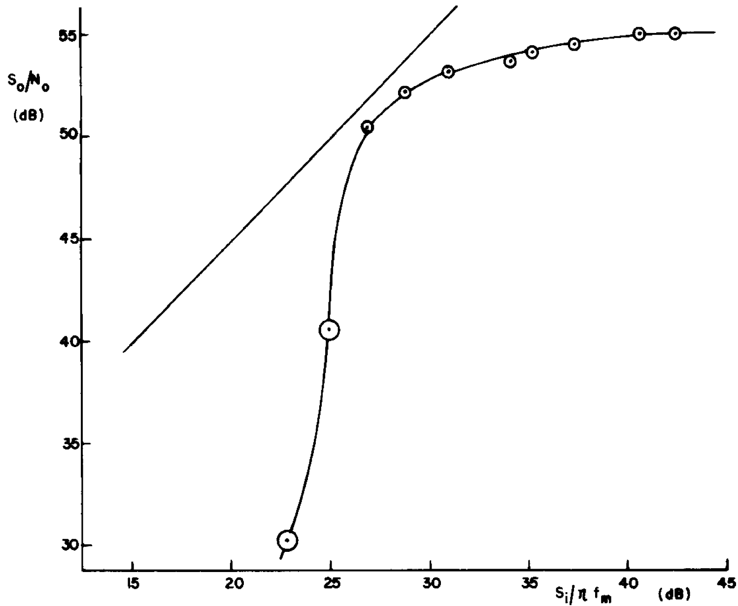
Fig. 3.8-4. First order DPLL performance with constant offset modulation and \beta = 10 .
