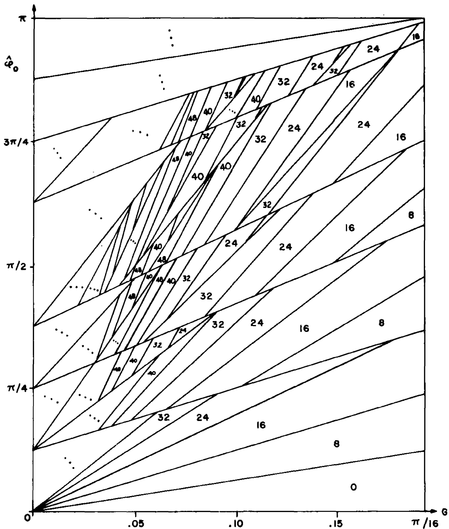
Fig. 3.3-3. Transient time (normalized to the sampling period) as a function of loop gain and positive initial VCO phase for the first order DPLL.
