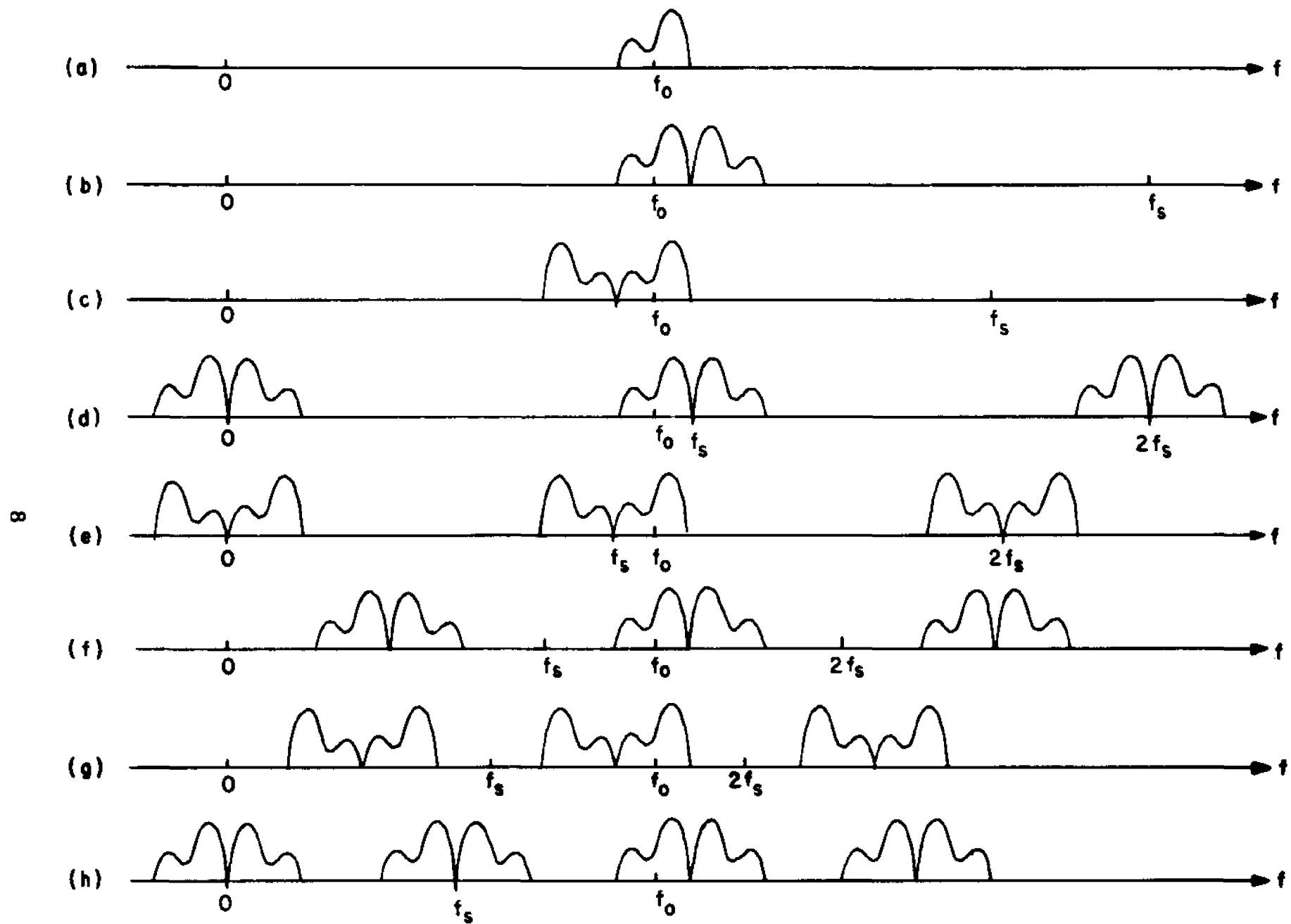
Fig. 2.2-1. Spectra of the bandpass signal and sampled bandpass signal for various sampling frequencies, f_s .
