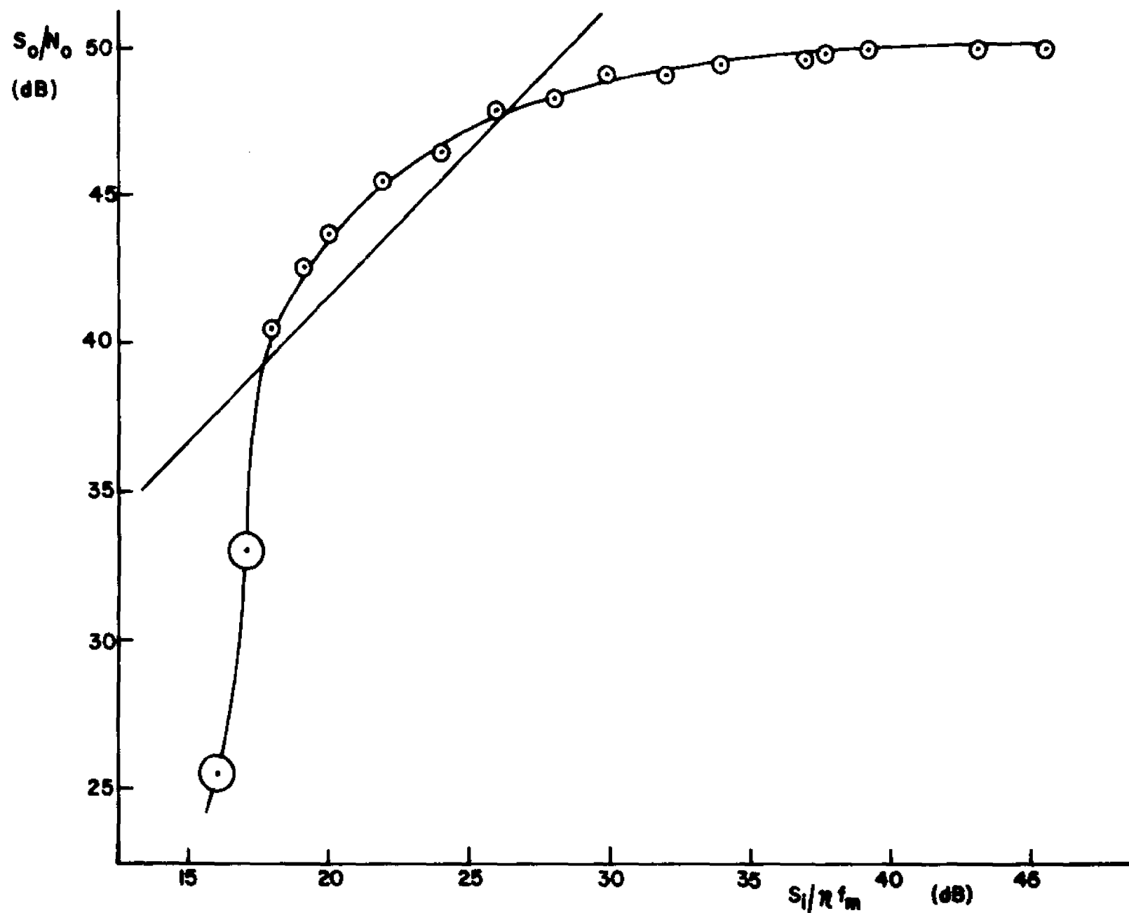
Fig. 4.6-4. Second order DPLL performance with sinusoidal modulation and \beta = 10 .
