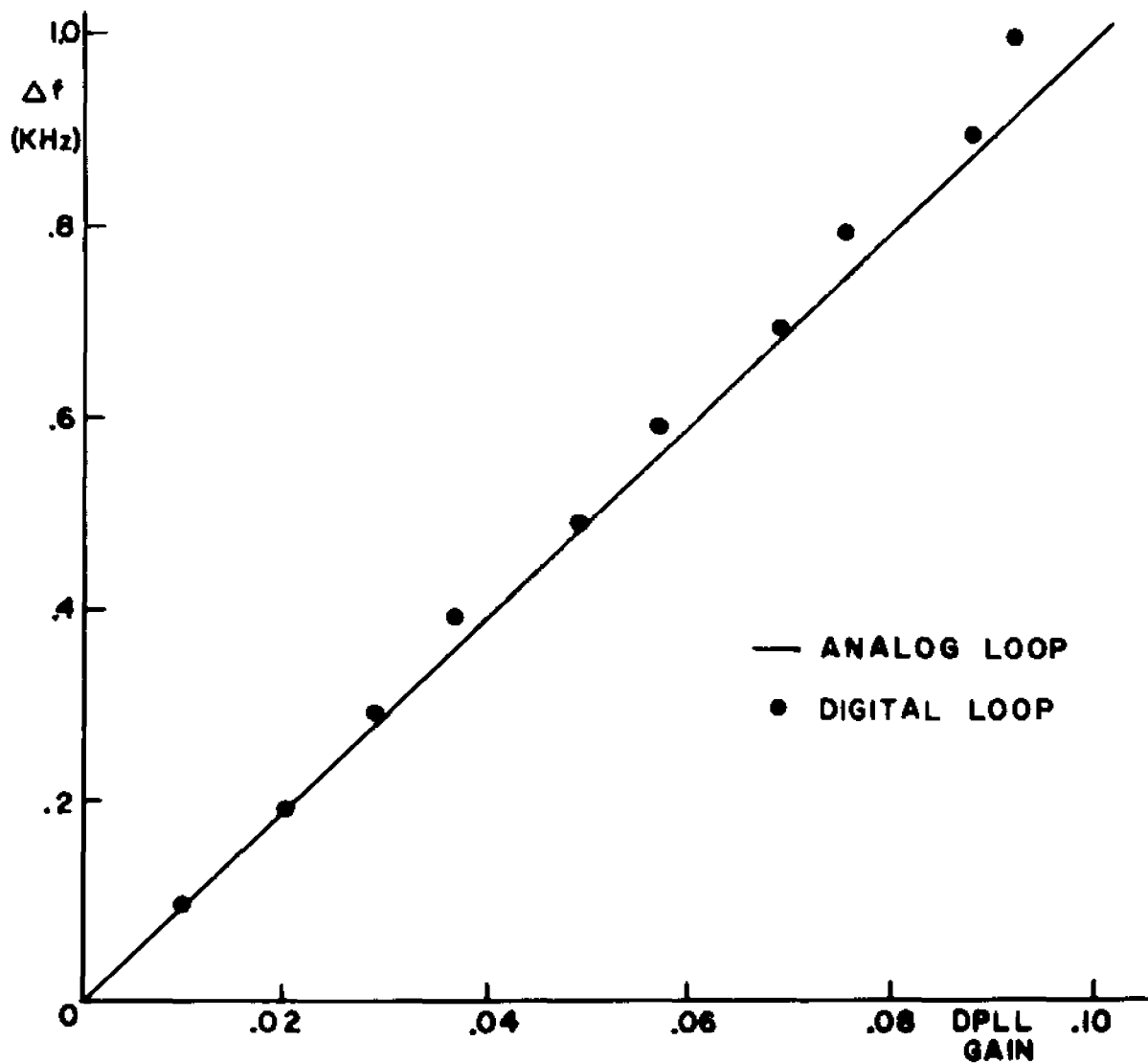
Fig. 3.4-2. Maximum trackable frequency deviation as a function of loop gain for both analog and digital phase-locked loops.
