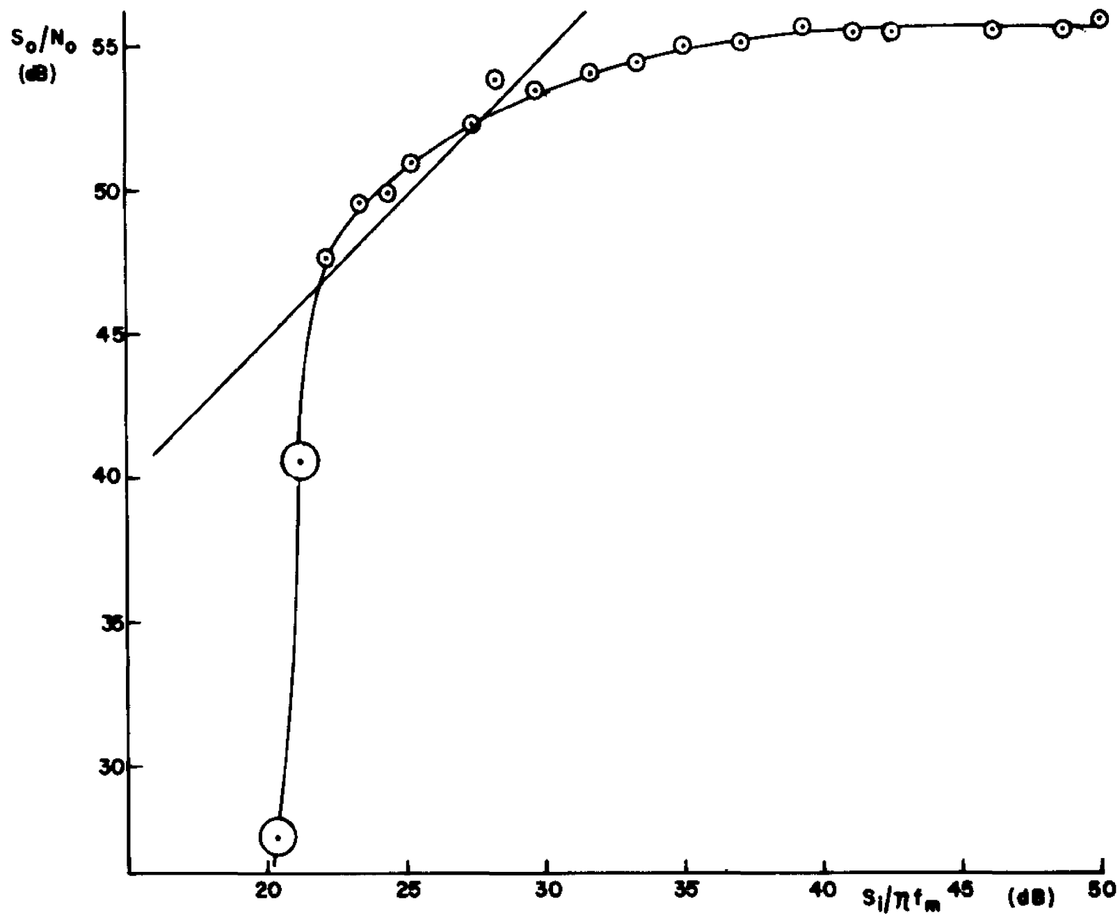
Fig. 4.6-2. Second order DPLL performance with constant offset modulation, \beta = 10 .
