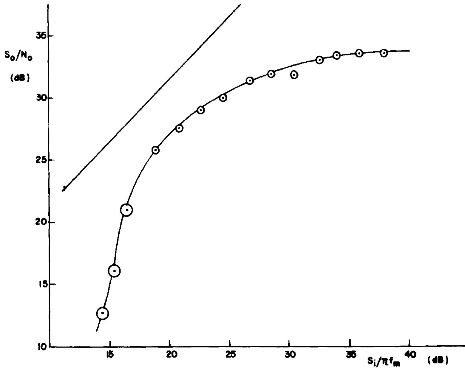
Fig. 3.8-5. First order DPLL performance with sinusoidal modulation and \beta = 3 .
