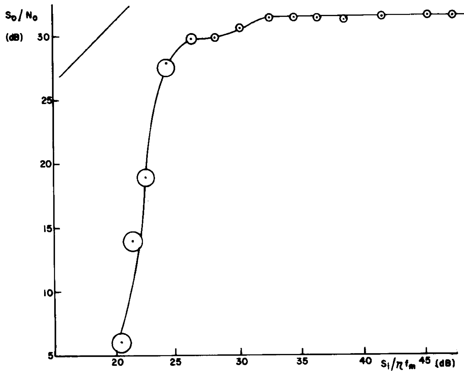
Fig. 5.6-1. Third order DPLL performance with sinusoidal modulation and \beta = 3 .
