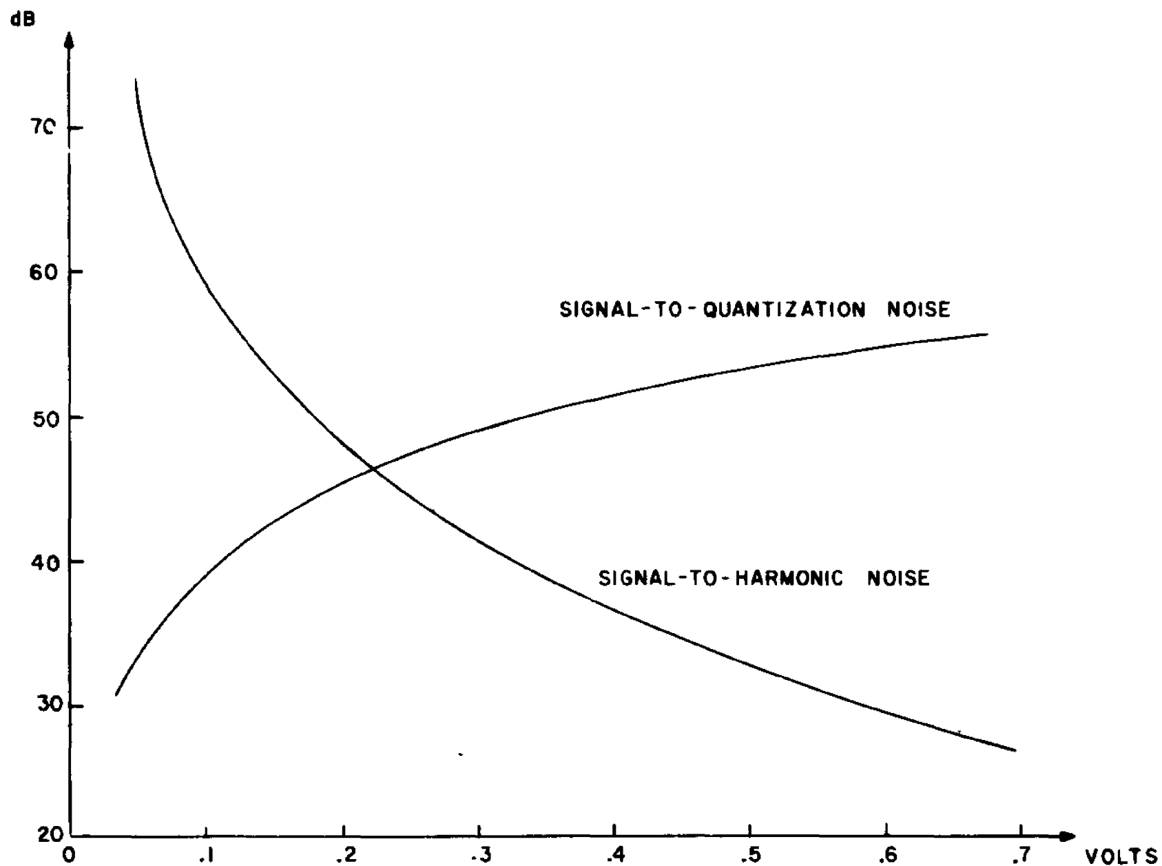
Fig. 2.5-2. Signal-to-quantization noise and signal-to-harmonic noise as a function of the maximum phase difference for a 12-bit A/D converter.
