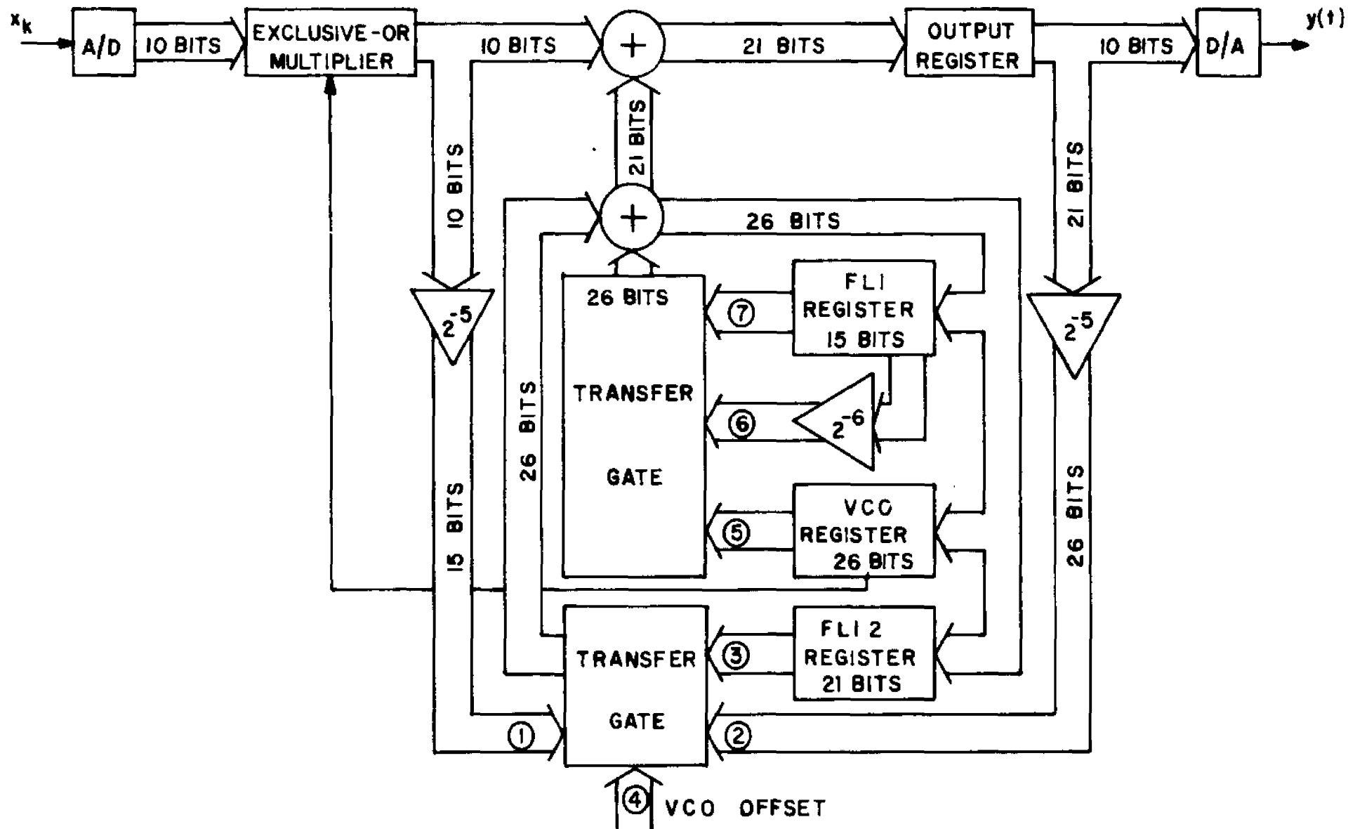
Fig. 5.4-2a. Schematic diagram of the third order DPLL.
