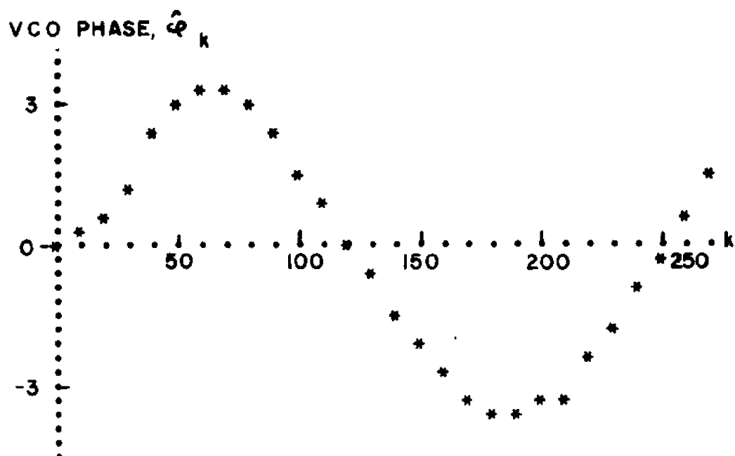
Fig. 4.3-4. Second order DPLL response to sinusoidal modulation plus a 32-sample, constant amplitude spike.
