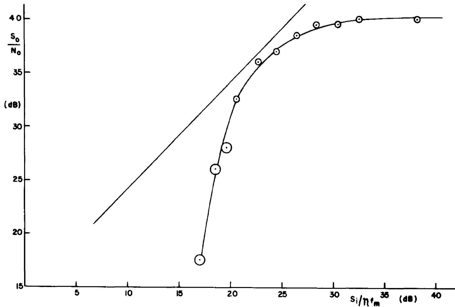
Fig. 3.8-3. First order DPLL performance with constant offset modulation and \beta = 3 .
