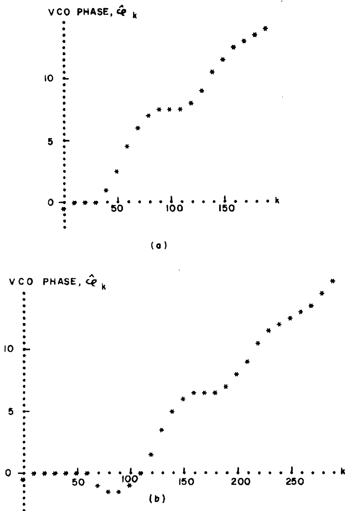
Fig. 4.3-10a,b. Second order DPLL response to constant offset modulation plus a spike of duration (a) 32 samples, (b) 38 samples.
