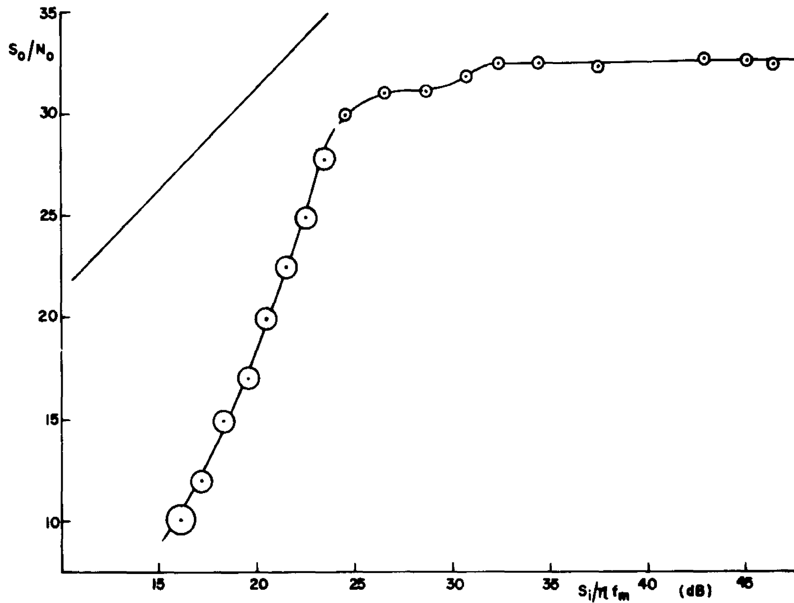
Fig. 3.8-7. First order DPLL performance with sinusoidal modulation, \beta = 3 , and a three-bit A/D converter.
