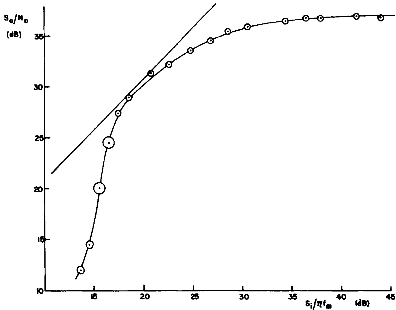
Fig. 4.6-3. Second order DPLL performance with sinusoidal modulation and \beta = 3 .
