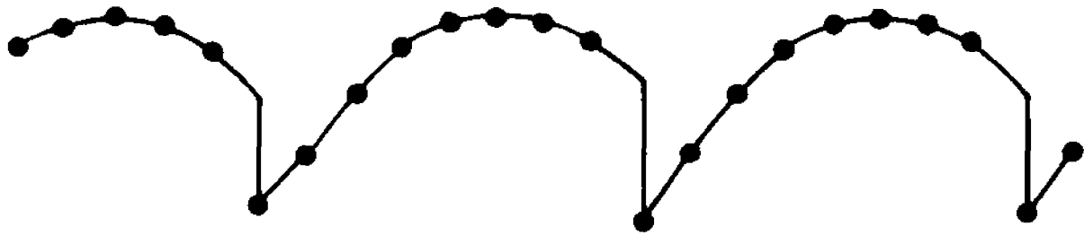
Fig. 3.4-1. Typical phase error sequence when the input frequency is deviated from the carrier frequency.
