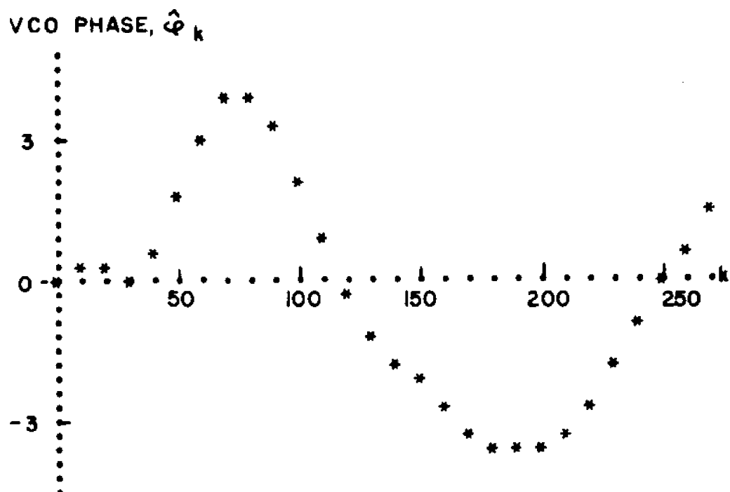
Fig. 4.3-5. Second order DPLL response to sinusoidal modulation plus a 40-sample, constant amplitude spike.
