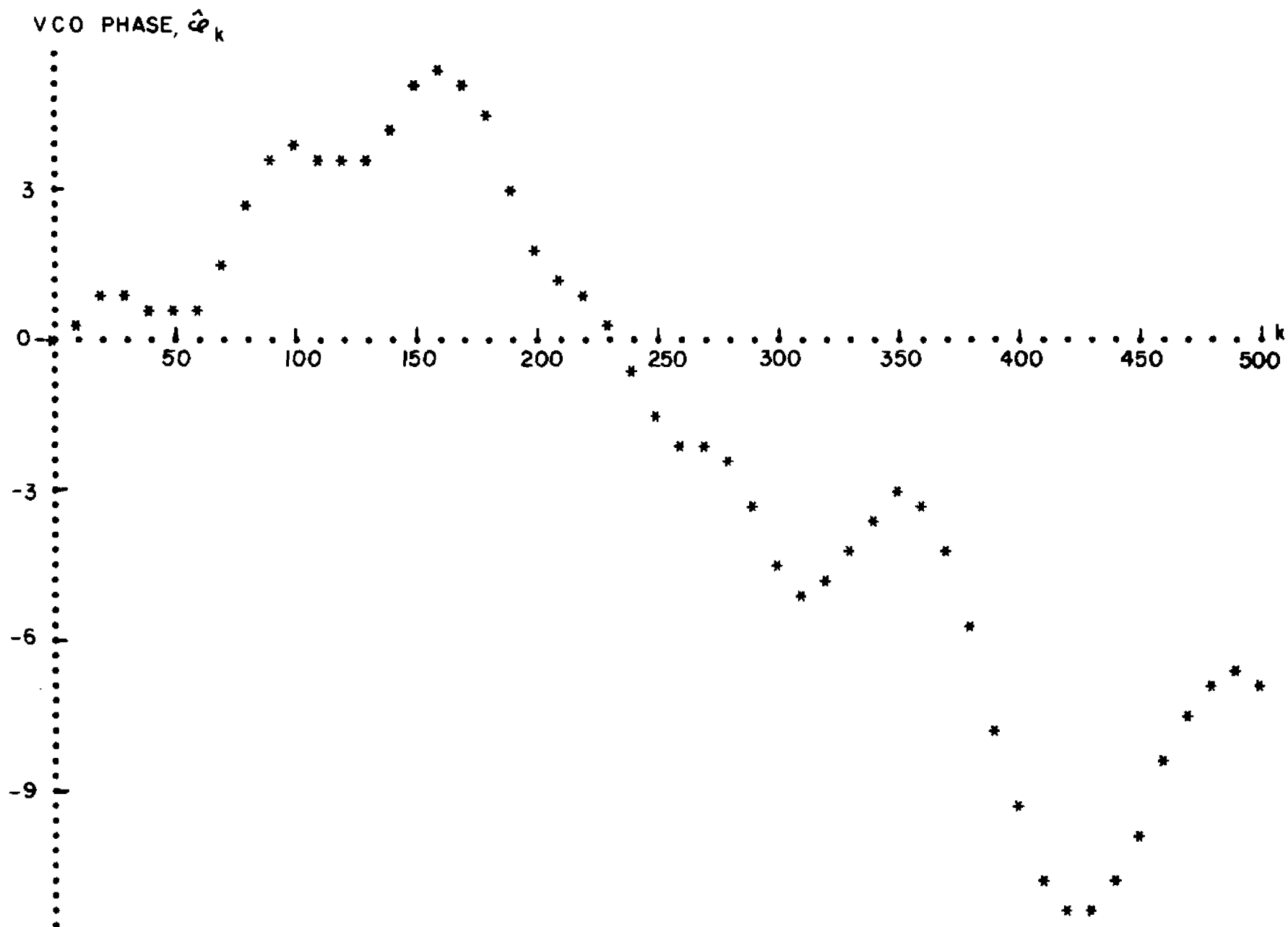
Fig. 4.3-8. Second order DPLL response to sinusoidal modulation plus a 60-sample, one volt minimum amplitude spike.
