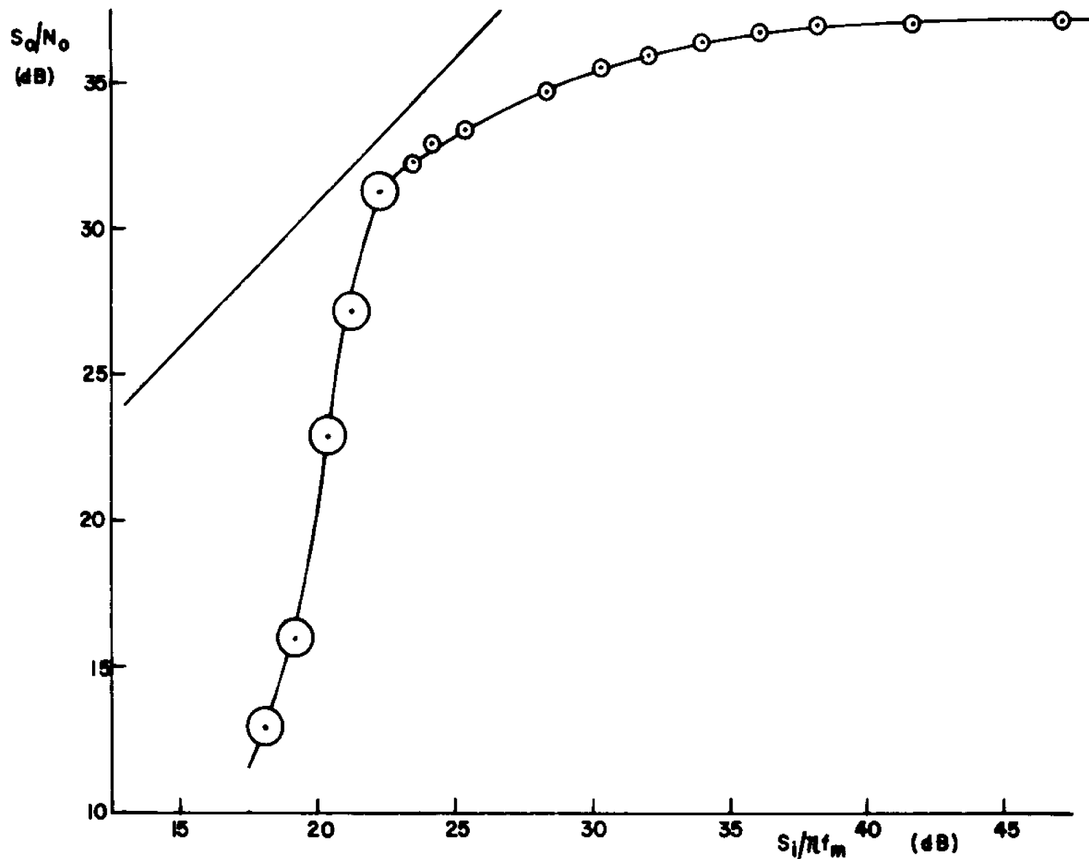
Fig. 4.6-5. Second order DPLL performance with sinusoidal modulation, \beta = 3 , and a three-bit A/D converter.
