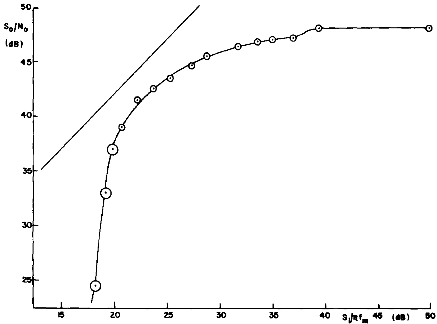
Fig. 3.8-6. First order DPLL performance with sinusoidal modulation and \beta = 10 .
