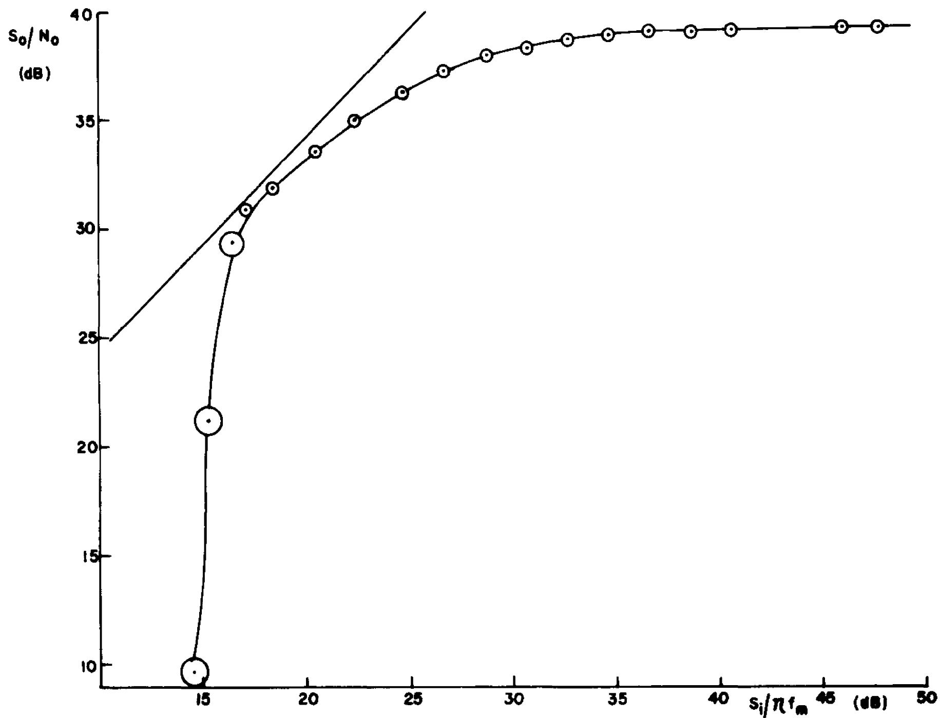
Fig. 5.6-3. Third order DPLL performance with constant offset modulation and \beta = 3 .
