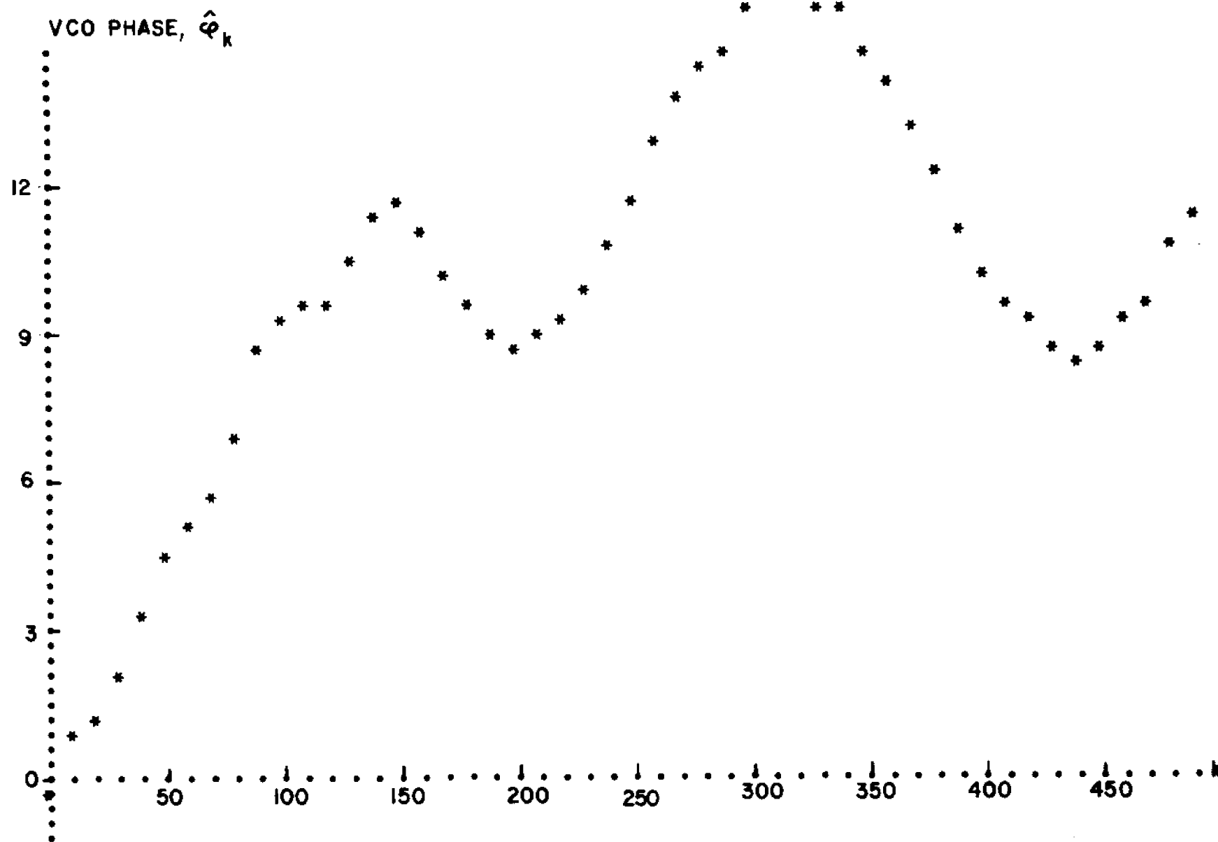
Fig. 5.3-4b. Third order DPLL response to sinusoidal modulation plus a 70-sample, 0.2 volt minimum amplitude spike.
