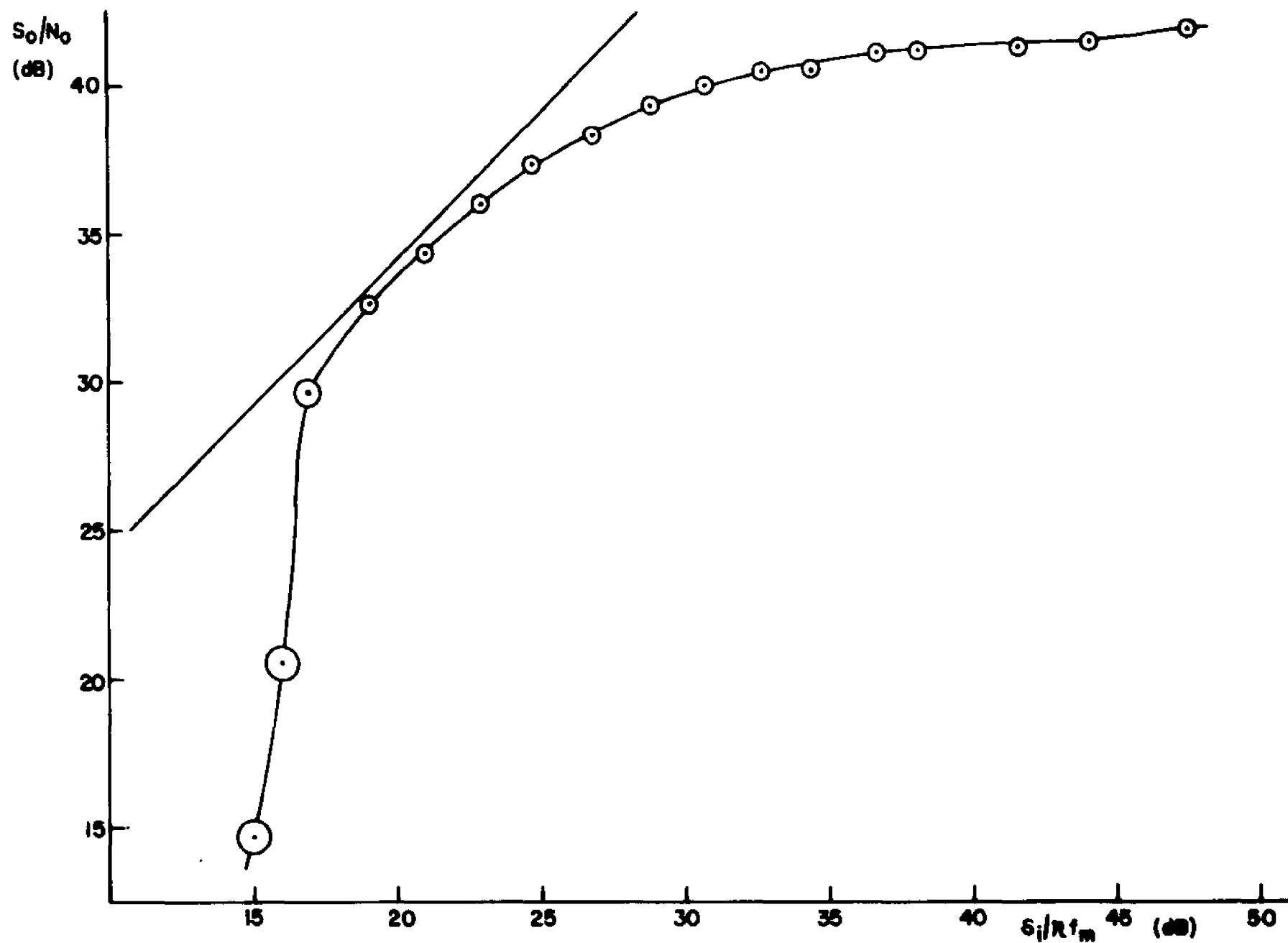
Fig. 4.6-1. Second order DPLL performance with constant offset modulation and \beta = 3 .
