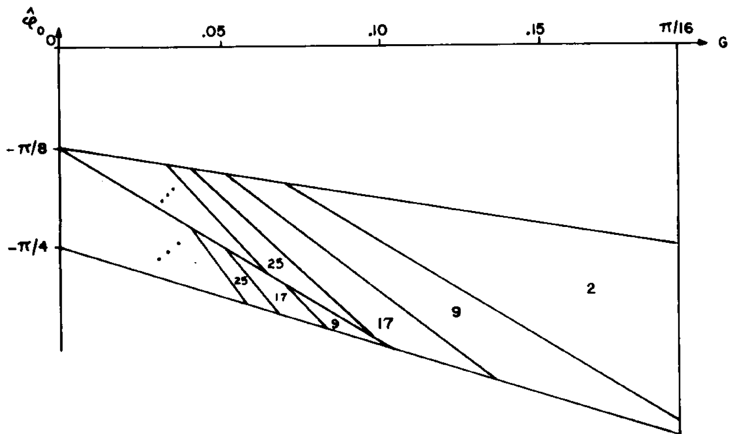
Fig. 3.3-5. The regions of Fig. 3.3-4 shifted down and their associated transient times.
