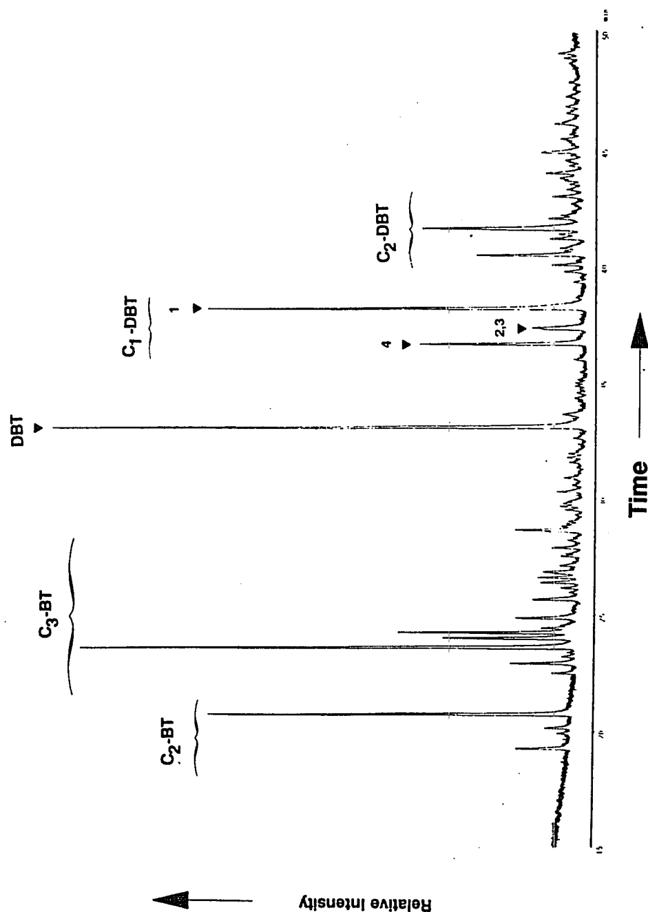
Fig. 42: Distribution patterns of selected sulfur aromatic compounds. The pattern is representative for the marls of type A, laminated anhydrite and lenticular anhydrite lithofacies. ( C_2 -BT = dimethylbenzothiophenes, C_3 -BT = trimethylbenzothiophenes, DBT = dibenzothiophene, C_1 -DBT = methyl dibenzothiophenes, C_2 -DBT = dimethyldibenzothiophenes).
