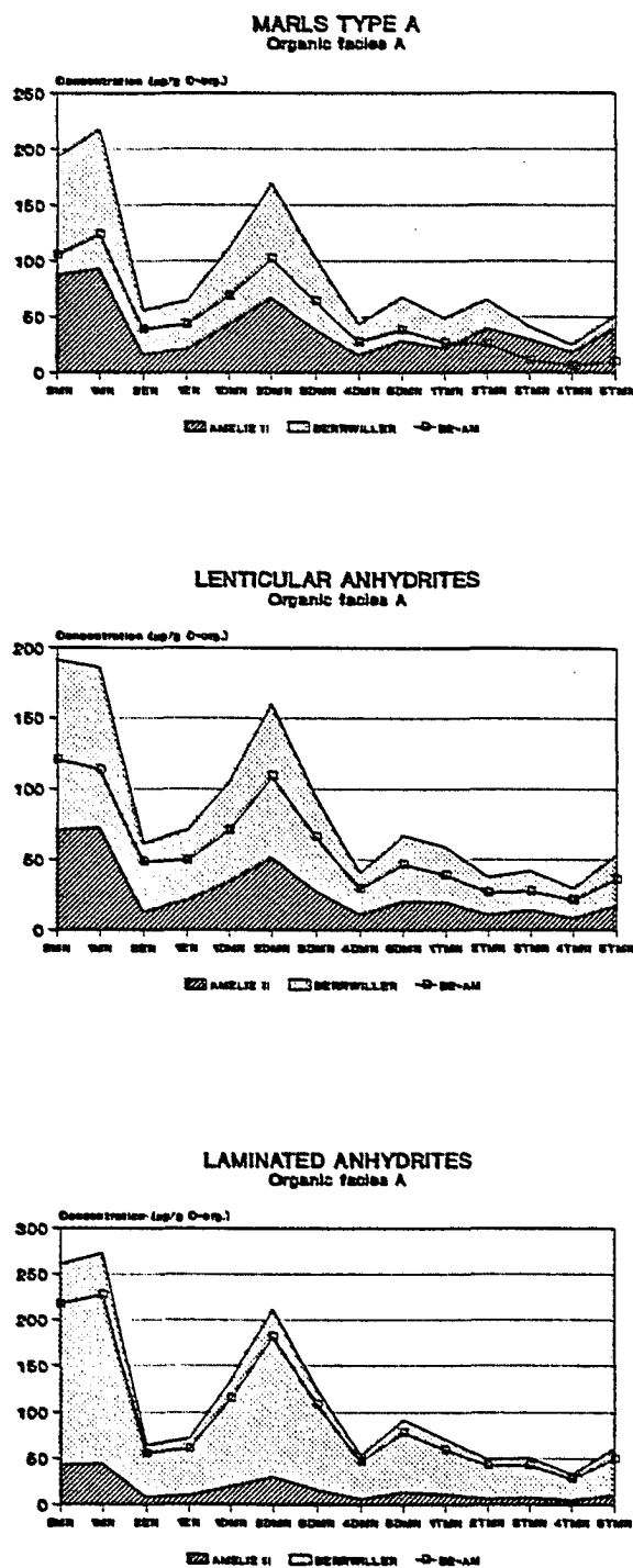
Fig. 72: Average naphthalene concentration pattern and absolute yield increase (BE - AM) of the lithofacies of the S unit. (Continued on following page.)
