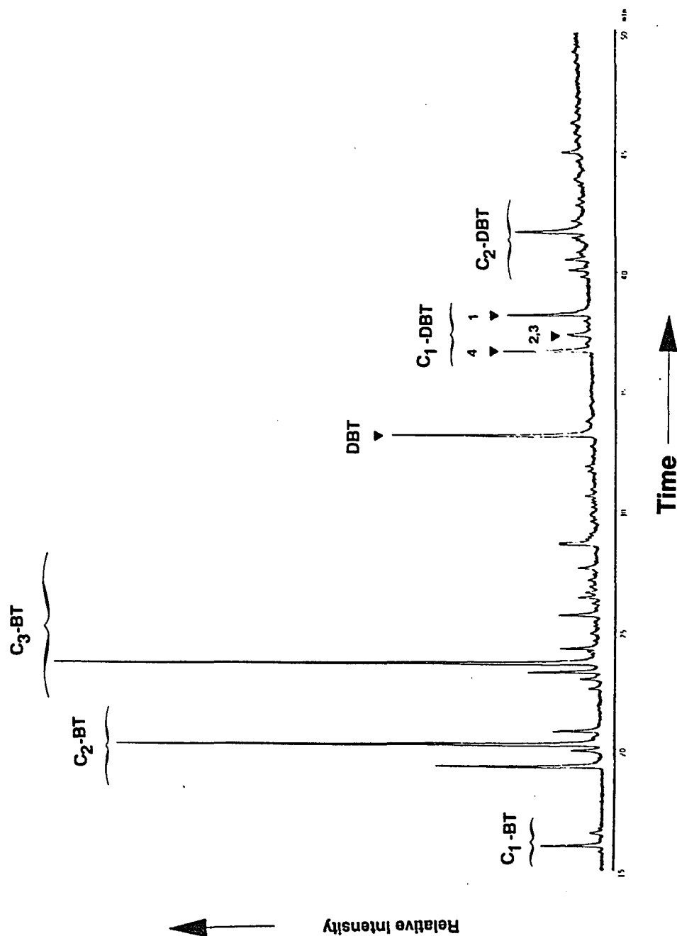
Fig. 43: Distribution patterns of selected sulfur aromatic compounds. The pattern is representative for the marl of type B, massive anhydrite and halite lithofacies. (C 2 -BT = dimethylbenzothiophenes, C 3 -BT = trimethylbenzothiophenes, DBT = dibenzothiophene, C 1 -DBT = methyl dibenzothiophenes, C 2 -DBT = dimethyldibenzothiophenes).
