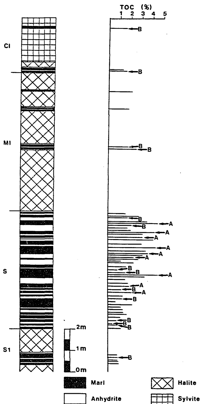
Fig. 44: TOC content of the marl beds at Amelie II. Note the cyclic increase and decrease of the organic carbon content from S1 to the CI unit. The samples marked with A and B refer to samples containing organic facies A and B.
