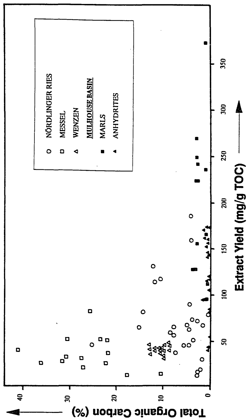
Fig. 78: Comparison of the extract yields of the lithofacies of the S unit with other immature source rocks.
