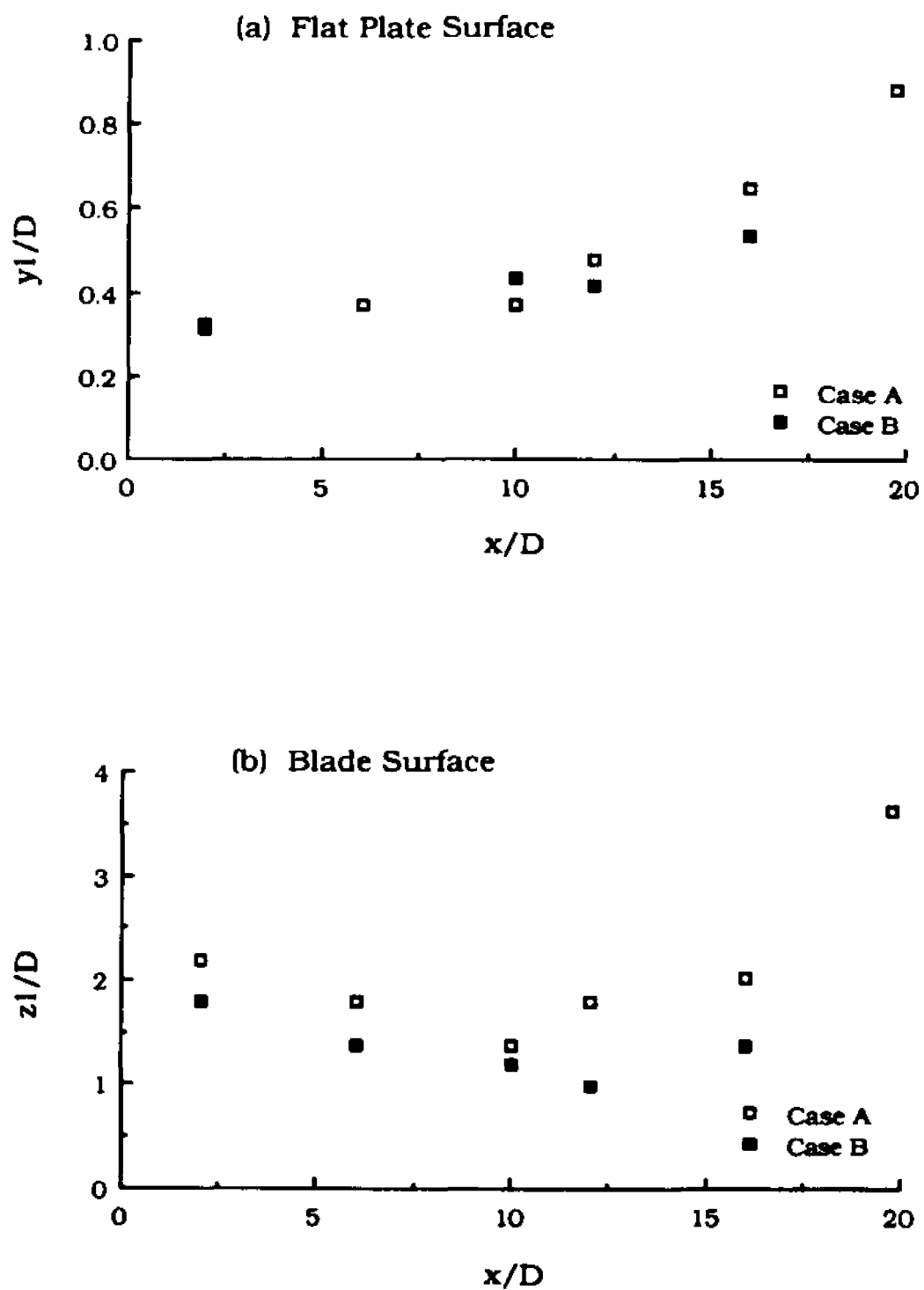
Fig. 5.39 Variation of the Location of Maximum Wall Shear Stress- A Comparison Between Case A and Case B
