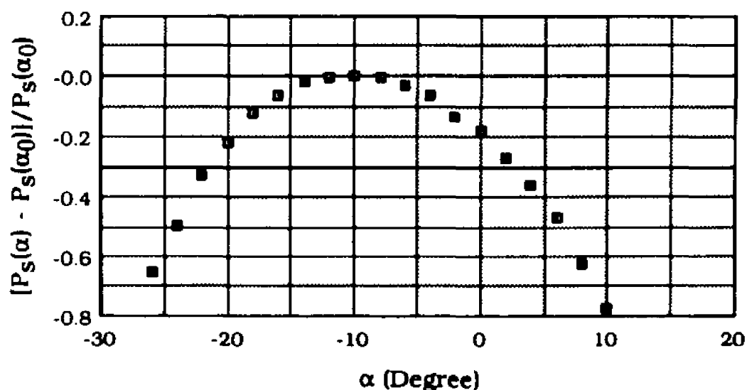
(b) Error as a Fraction of Surface Static Tube Pressure When Aligned in Local Flow Direction
