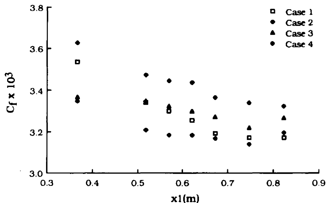
(a) Variation of C_f as a Function of Streamwise Distance
