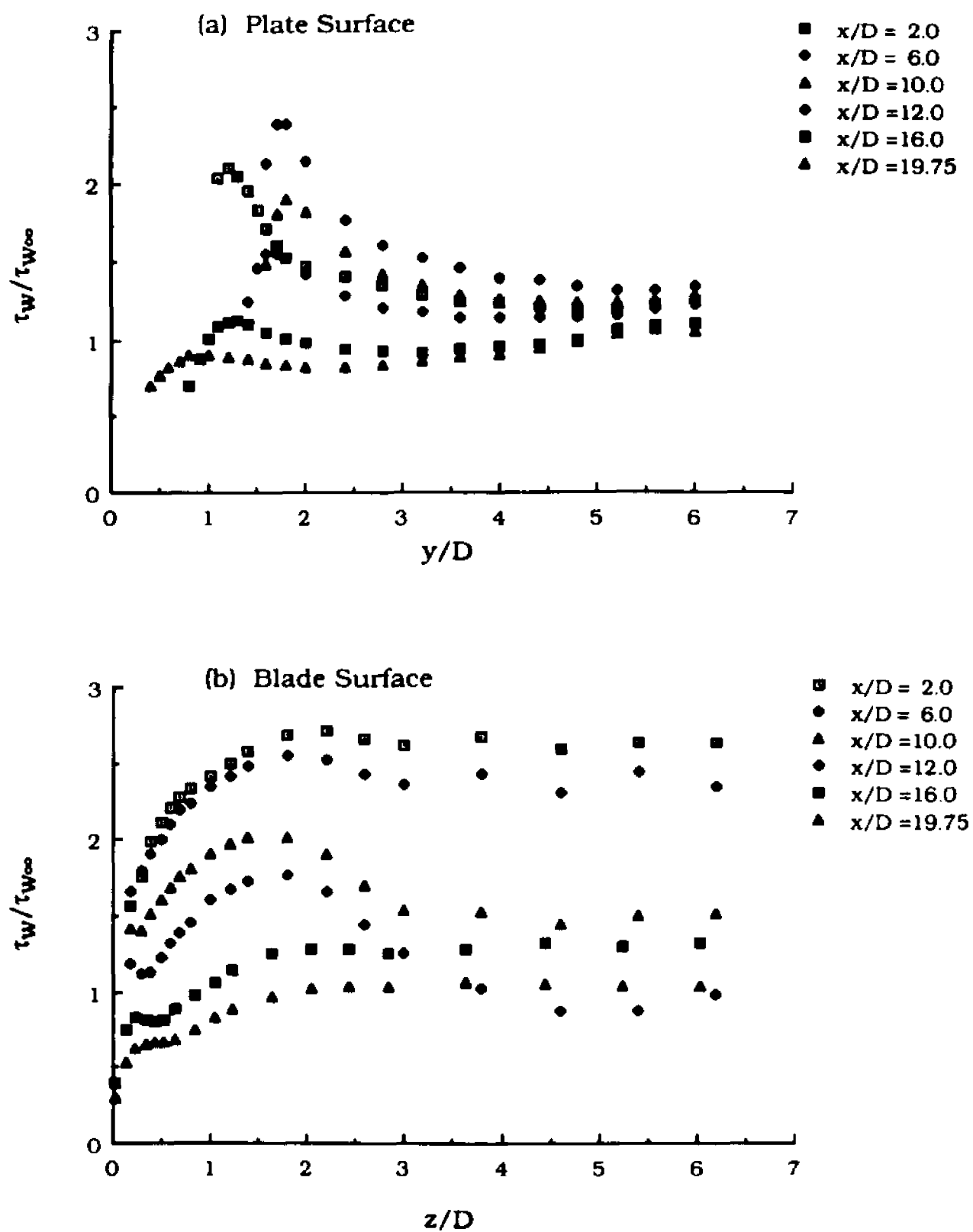
Fig. 5.23 Wall Shear Stress Variation in Blade End-Wall Corner Region for Case A
