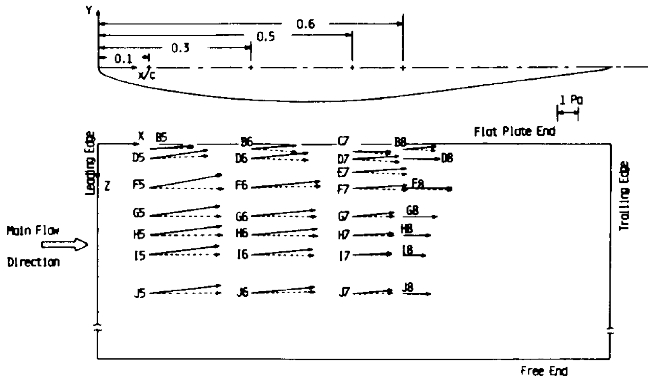
(b) Airfoil Surface
