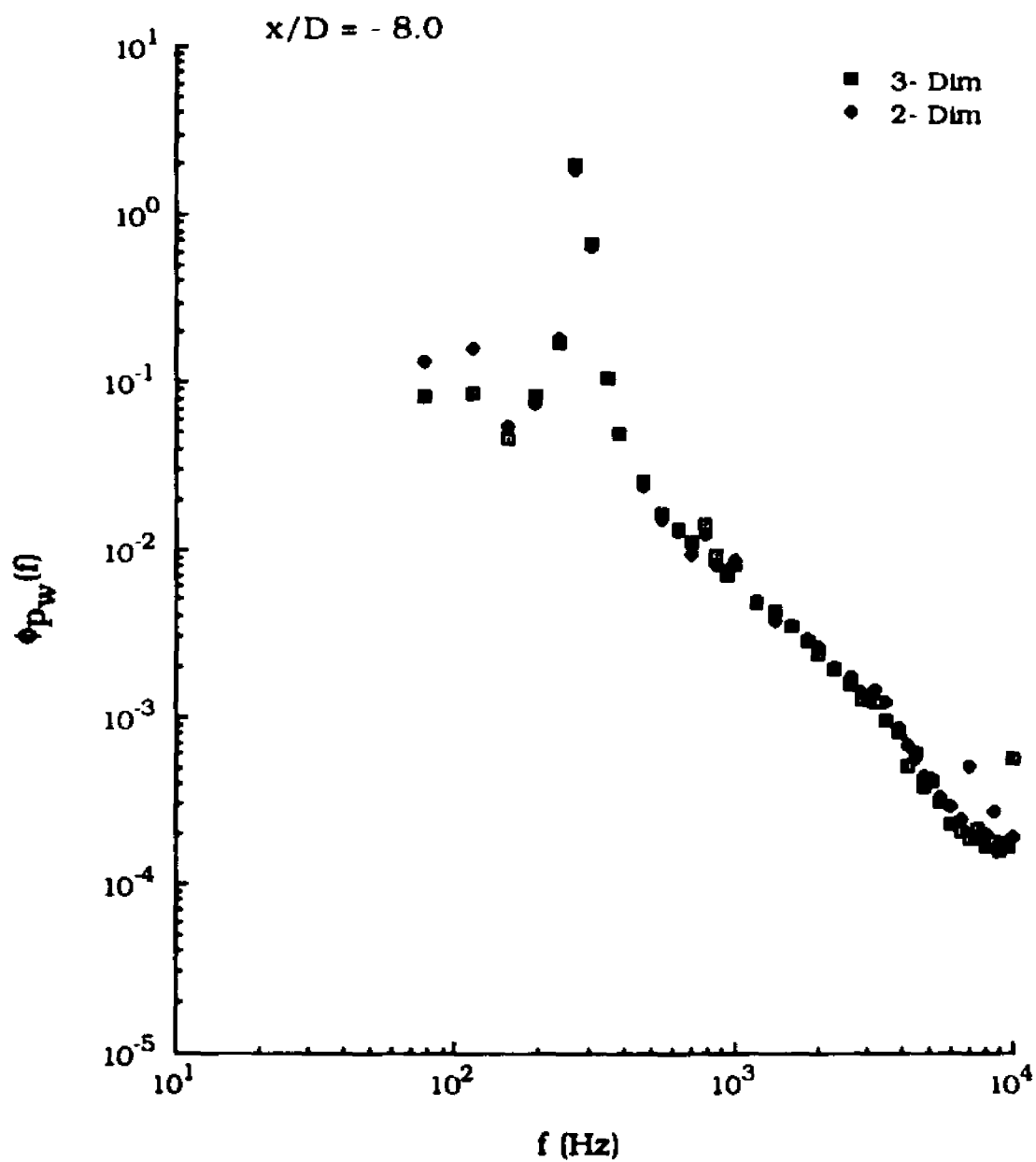
Fig. 6.3 Frequency Spectral Distribution of Wall Pressure Fluctuation Upstream of the Blade Leading Edge
