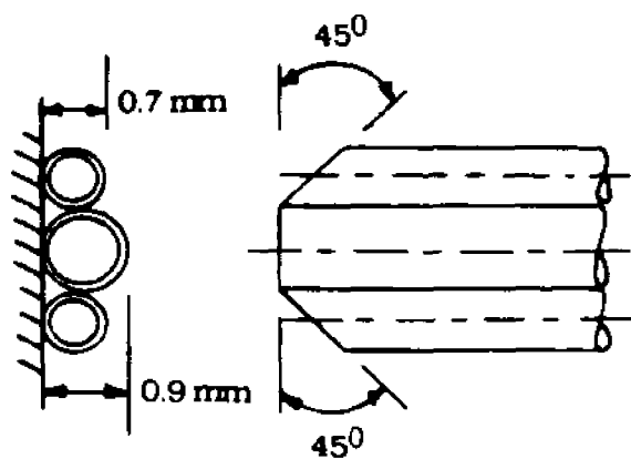
(b) Chamfered Type
