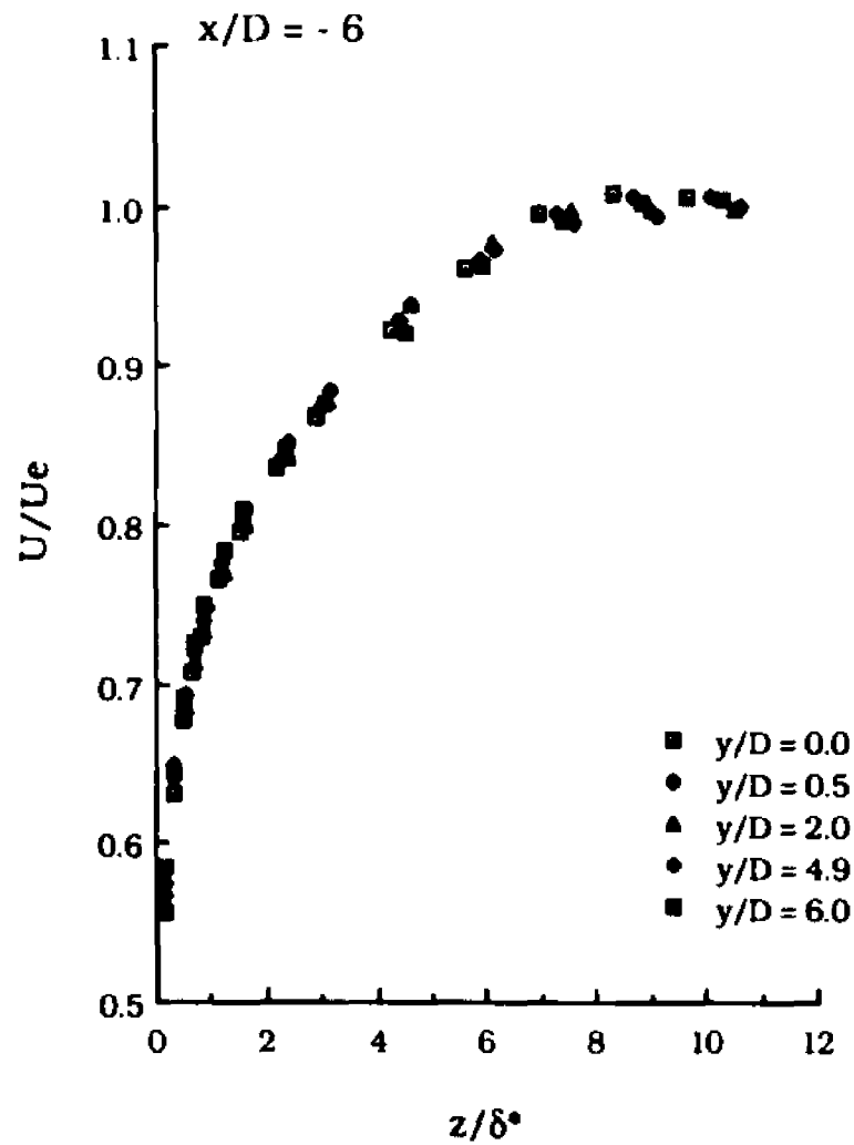
(a) In Outer-Layer Variables
