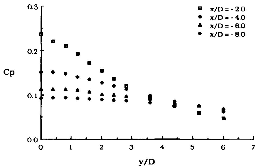
Fig. 5.3 Surface Static Pressure Distribution Upstream of the Blade Leading Edge
