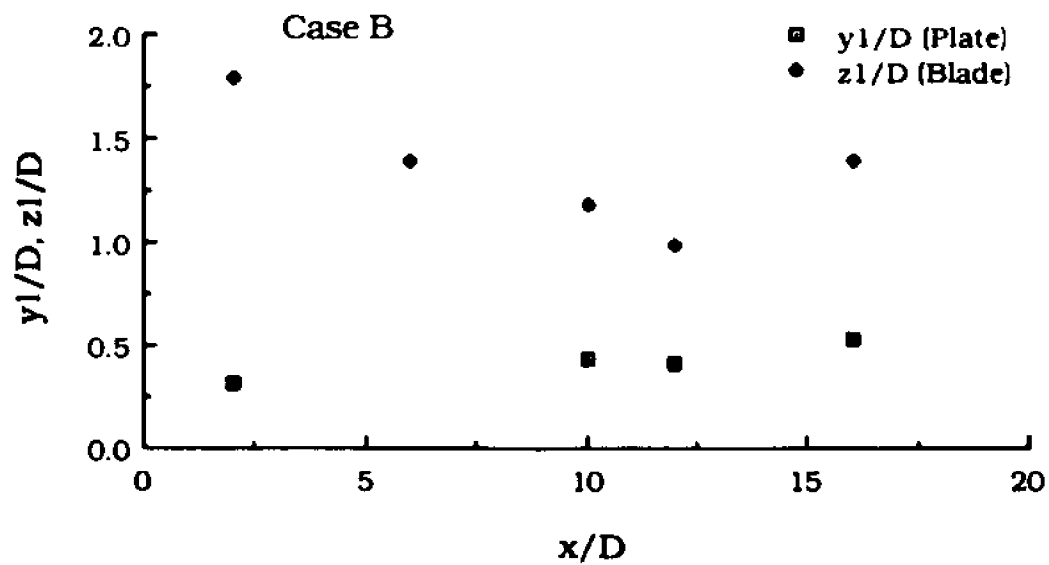
Fig. 5.31 Variation of the Location of Maximum Wall Shear Stress for Case B
