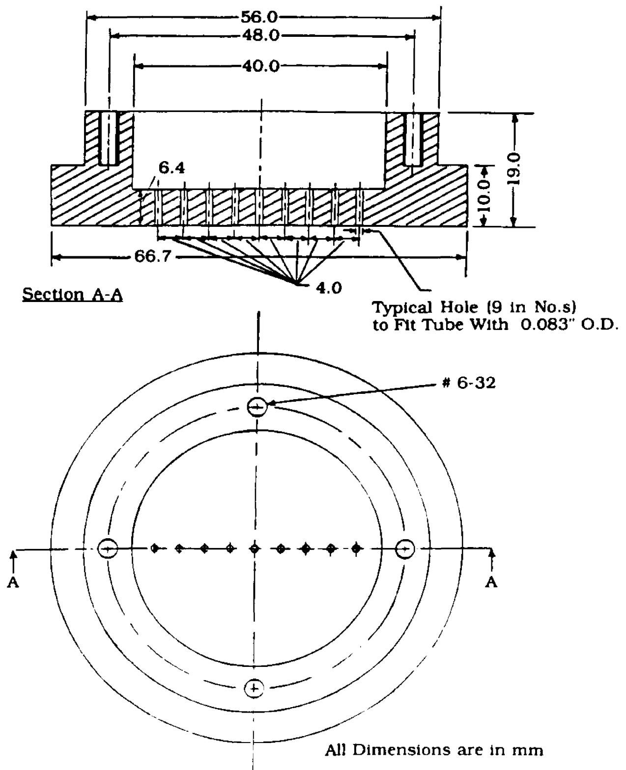
Fig. 3.4 Instrumentation Disk for Surface Pressure Taps- Disk No. 2
