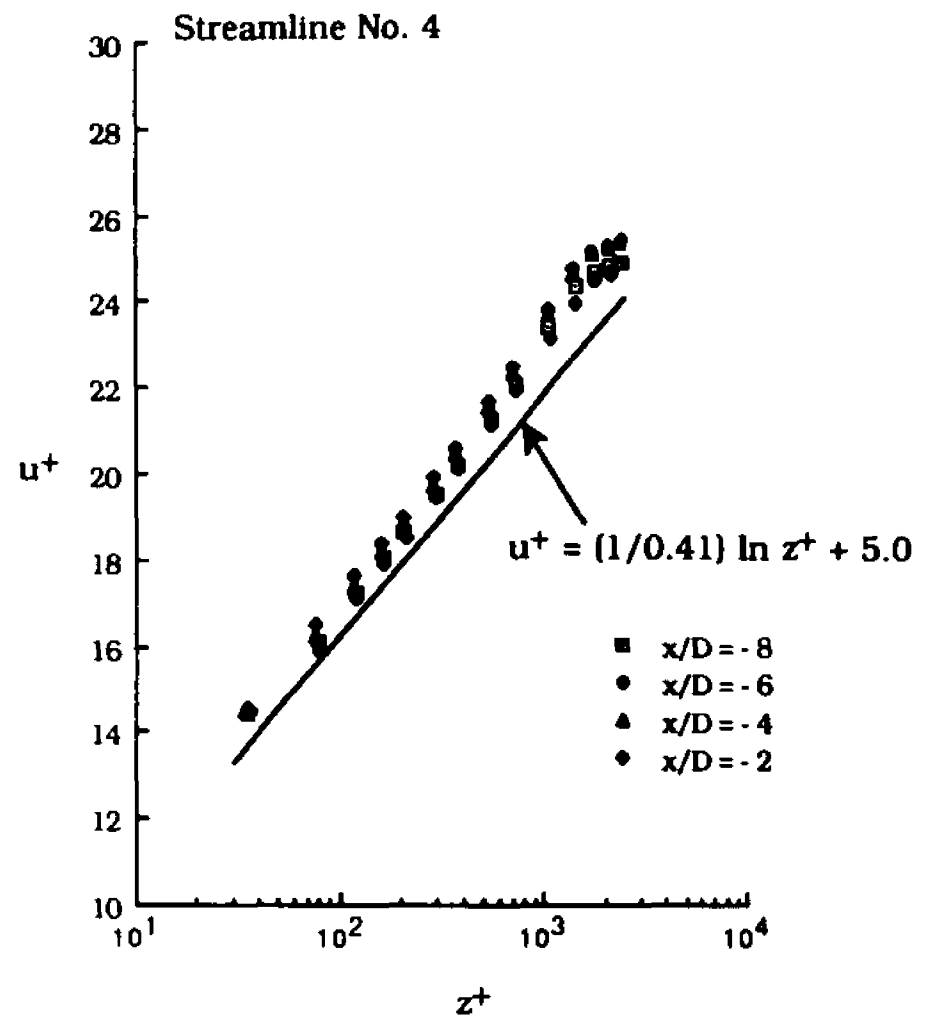
(b) In Inner-Layer Variables
