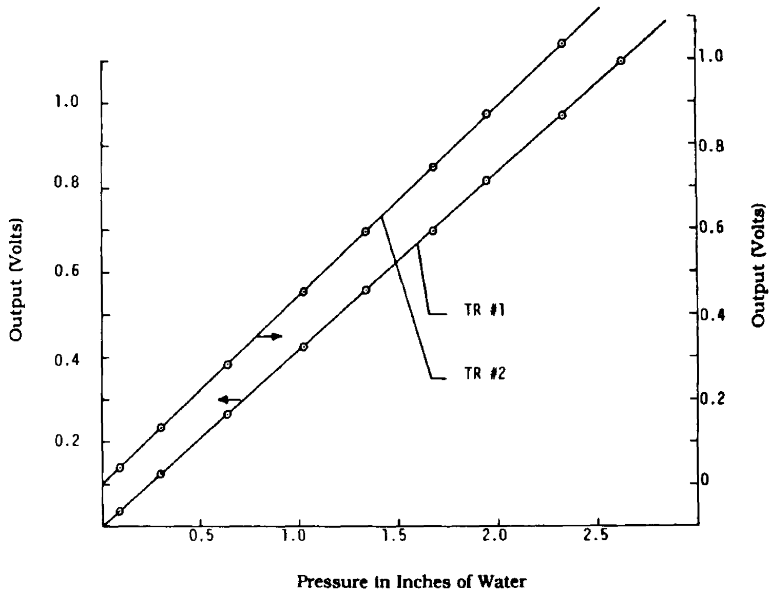
Fig. 3.10 A Typical Calibration of Variable Reluctance Type Differential Pressure Transducers
