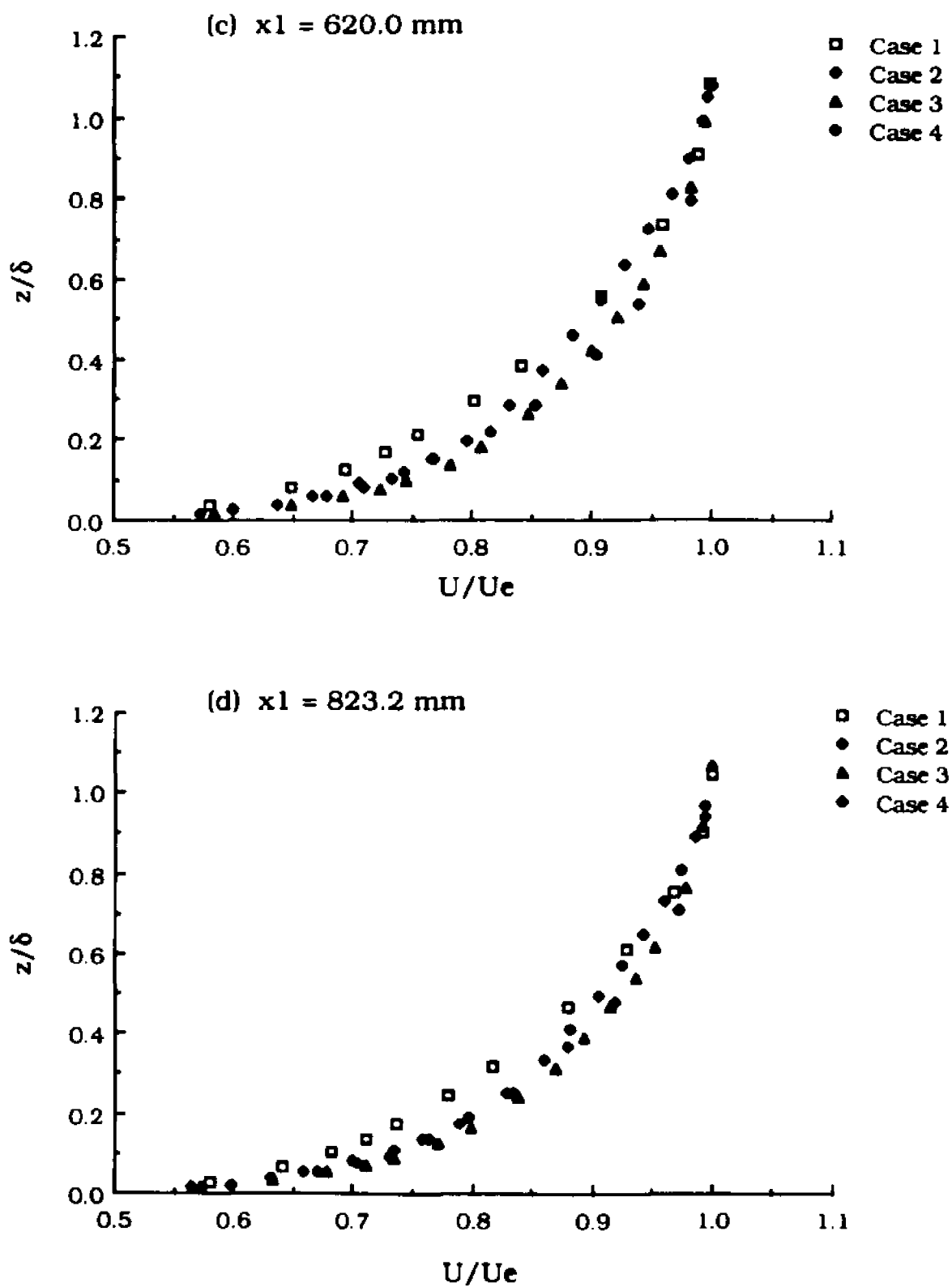
Fig. 4.8 (Contd.) Comparison of Non-Dimensional Mean Velocity Profiles
