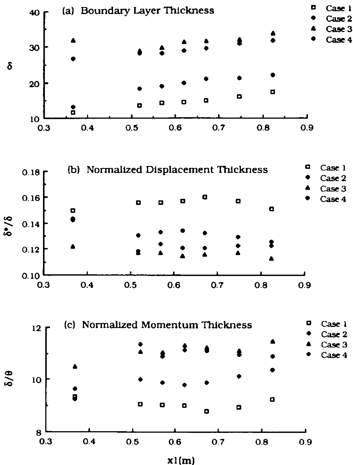
Fig. 4.3 Variation of Boundary Layer Parameters as a Function of Streamwise Distance
