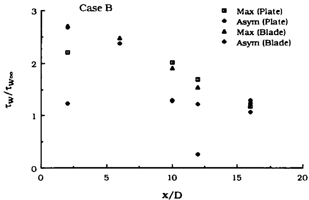
Fig. 5.30 Variation of Maximum and Asymptotic Values of Wall Shear Stress for Case B
