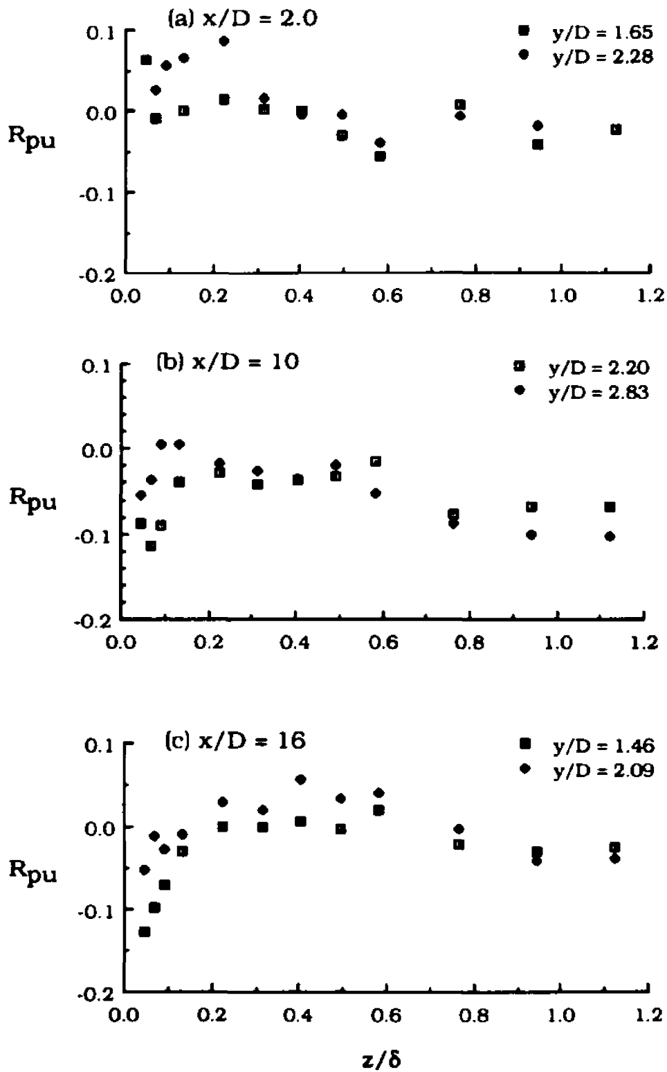
Fig. 6.7 Variation of Wall Pressure-Velocity Correlation Coefficient at Different Streamwise Locations in Blade End-Wall Corner Region
