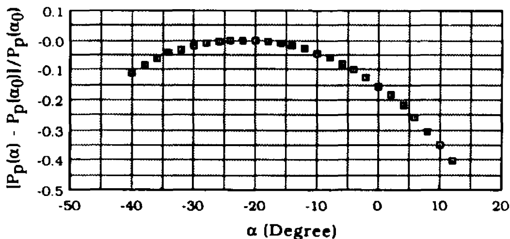
(b) Error in Preston Tube Pressure Due to its Misalignment With the Local Flow Direction- A Typical Error Distribution in Three-Dimensional Flow (Note: \alpha = 0 Implies that the Centerlines of the Preston Tube and the Flat Plate are Parallel)
