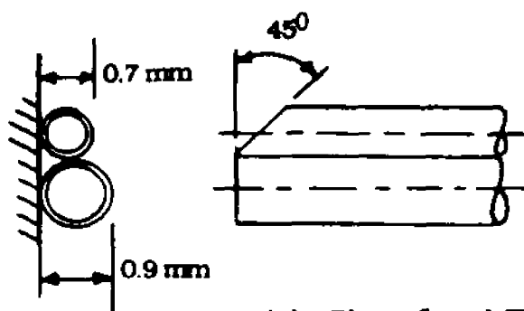
(a) Chamfered Type
