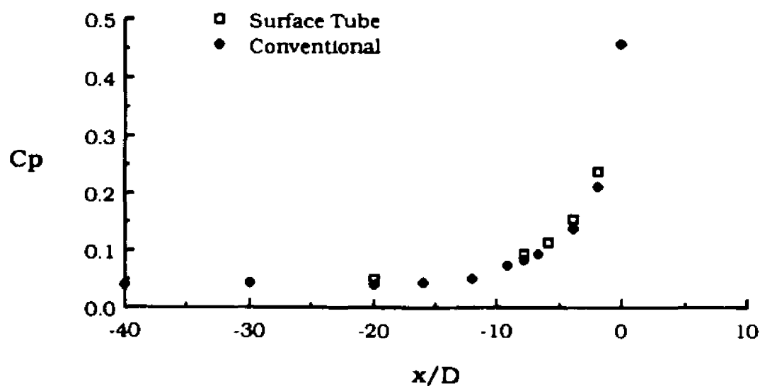
Fig. 5.4 Surface Static Pressure Variation on Stagnation Streamline- A Comparison Between Surface Static Tube and Conventional Techniques
