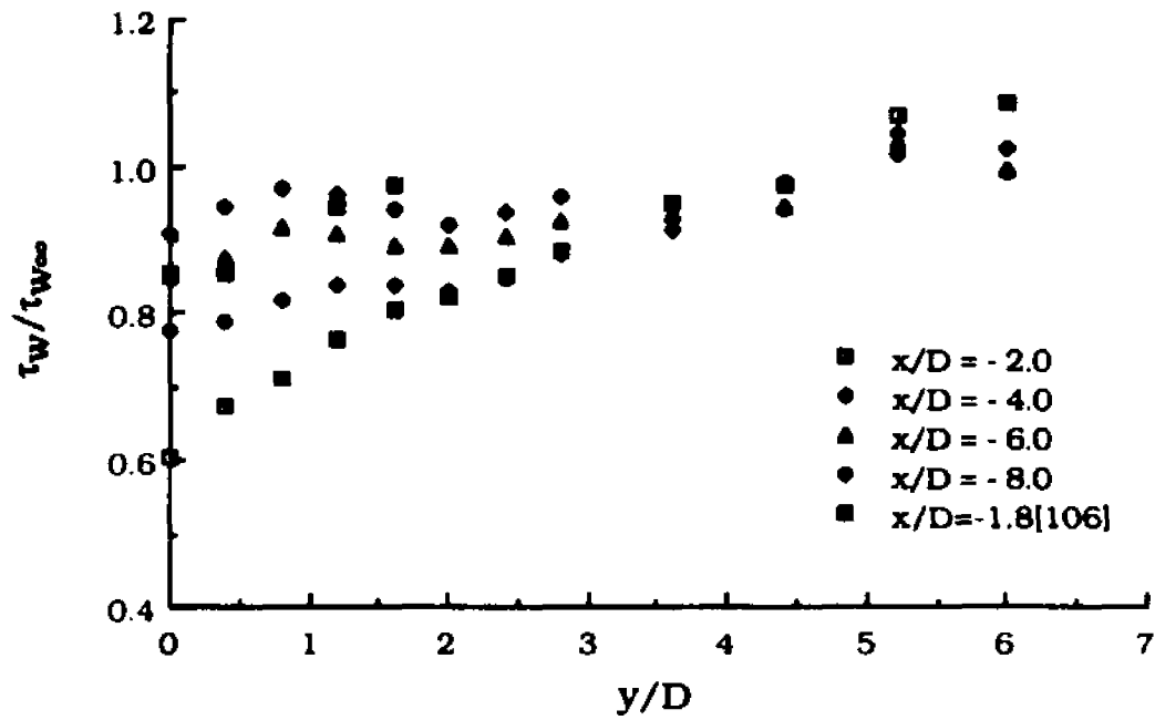
Fig. 5.5 Wall Shear Stress Variation Upstream of the Blade Leading Edge
