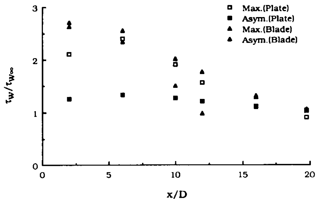
Fig. 5.24 Variation of Maximum and Asymptotic Values of Wall Shear Stress in Blade End-Wall Corner Region for Case A
