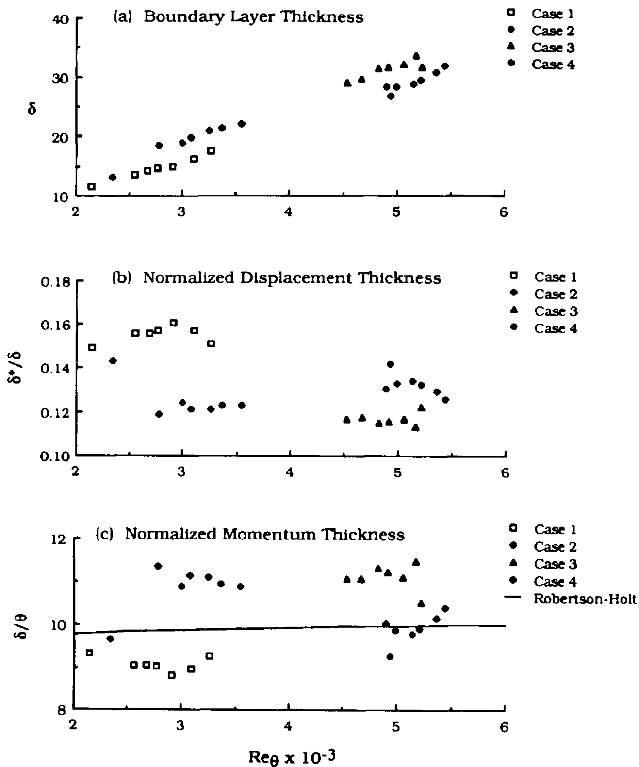
Fig. 4.5 Variation of Boundary Layer Parameters With Re_\theta
