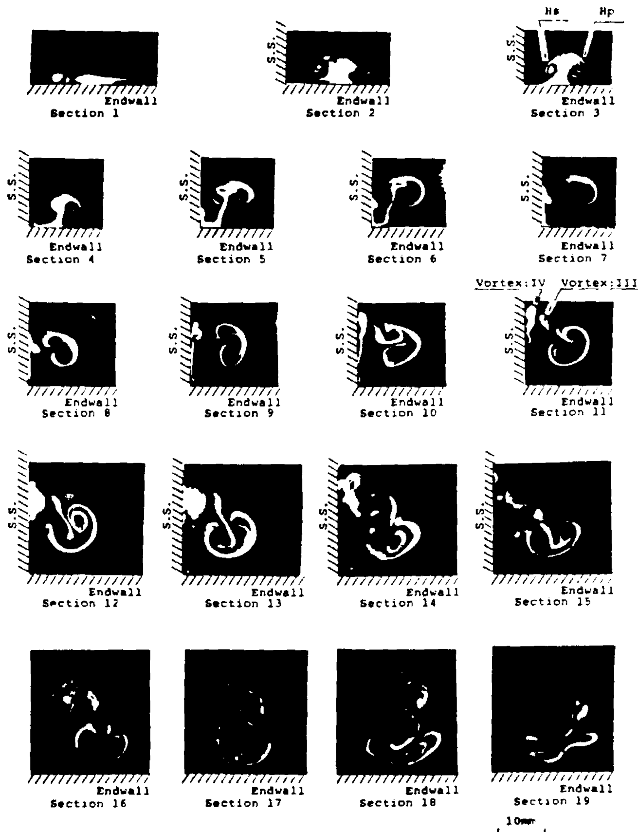
Fig. 2.2 Development of Streamwise Vortices in a Turbine Cascade Passage, Fig.10 of Reference 12(Reprinted by Permission of the Publisher)
