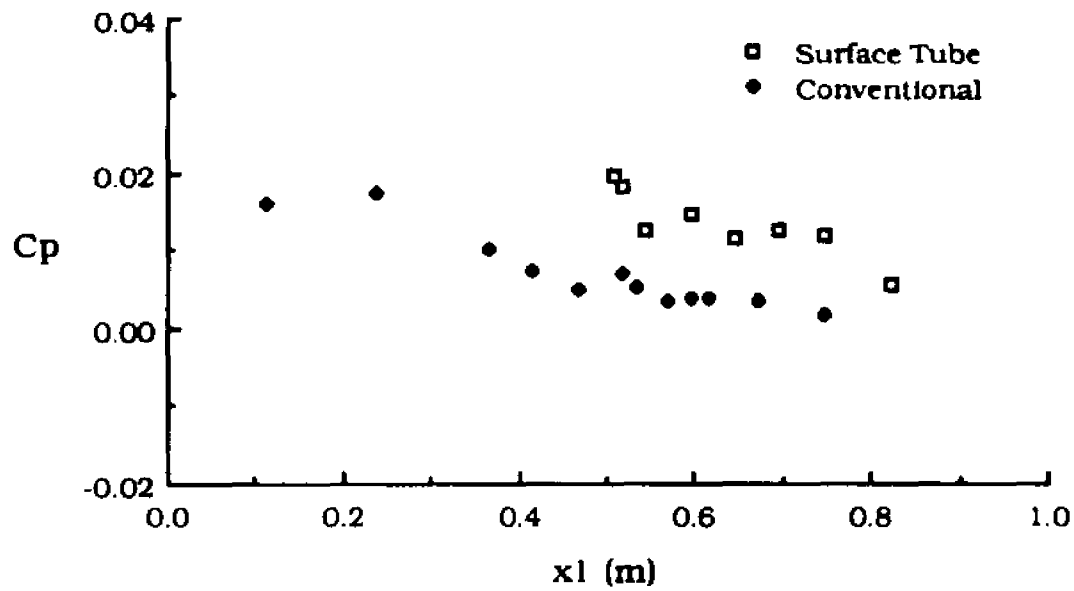
Fig. 5.1 Surface Static Pressure Variation Along Flat Plate Centerline (Two-Dimensional Flow)
