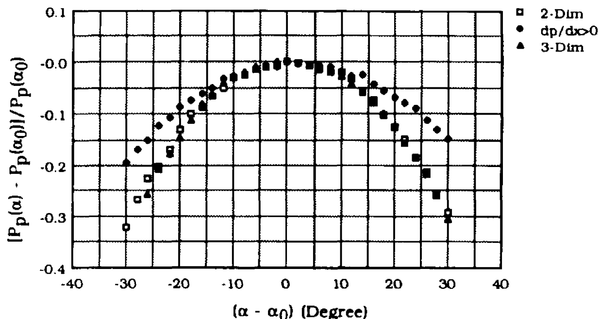
(a) Yaw Sensitivity of Preston Tube in Different Flow Conditions
