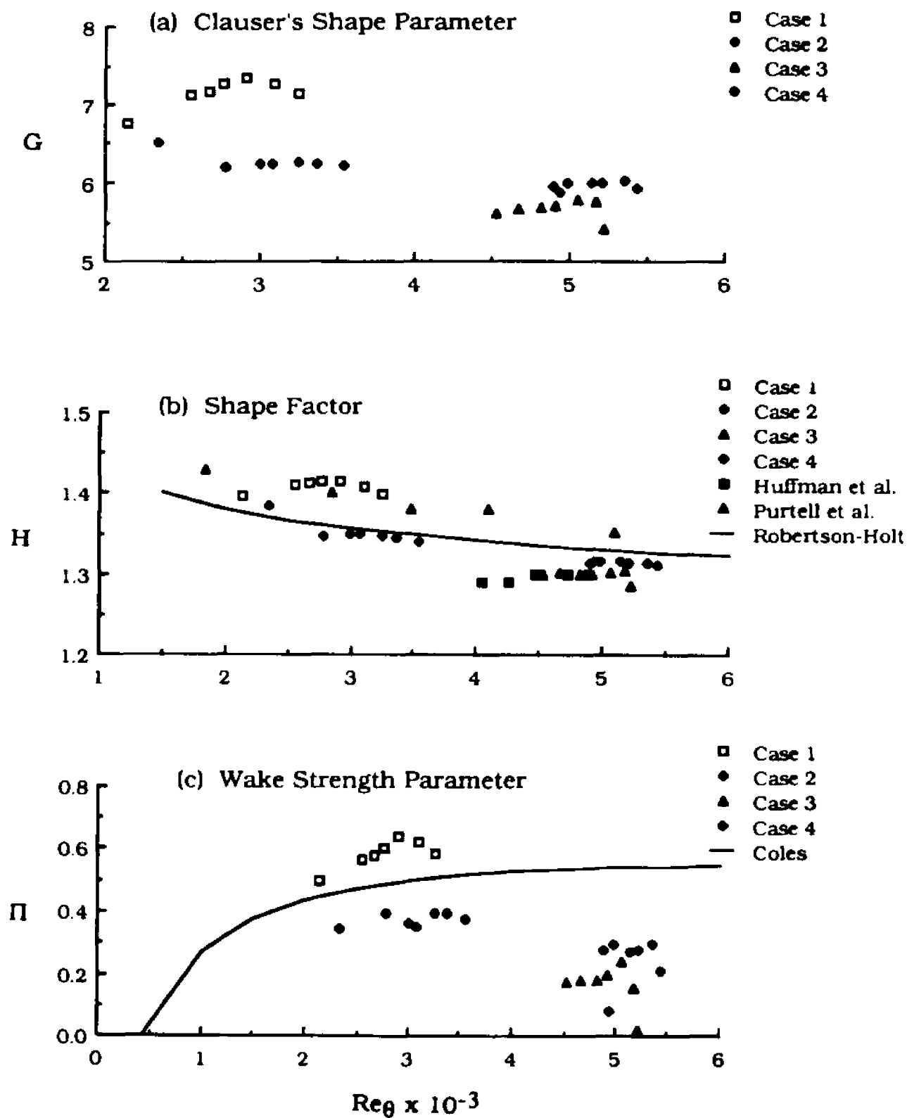
Fig. 4.6 Variation of Boundary Layer Parameters With Re_\theta
