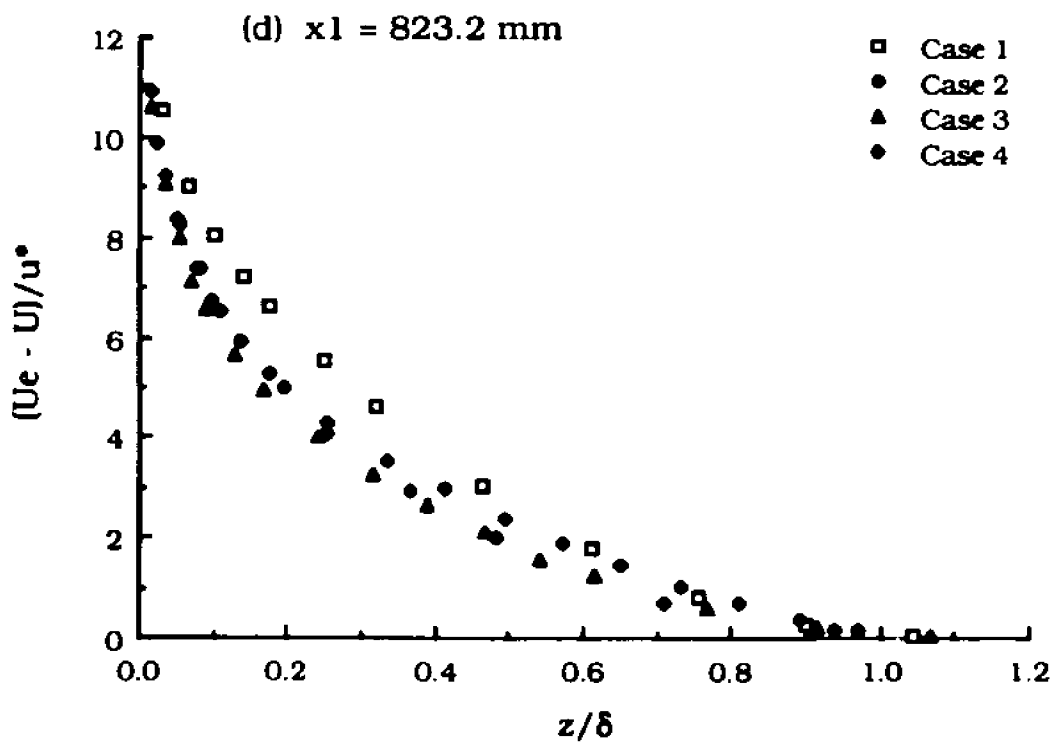
Fig. 4.9 (Contd.) Comparison of Mean Velocity Profiles on Velocity-Defect Plot
