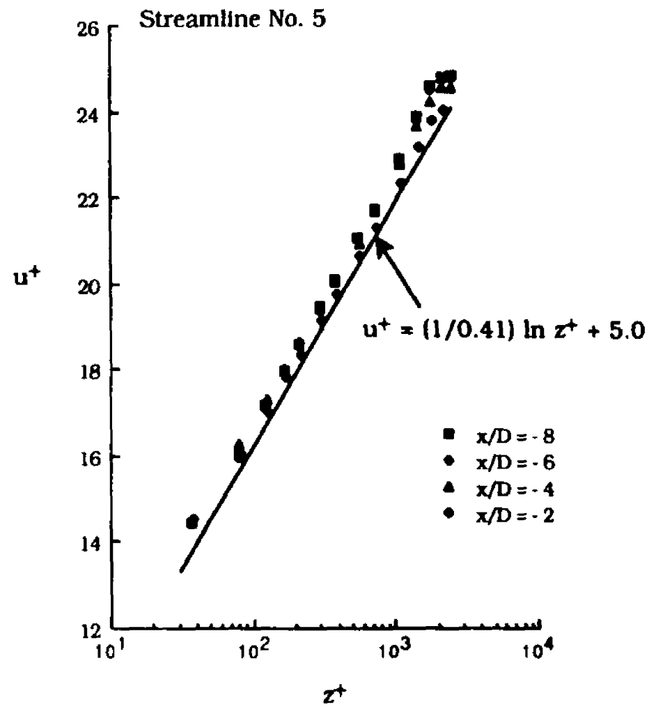
(b) In Inner-Layer Variables
