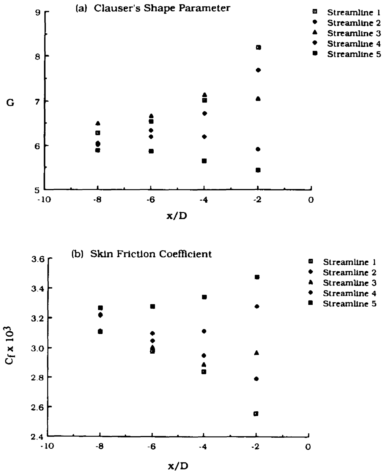
Fig. 5.15 Variation of Clauser's Shape Parameter and Skin Friction Coefficient in Upstream Region of the Blade Leading Edge
