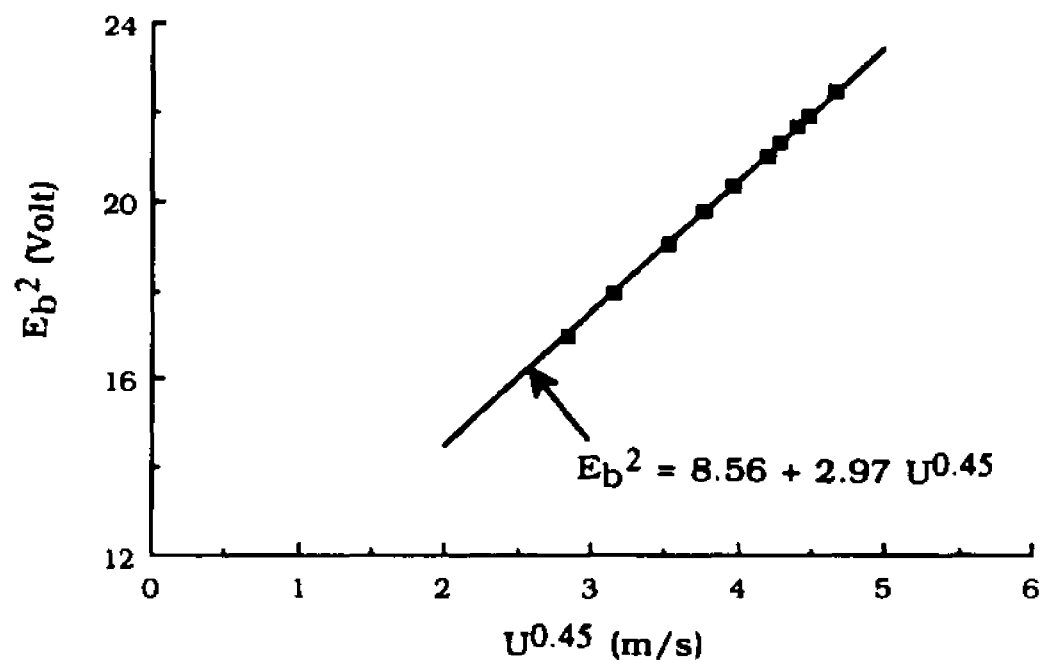
Fig. A.1 A Typical Calibration of Normal Single Sensor Hot-Wire Probe
