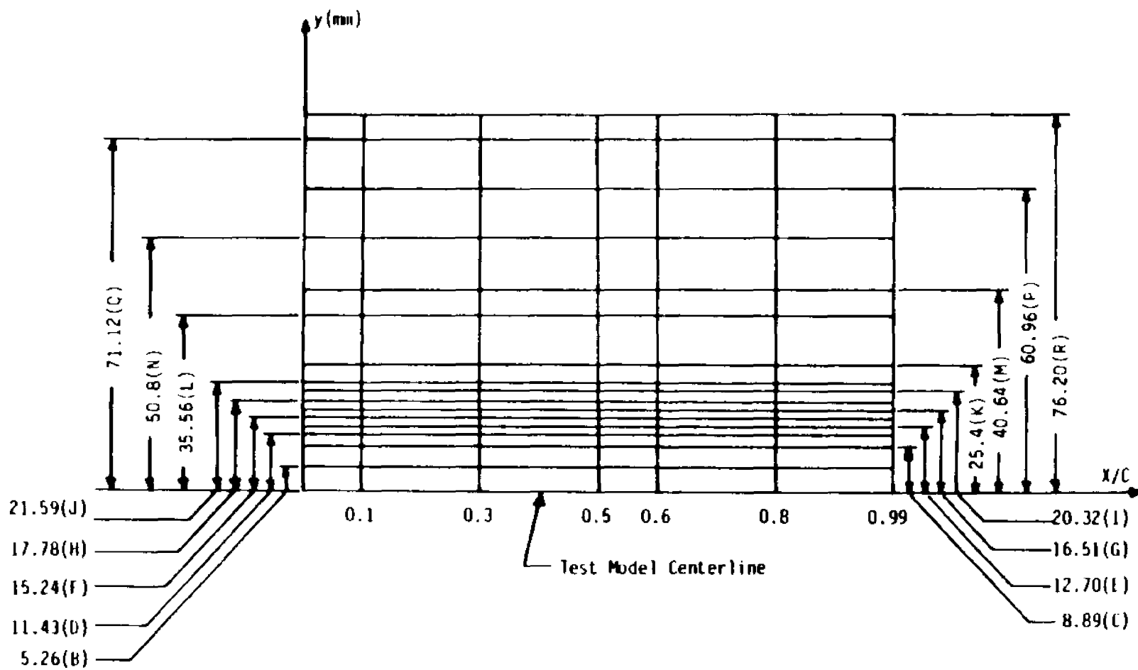
Fig. 3.16 Locations of Measurement on the Flat Plate Surface of the Test-Model in Corner Region
