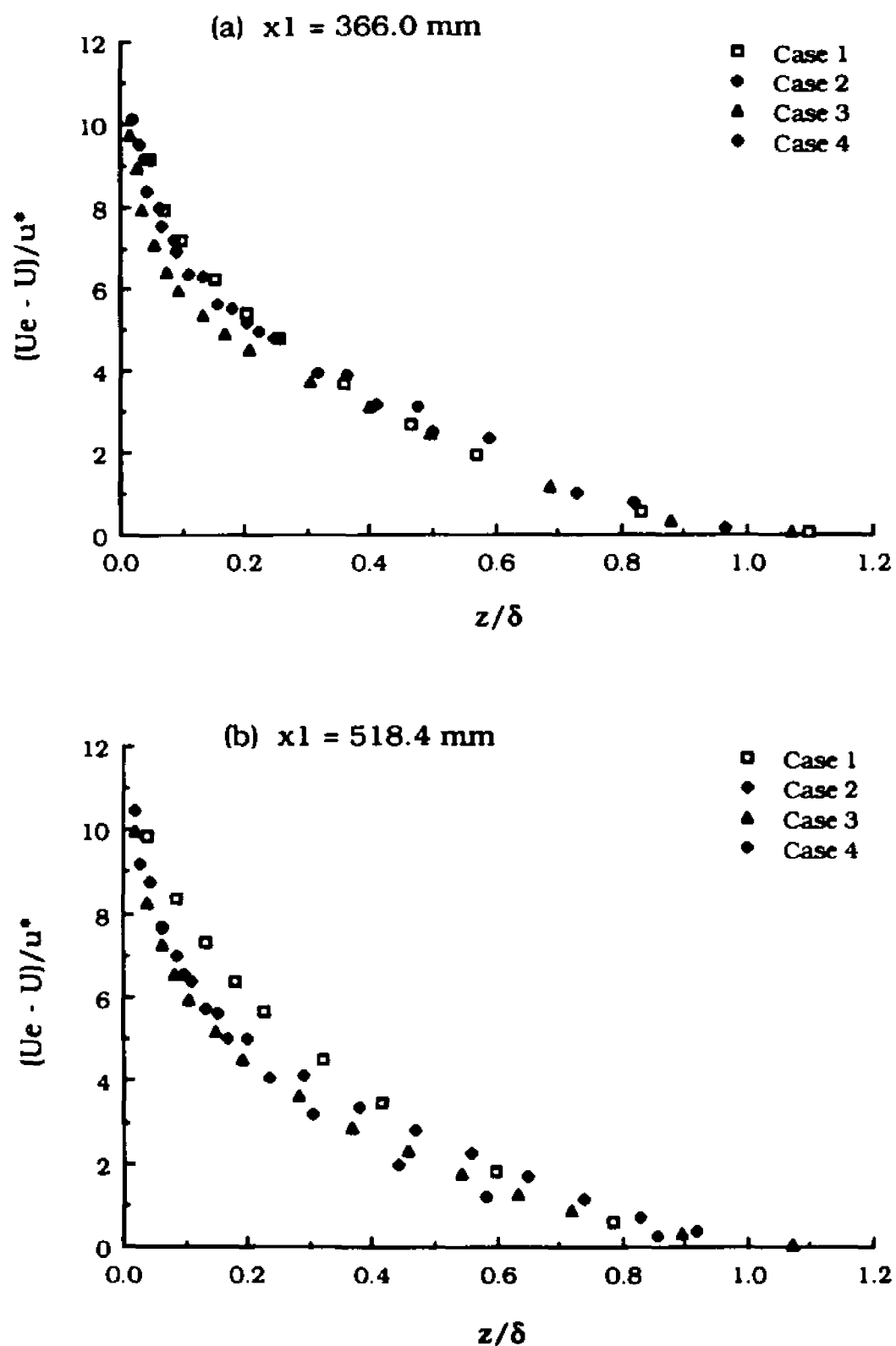
Fig. 4.9 Comparison of Mean Velocity Profiles on Velocity-Defect Plot
