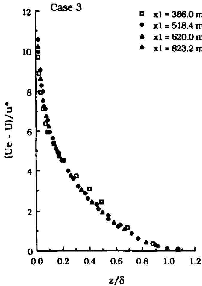
(a) Velocity-Defect Plot
