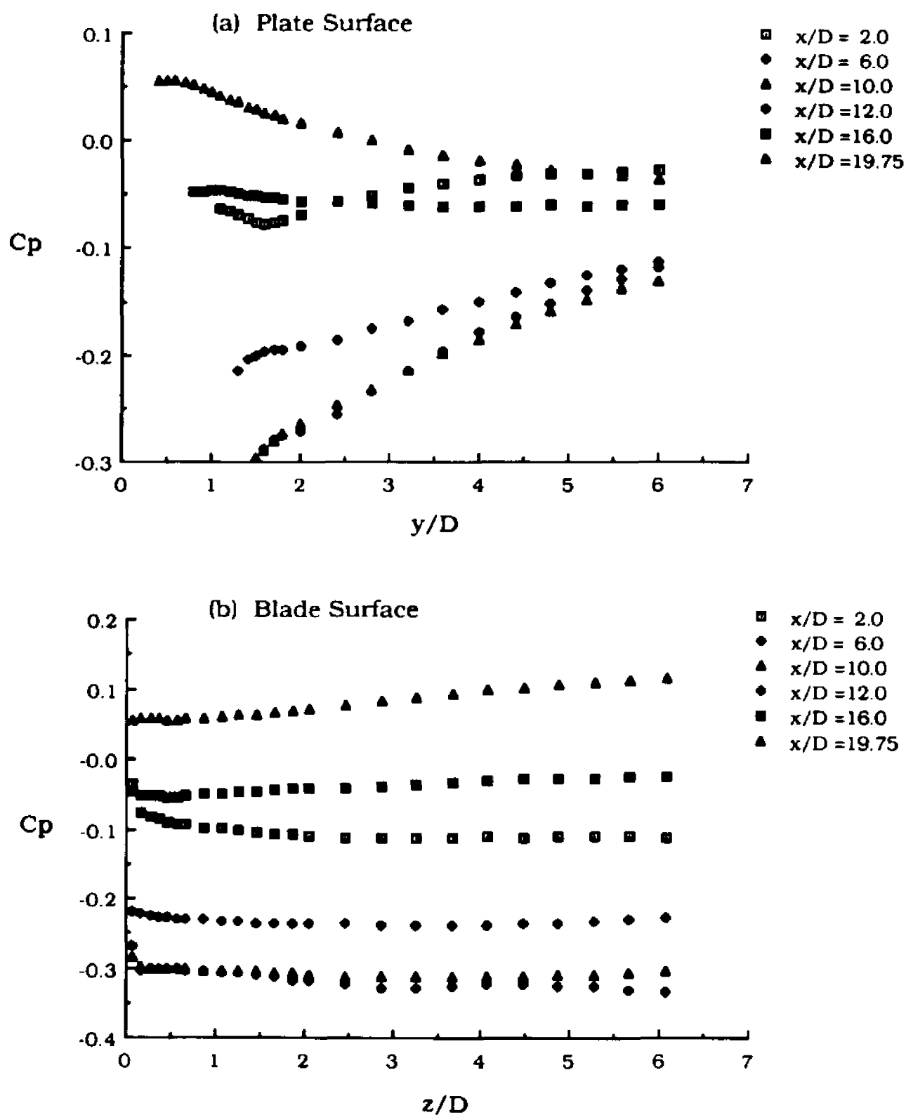
Fig. 5.20 Surface Static Pressure Distribution in Blade End-Wall Corner Region for Case A
