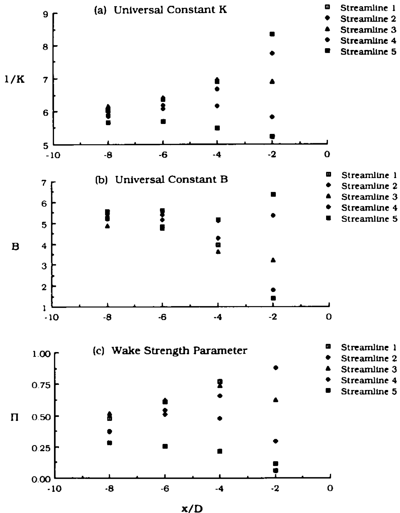
Fig. 5.13 Variation of 1/K , B , and \Pi in Combined Law of the Wall and the Wake in Upstream Region of the Blade Leading Edge
