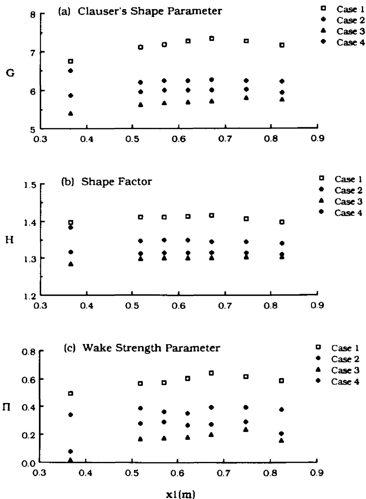
Fig. 4.4 Variation of Boundary Layer Parameters as a Function of Streamwise Distance
