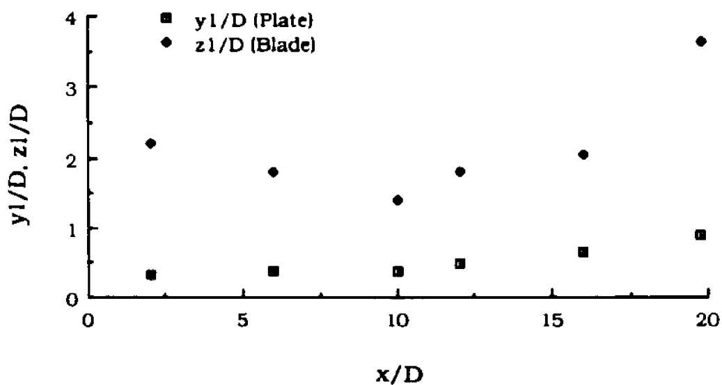
Fig. 5.25 Variation of the Location of Maximum Wall Shear Stress in Blade End-Wall Corner Region for Case A
