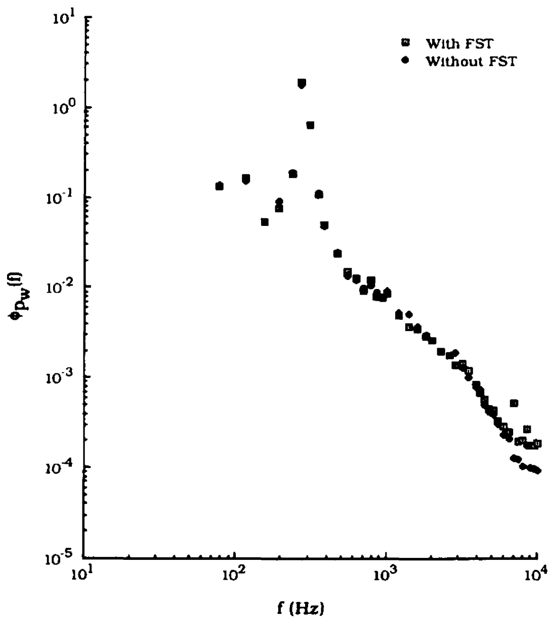
Fig. 6.1 Frequency Spectral Distribution of Wall Pressure Fluctuation (Two-Dimensional Flow)
