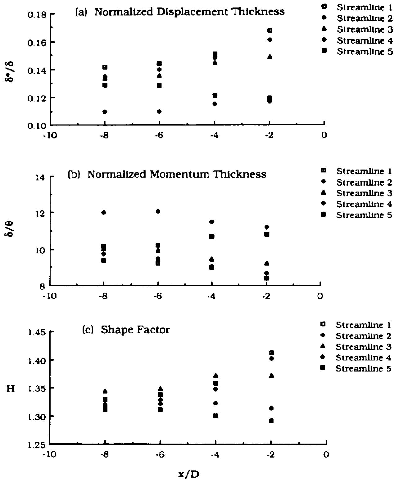
Fig. 5.14 Variation of Boundary Layer Integral Parameters Upstream of the Blade Leading Edge
