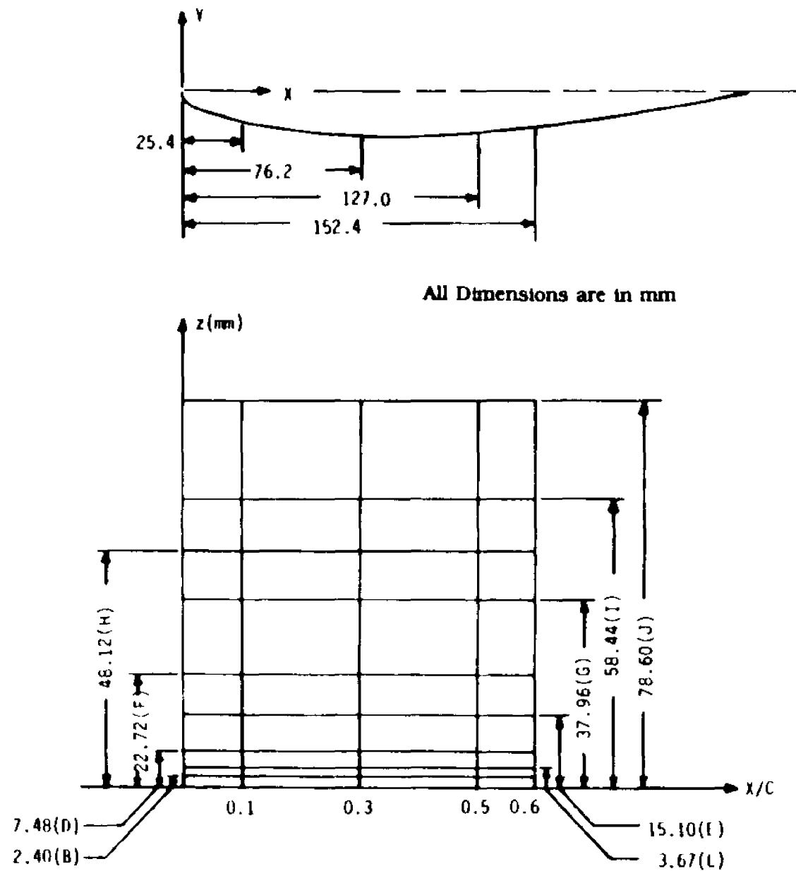
Fig. 3.17(a) Locations of Measurement on the Blade Surface of the Test-Model in Corner Region
