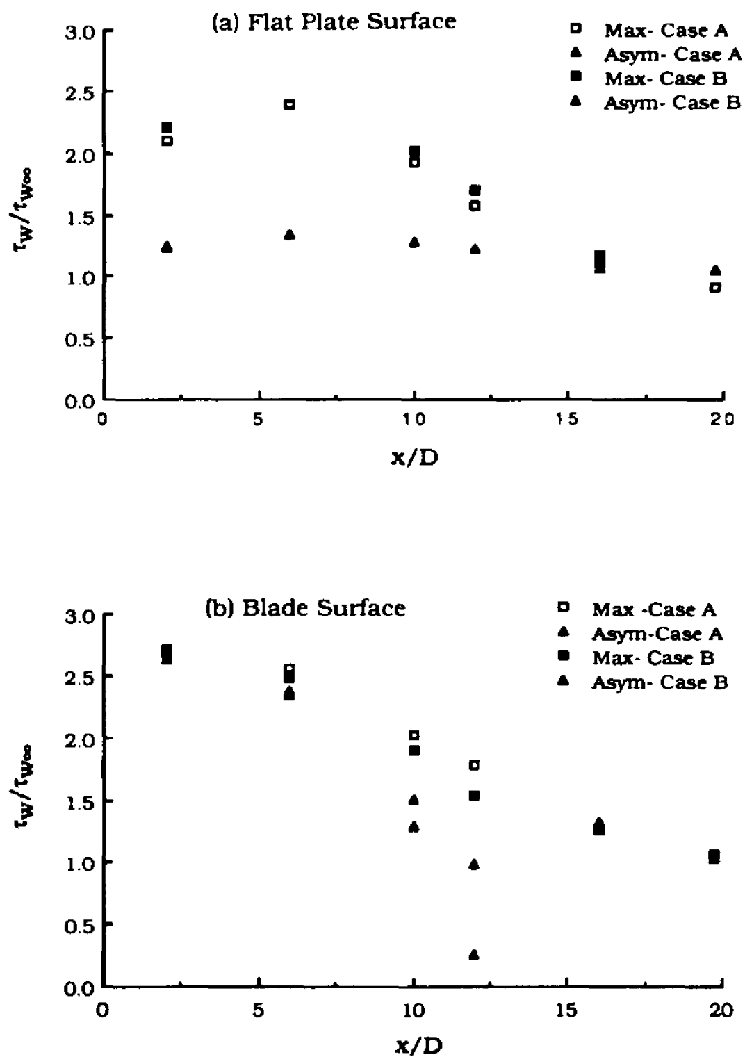
Fig. 5.38 Variation of Maximum and Asymptotic Values of Wall Shear Stress- A Comparison Between Case A and Case B
