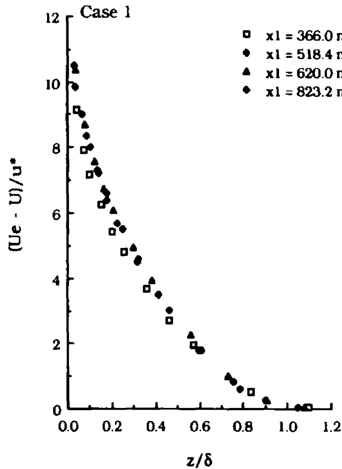
(a) Velocity-Defect Plot
