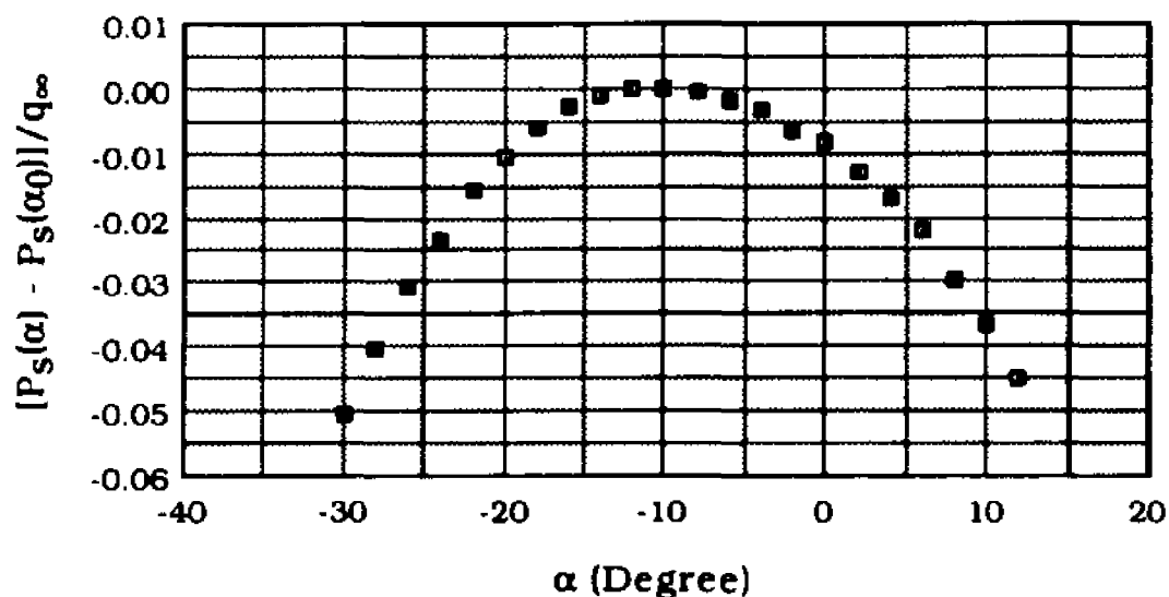
(a) Error in Surface Static Pressure as a Fraction of Free Stream Dynamic Pressure
