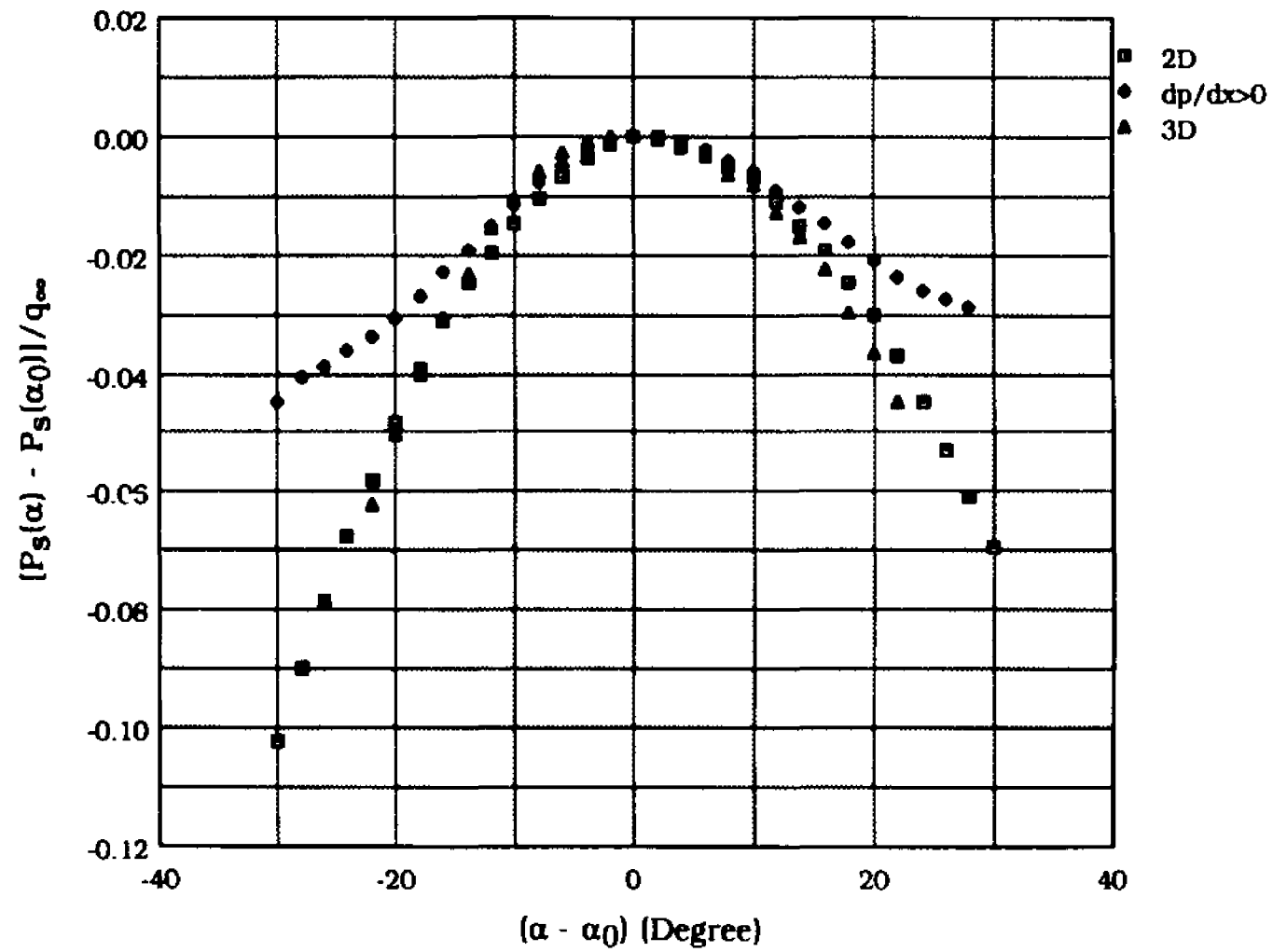
Fig. C.1 Yaw Sensitivity of Static Tube Resting on the Surface in Different Flow Conditions
