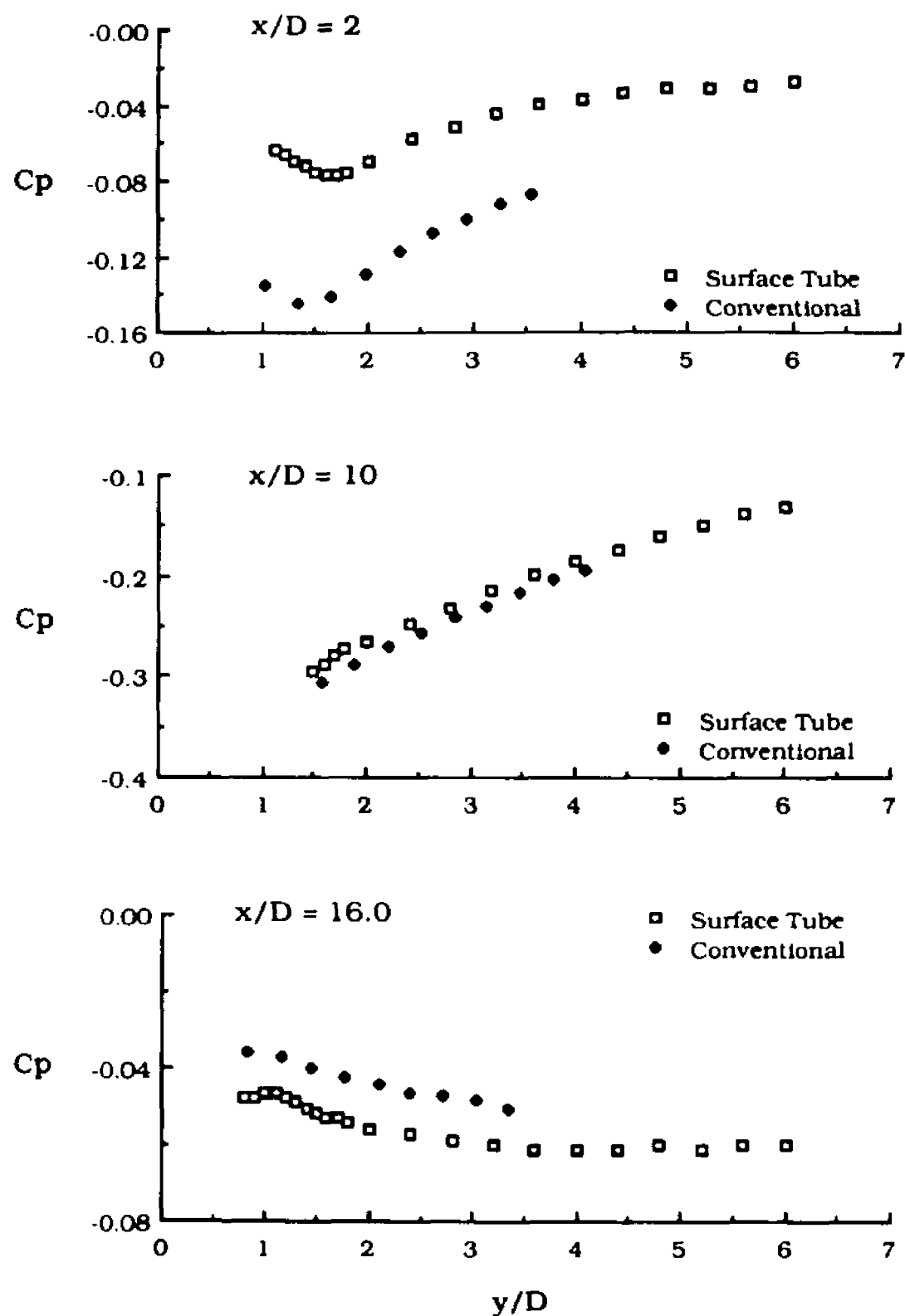
Fig. 5.22 Surface Static Pressure Variation in Blade End-Wall Corner Region- A Comparison Between Surface Static Tube and Conventional Methods (Case A)
