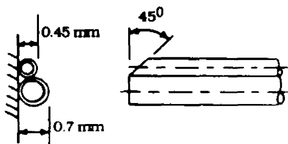
(b) Chamfered Type
