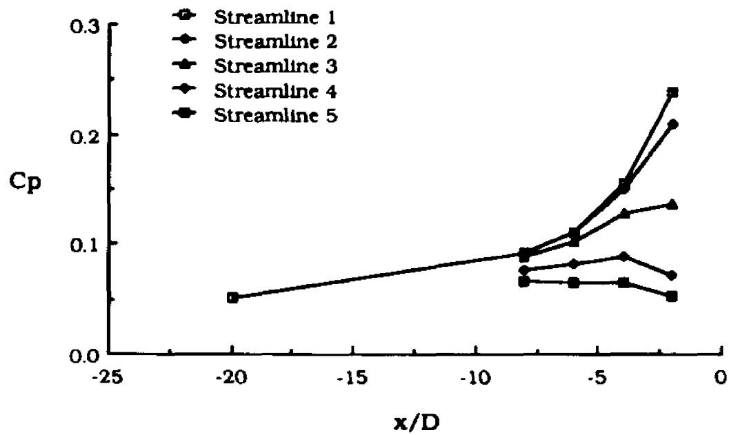
Fig. 5.6 Variation of Surface Static Pressure Along Different Streamlines
