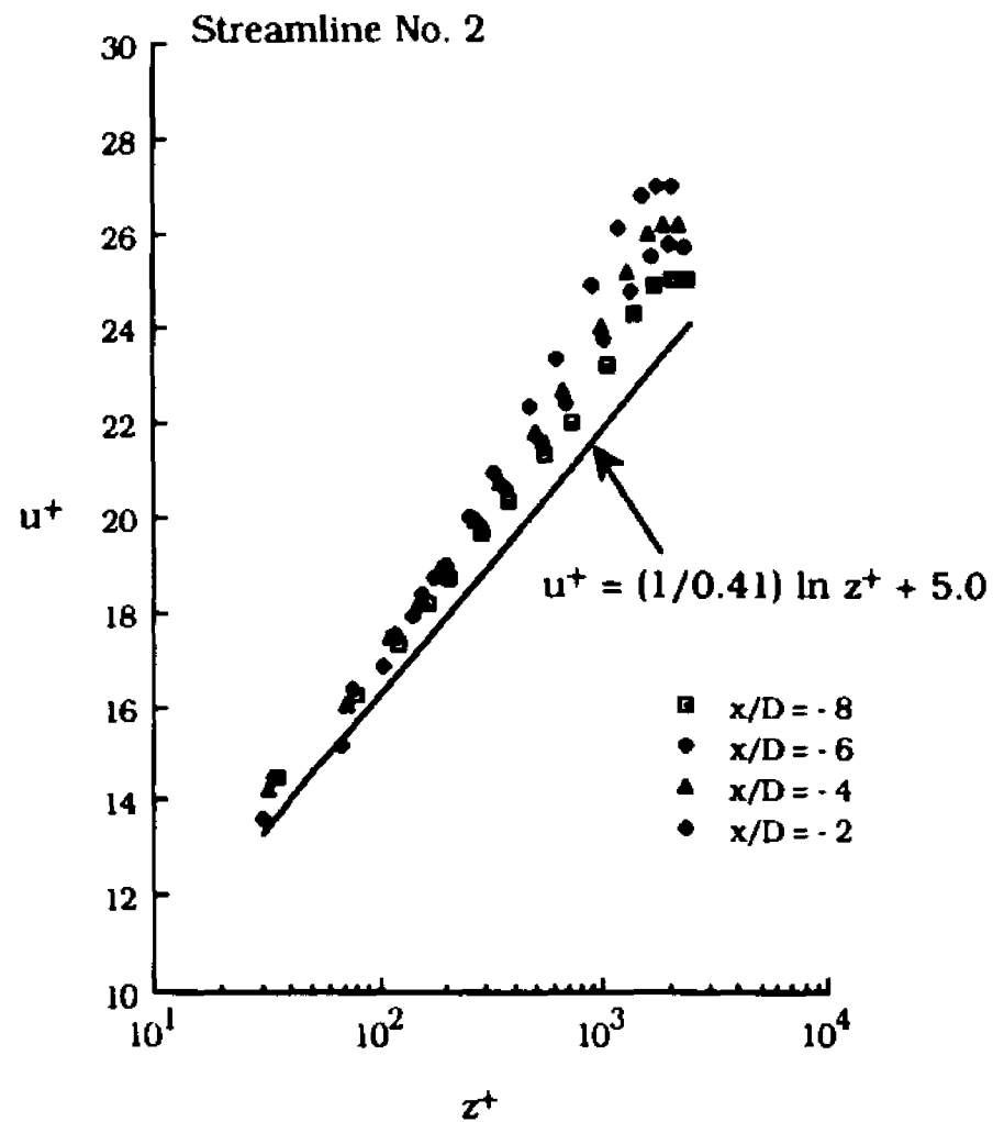
(b) In Inner-Layer Variables
