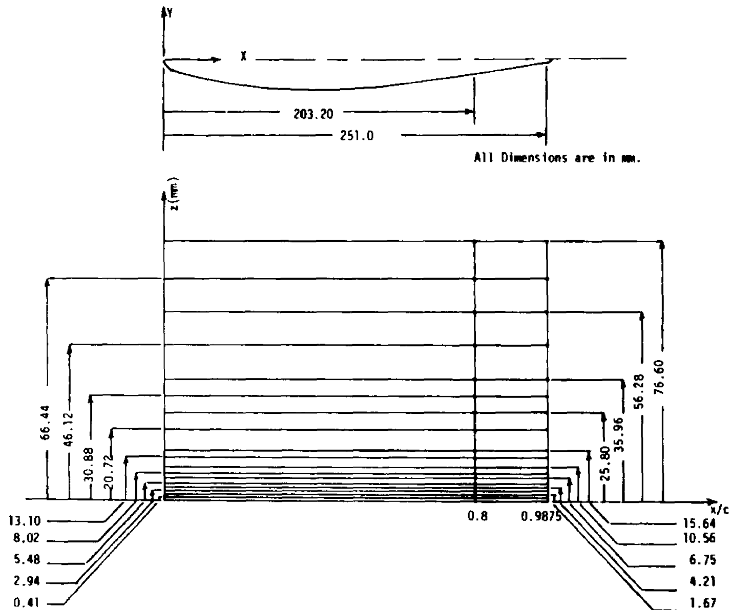
Fig. 3.17(b) Locations of Measurement on the Blade Surface of the Test-Model in Corner Region
