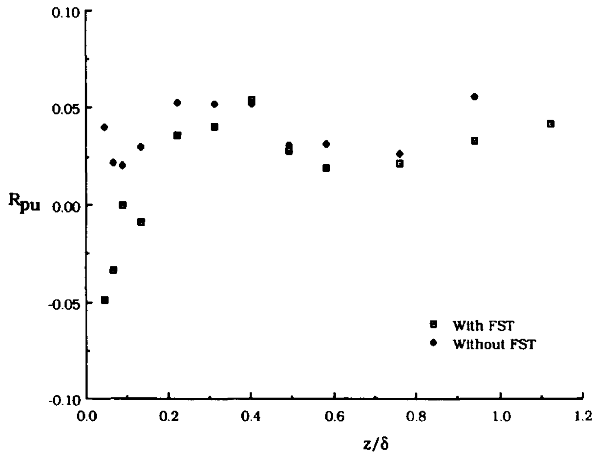
Fig. 6.2 Wall Pressure-Velocity Correlation Coefficient (Two-Dimensional Flow)
