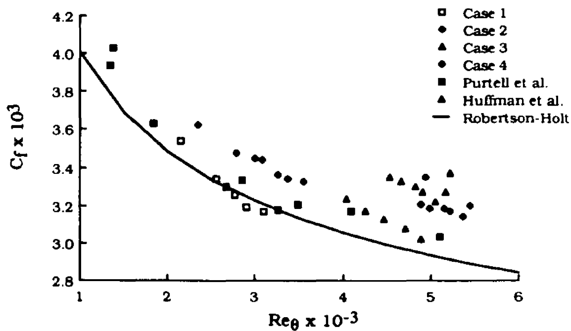
(b) Variation of C_f With Re_\theta
