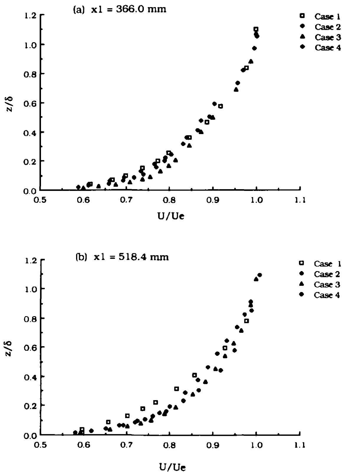
Fig. 4.8 Comparison of Non-Dimensional Mean Velocity Profiles
