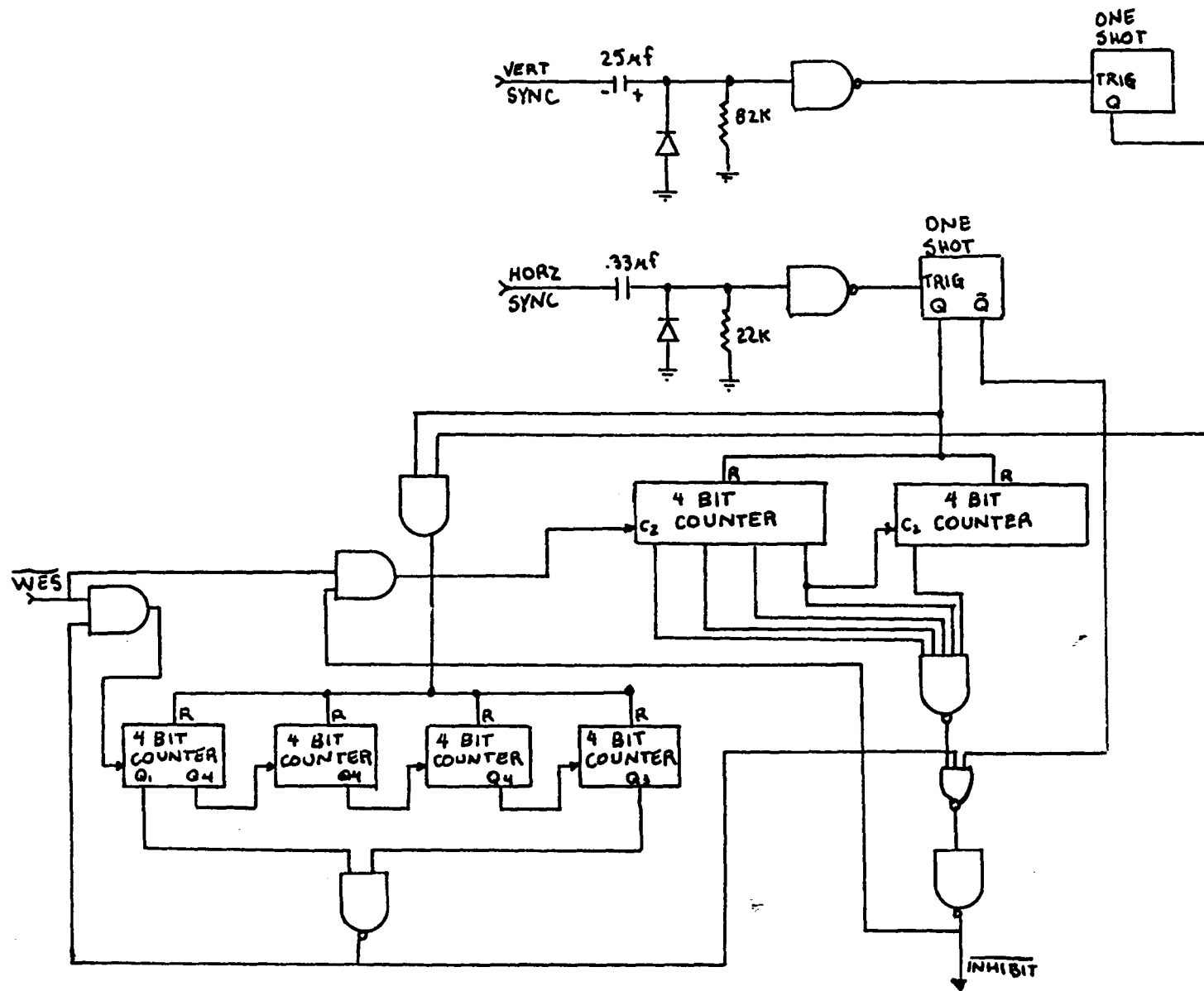
FIG 47 SYNC. GENERATOR
