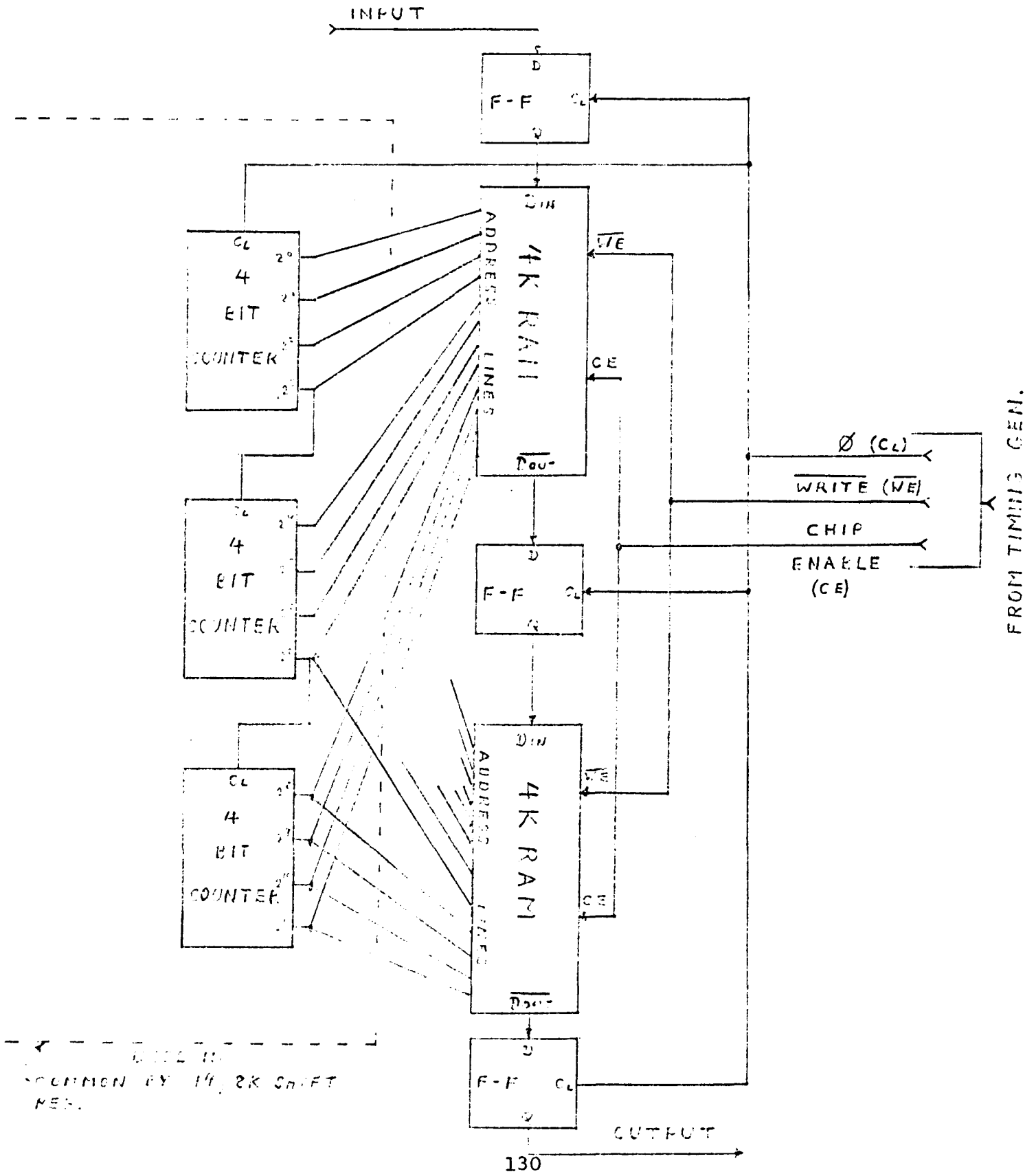
Fig. 4 One 8K Shift Register Made From 8K of Random Access Memory
