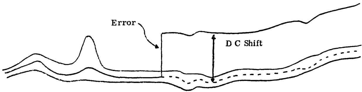
Part A. The Video Signal From 3 Consecutive Scanning Lines
