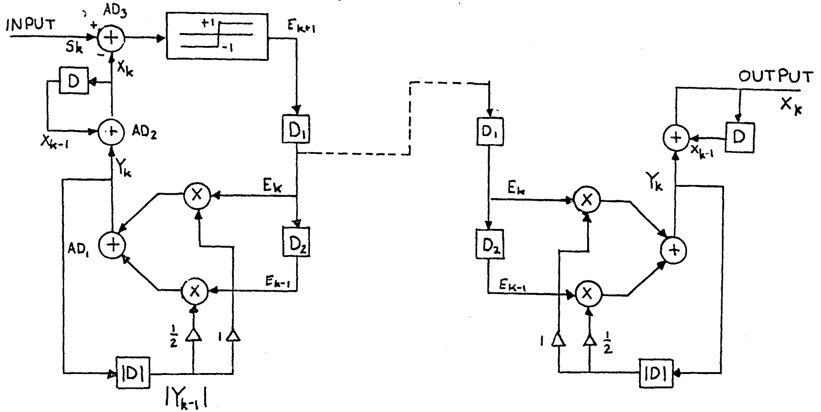
FIG 10 DIGITAL ADAPTIVE DELTA MODULATOR
