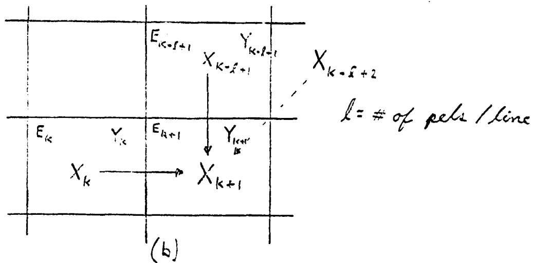
FIG 51 TWO DIMENSIONAL $\Delta$ MOD
