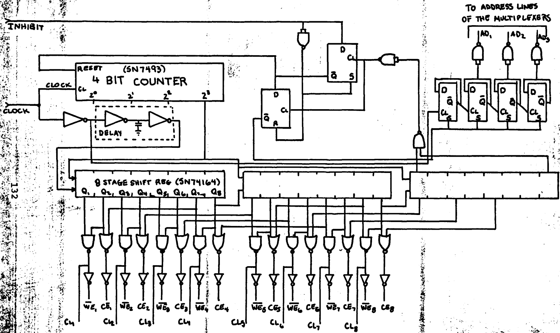
FIG 46 8STAGE CLOCK AND TIMING GENERATOR
