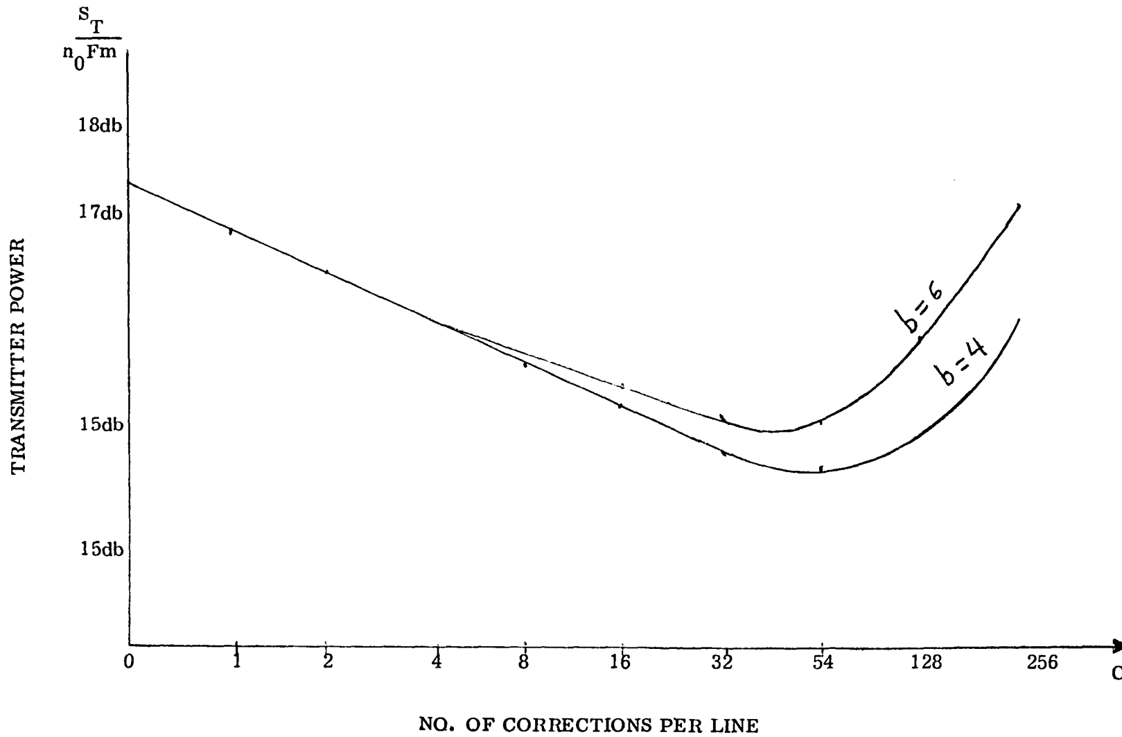
Fig. 28 The number of corrections per line vs. the transmitted power required to maintain a picture signal to distortion ratio of +30db due to channel errors
