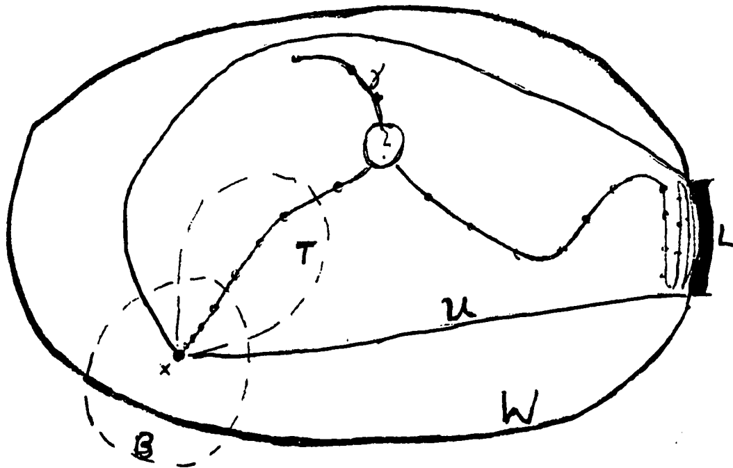
Figure 3.5: The Snake Argument
