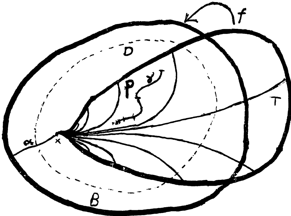
Figure 3.3: Fixed points in a tract
