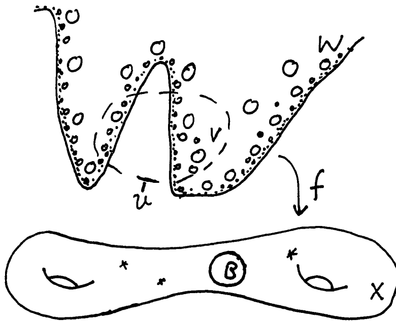
Figure 3.2: Proper preimages near \partial(f)
