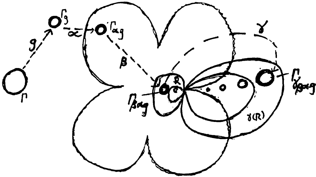
Figure 4.3: Wandering annuli II
