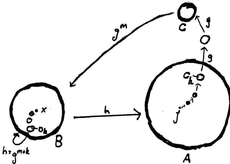
Figure 3.4: Creating more fixed points
