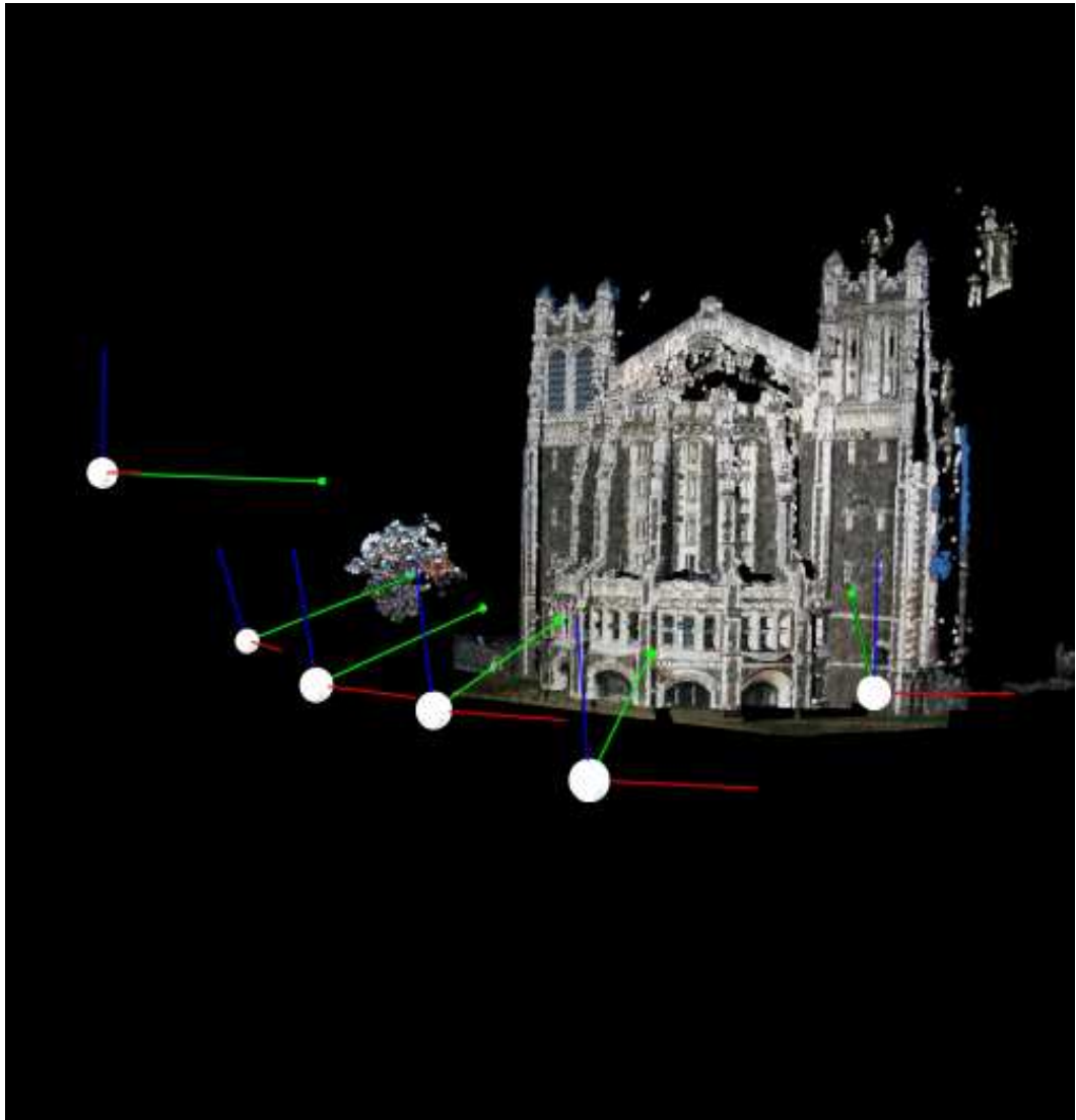
Figure 3.9: Camera configurations (6 cameras) with respect to texture-mapped 3D model of building 3 (Shepard Hall at CCNY, NYC).
