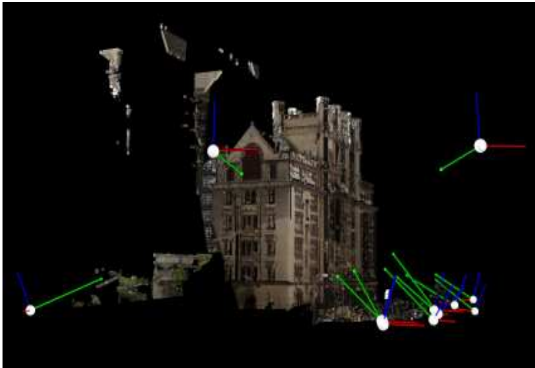
Figure 3.7: Camera configurations (11 cameras) with respect to texture-mapped 3D model of building 1 (Thomas Hunter building at Hunter College of CUNY).
