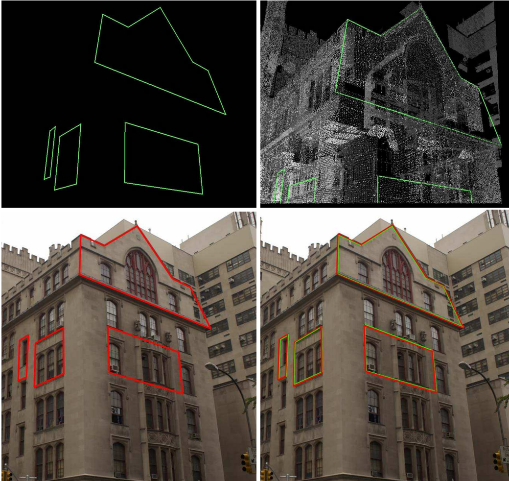
Figure 5.5: The evaluation of the registration result on building 1. For this case, 19 pairs of 3D and 2D lines are selected and the average error is 1.6833 in pixels (see Sec. 5.4 and Table 5.1 for description of error measurements). Top Left: The manually marked 3D lines; Top Right: Closed view of marked 3D lines with 3D range point cloud; Bottom Left: The manually marked 2D lines; Bottom Right: The marked 3D lines are projected onto the image plane (green) based on the registration result and overlaid with their corresponding 2D lines (red).
