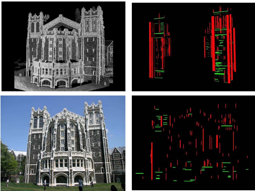
Figure 3.14: A successful image-to-range registration for Building 3. top left : 3D range data of Building 3. top right : extracted 3D rectangular parallelepipeds. bottom left : the 2D image of building 3, two towers are captured in the image. bottom right : extracted 2D rectangles. The abundance of linear structures in these two towers allows the extraction of sufficient 3D and 2D features. With adequate features, the system can register the 2D image with the 3D range data.
