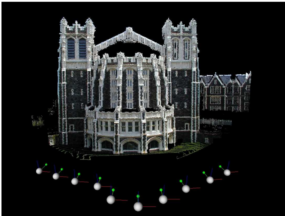
Figure 4.8: Shepard Hall with ten automatically texture mapped images. All ten images are registered with the range data by image-to-range registration (Sec. 4.2) and then the SFM is integrated (Sec. 4.4).
