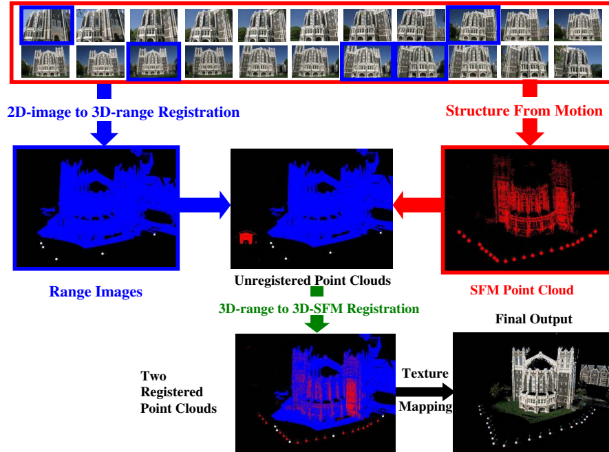
Figure 4.1: On the left branch (highlighted in blue): five color images out of 22 are automatically registered with the dense 3D point cloud M_{range} acquired from the range scanner (Sec. 4.2). The recovered camera positions are shown in white dots. On the right branch (highlighted in red): the set of 22 color images are registered together and a sparse 3D point cloud M_{sfm} is reconstructed from them by using a structure-from-motion (SFM) algorithm (Sec. 4.3). The camera positions (red dots) are shown with respect to the reconstructed 3D point cloud. Then, the sparse 3D point cloud M_{sfm} is registered with the dense 3D point cloud M_{range} (Sec. 4.4). This step brings all the 2D images into alignment with M_{range} . As a result, the whole collection of color images are texture mapped onto the 3D range model M_{range} .
