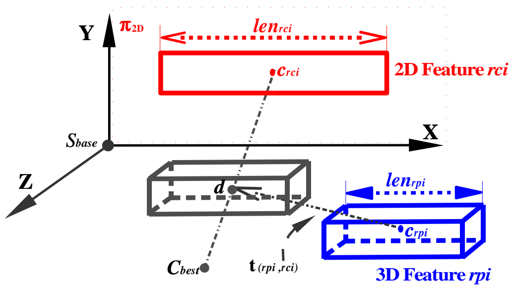
Figure 3.6: Translation computation.
