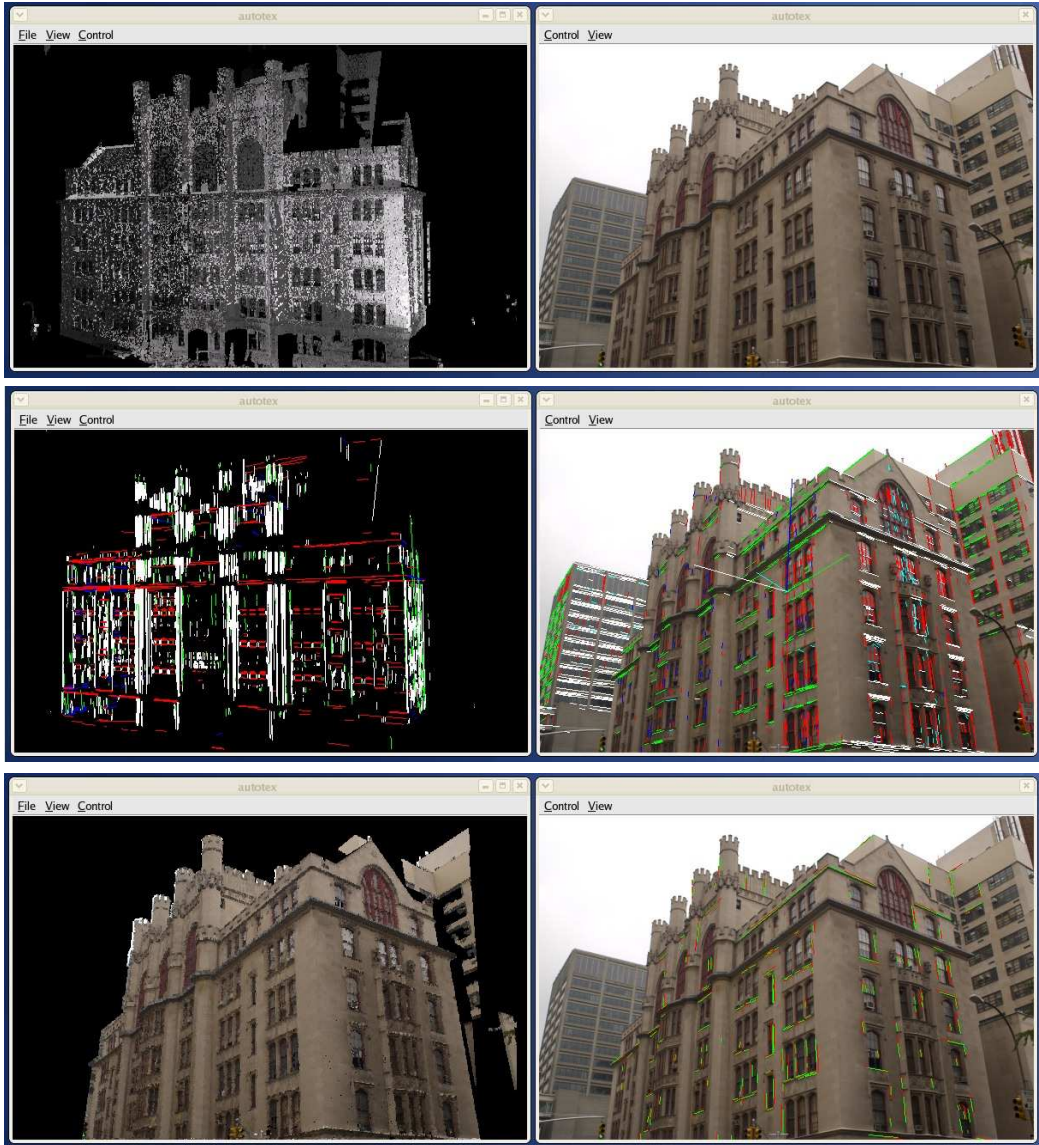
Figure 5.11: Registration result of Building 1. For description see caption of Fig. 5.10
