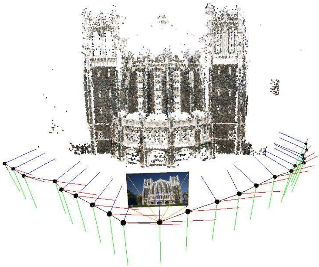
Figure 4.3: The path of camera motion (22 images used) and reconstruction of Shepherd Hall (CCNY) using SFM(see Sec. 4.3). This algorithm was designed and implemented by Wolberg and Zokai [Liu et al. , 2006].
