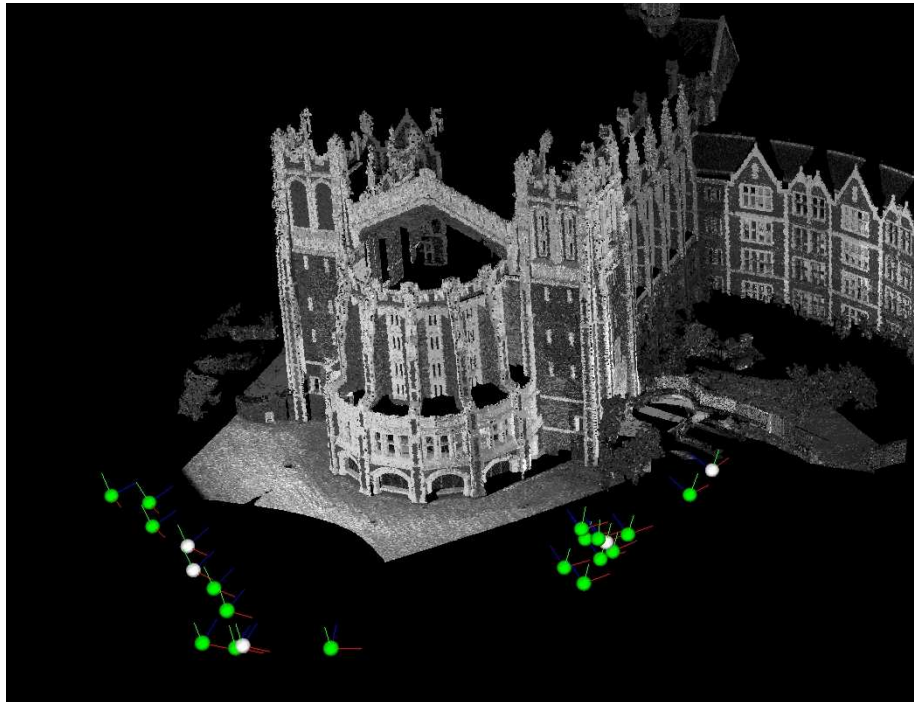
Figure 4.6: We applied our image-to-range registration method (Sec. 4.2) for the registration of all 22 images with the 3D range model. Five of them are successfully registered (white dots). For all other images, the image-to-range registration system fails to produce satisfactory results (green dots). For the reasons of this failure please refer to Sec. 3.6 of Chapter 3. The integration of multiview geometry allows us to successfully register all 22 images with the 3D model (see Figs. 4.2 and 4.7).
