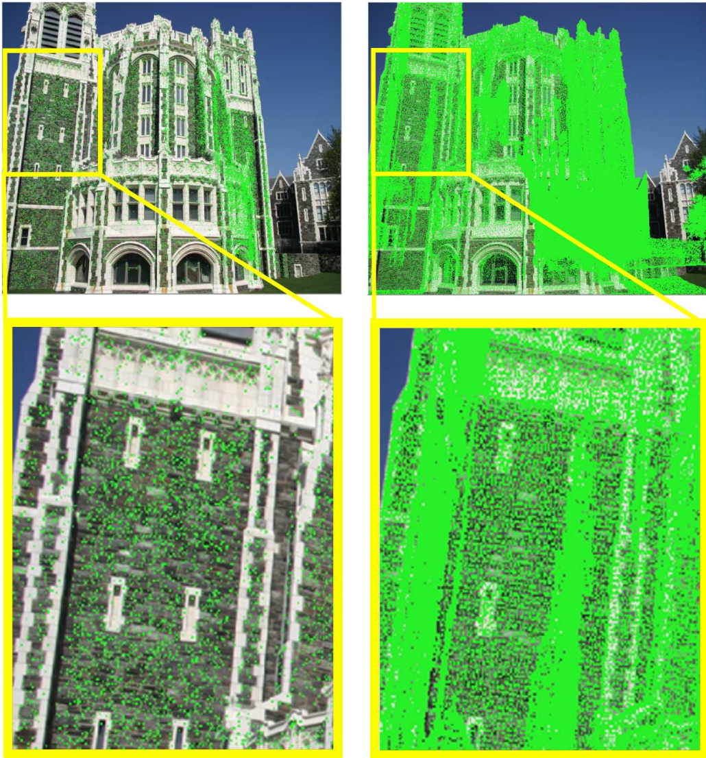
Figure 4.4: (Left) : The points of model M_{sfm} projected onto one 2D image I_n (Sec. 4.3). The projected points are shown in green. (Right) : The points of model M_{range} projected onto the same 2D image I_n (projected points shown in green) after the automatic image-to-range registration (Sec. 4.2). Note that the density of 3D range points is much higher than the density of the SFM points, due to the different nature of the two reconstruction processes. Finding corresponding points between M_{range} and M_{sfm} is possible on the 2D image space of I_n . This yields the transformation between the two models (Sec. 4.4).
