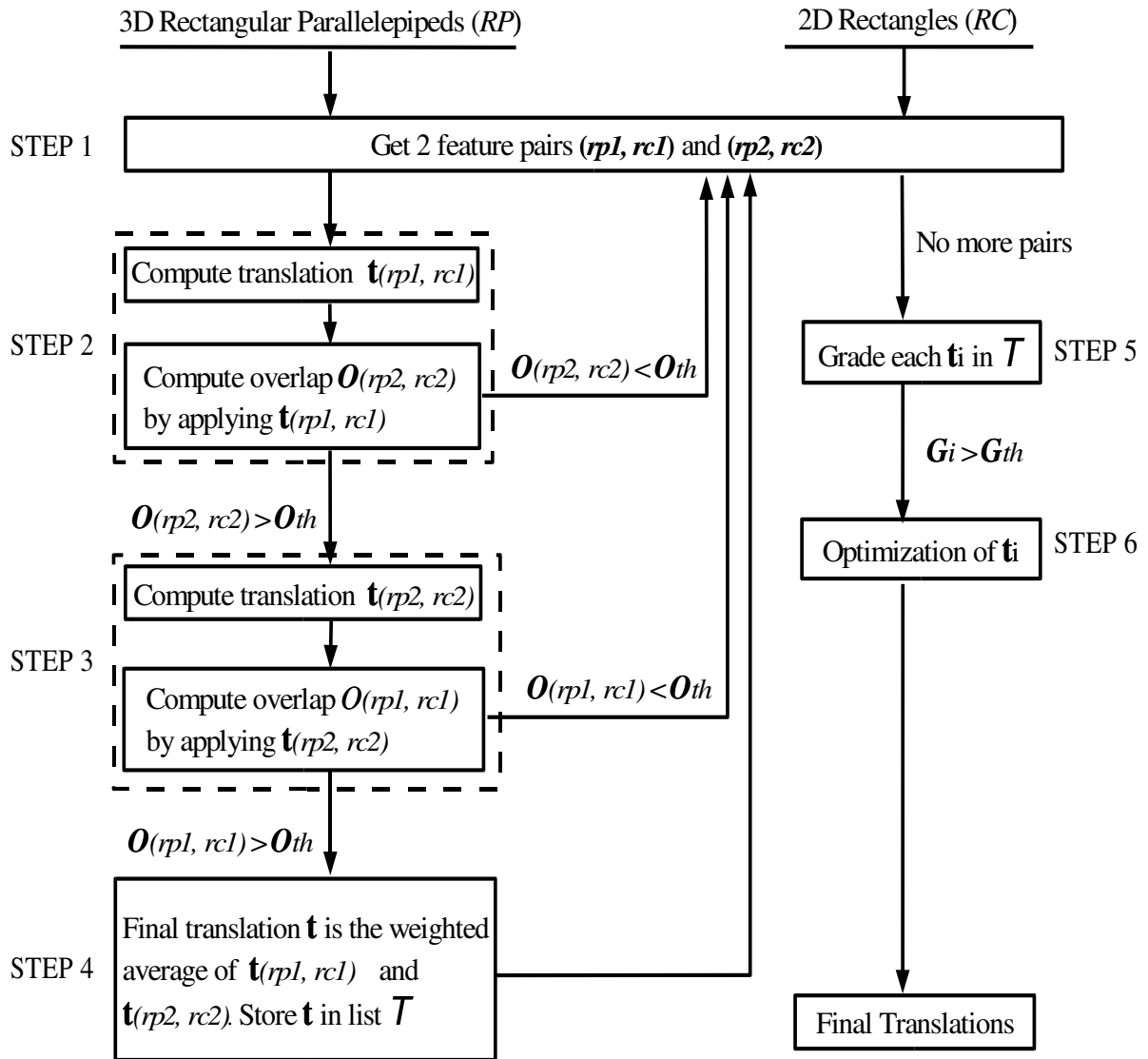
Figure 3.5: Translation computation algorithm outline.
