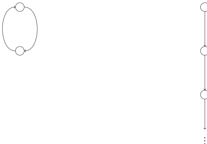
FIGURE 6. Alternative graphs of the set a = \{a\} .
