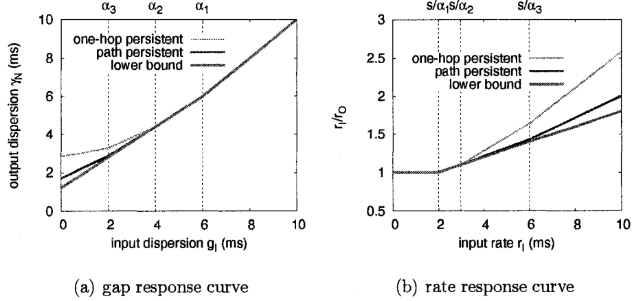
Figure 4.1: An example of multi-hop response curves.
