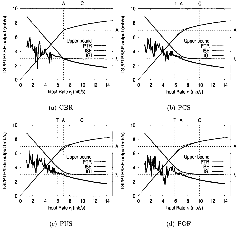
Figure 3.12: Trace driven testing of three estimators: IGI, PTR, and ISE: (a) using CBR, (b) using PCS, (c) using PUS, (d) using POF.
