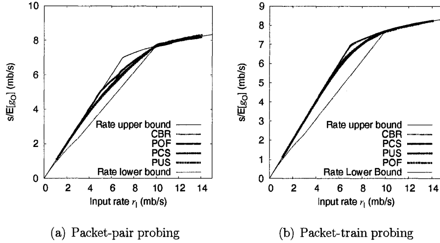
Figure 3.8: Rate response curve for the four cross-traffic traces: (a) probing pairs, (b) 16-packet trains (probing packet size 750 bytes).
