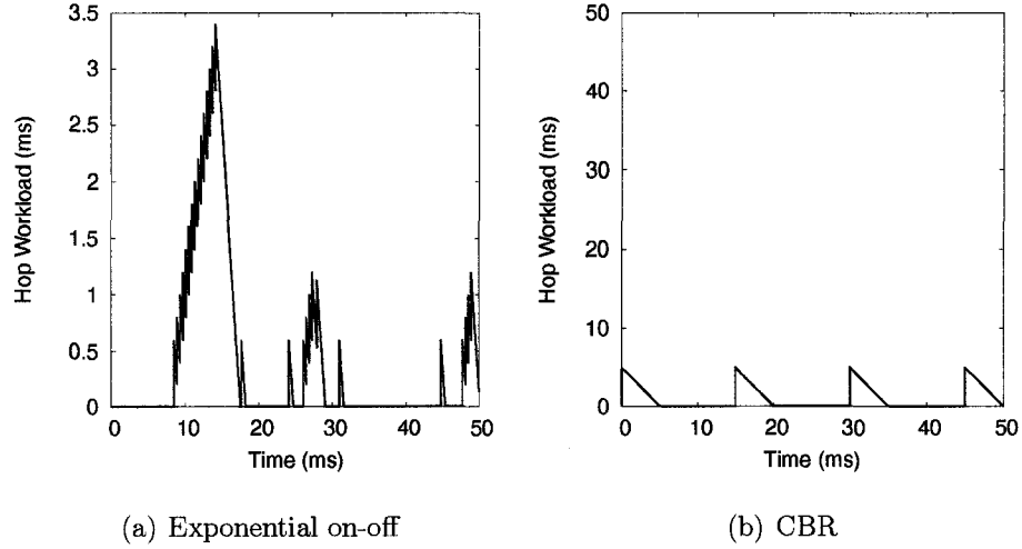
Figure 3.2: (a) The first 50 ms of the workload sample-path W(t) of exponential on-off ns-2 traffic ( C = 10 mb/s, s = 750 bytes); (b) Hop workload W(t) of CBR ns-2 traffic ( C = 2.4 mb/s, s = 1500 bytes).
