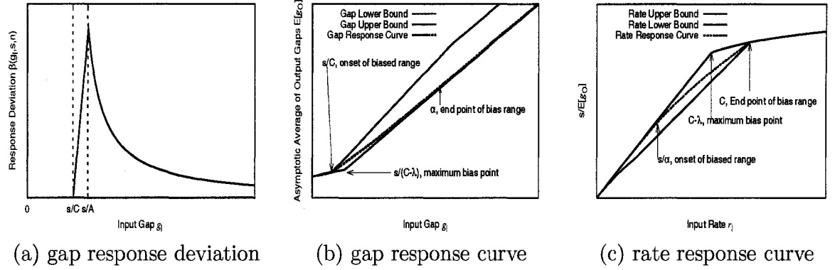
Figure 3.4: Illustrations of (a) the gap response deviation, (b) gap response curve, and (c) rate response curve in the entire input range.
