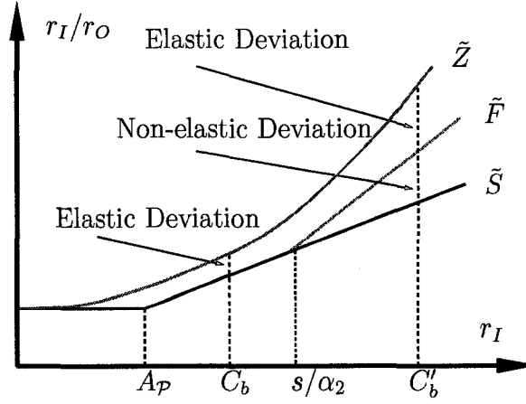
Figure 4.5: Illustration of two types of curve deviations.
