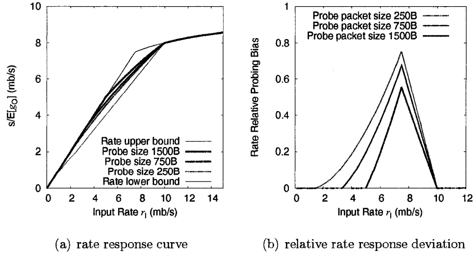
Figure 3.5: Packet pair probing in CBR cross-traffic: (a) Rate response curves, (b) relative rate response deviation. C=10\text{mb/s} , \lambda=2.5\text{mb/s} .
