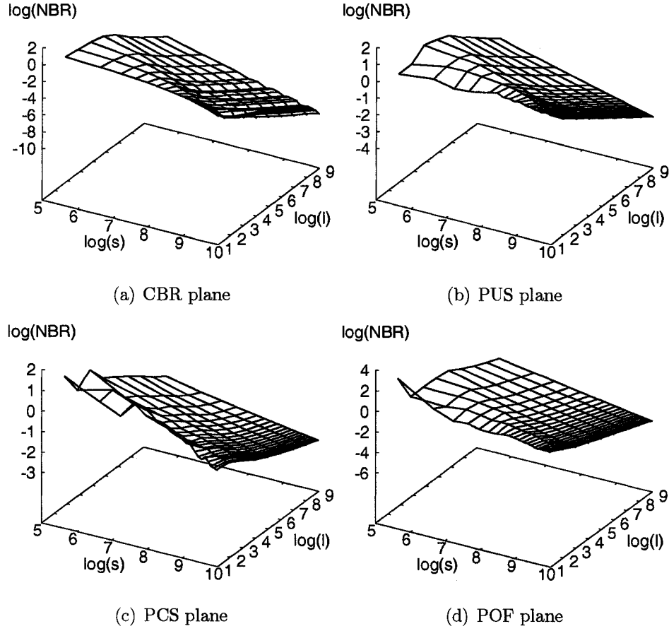
Figure 3.10: \text{NBR}(s, l) for four types of cross-traffic on log-log scale.
