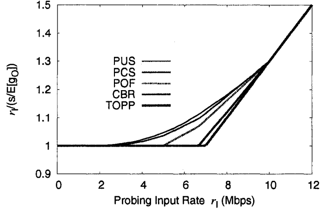
Figure 3.11: TOPP-transformed rate response curves.
