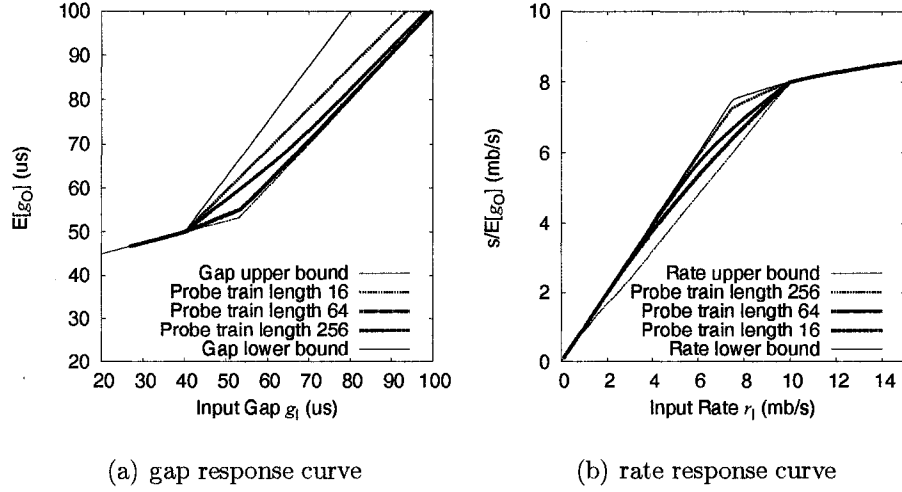
Figure 3.6: Packet train probing in CBR traffic: (a) Gap response curves, and (b) rate response curves. C=10\text{mb/s} , \lambda=2.5\text{mb/s} .
