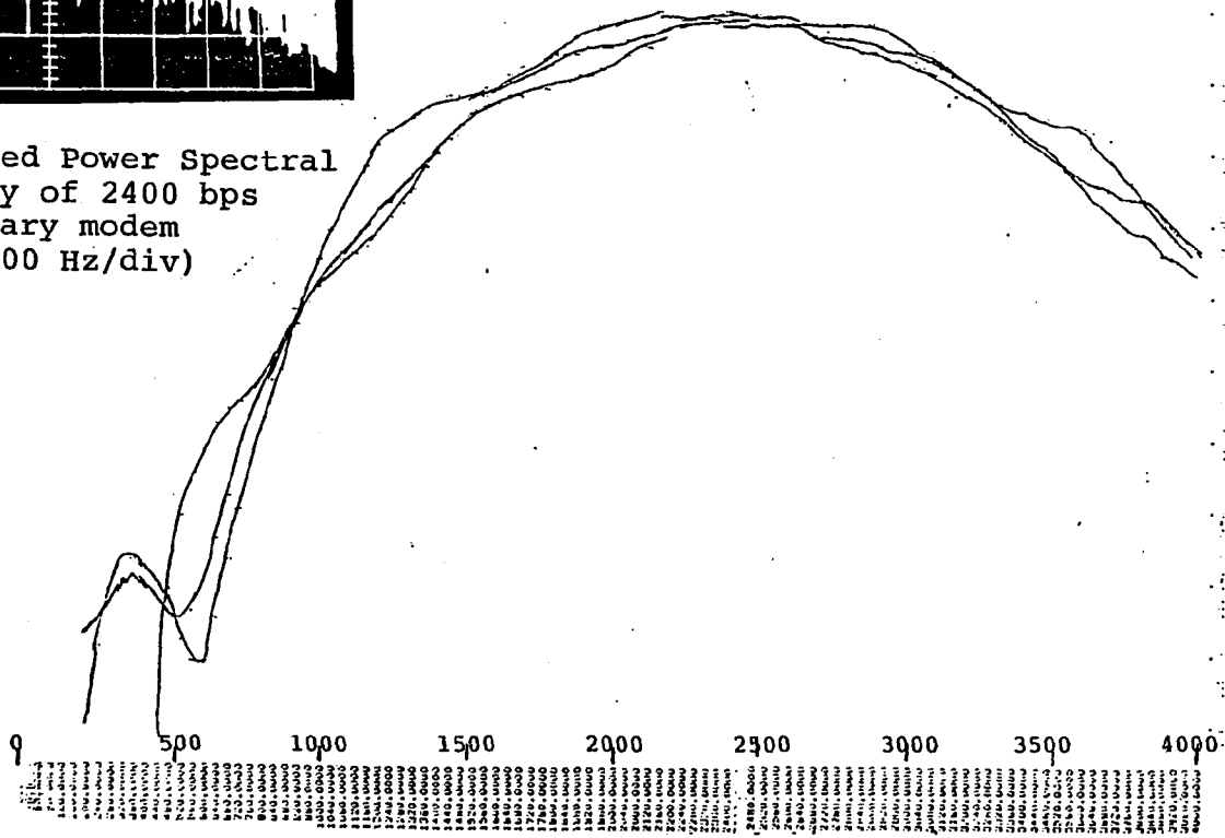
Figure 5.4.7 Calculated PSD of 2400 bps duobinary modem
