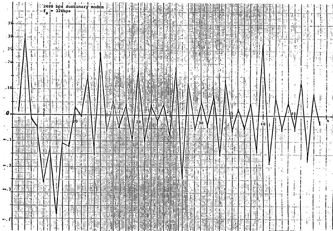
Figure 5.4.6 Measured autocorrelation of 2400bps duobinary modem using time averaging techniques
