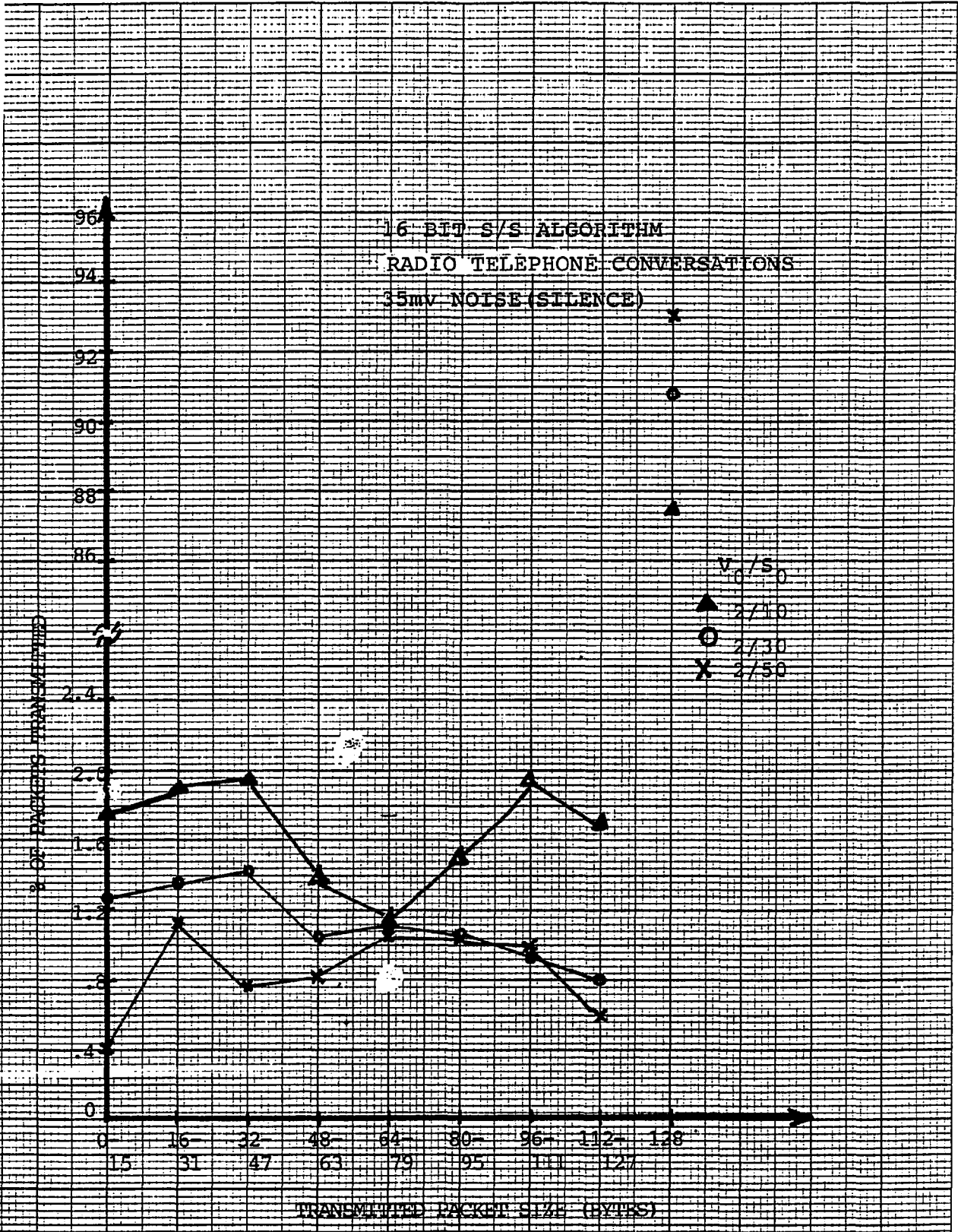
FIGURE 4.5a Transmitted packet statistics for radio telephone conversations (35mv noise)
