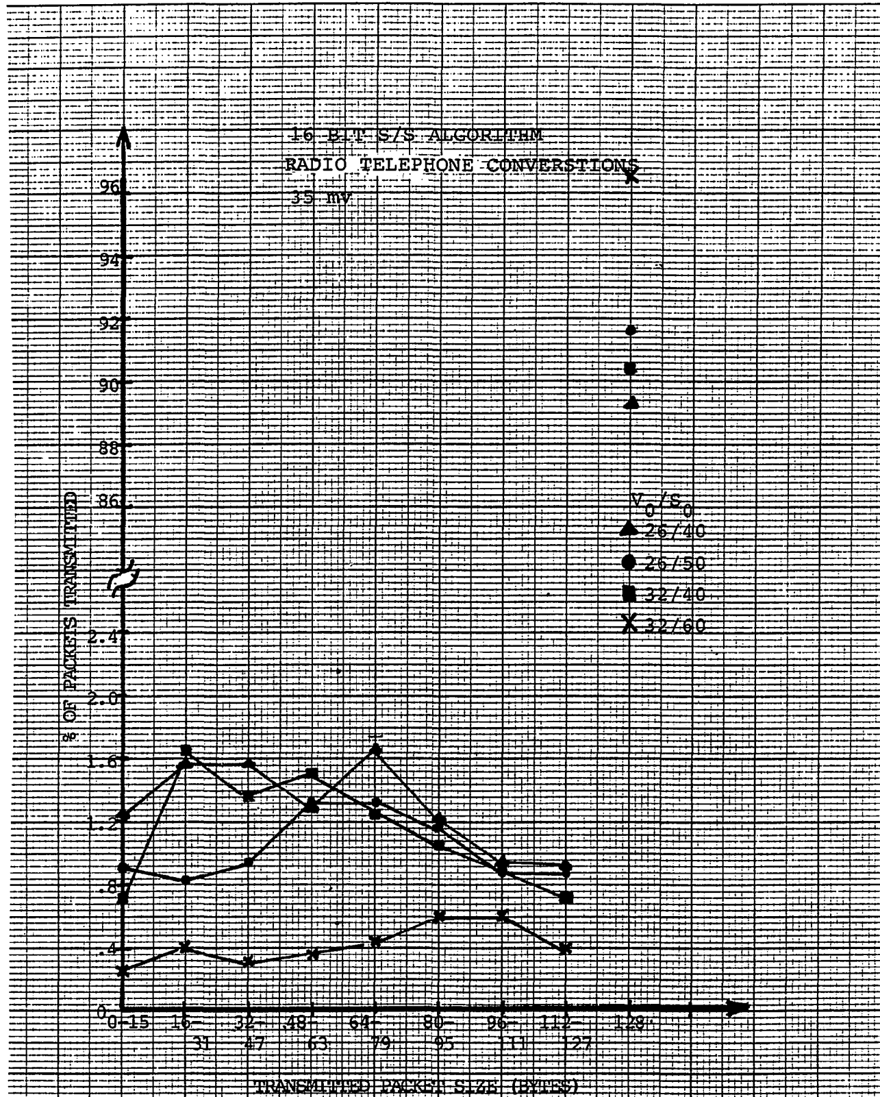
Figure 4.5c Transmitted packet statistics for radio telephone conversations (35mV noise)
