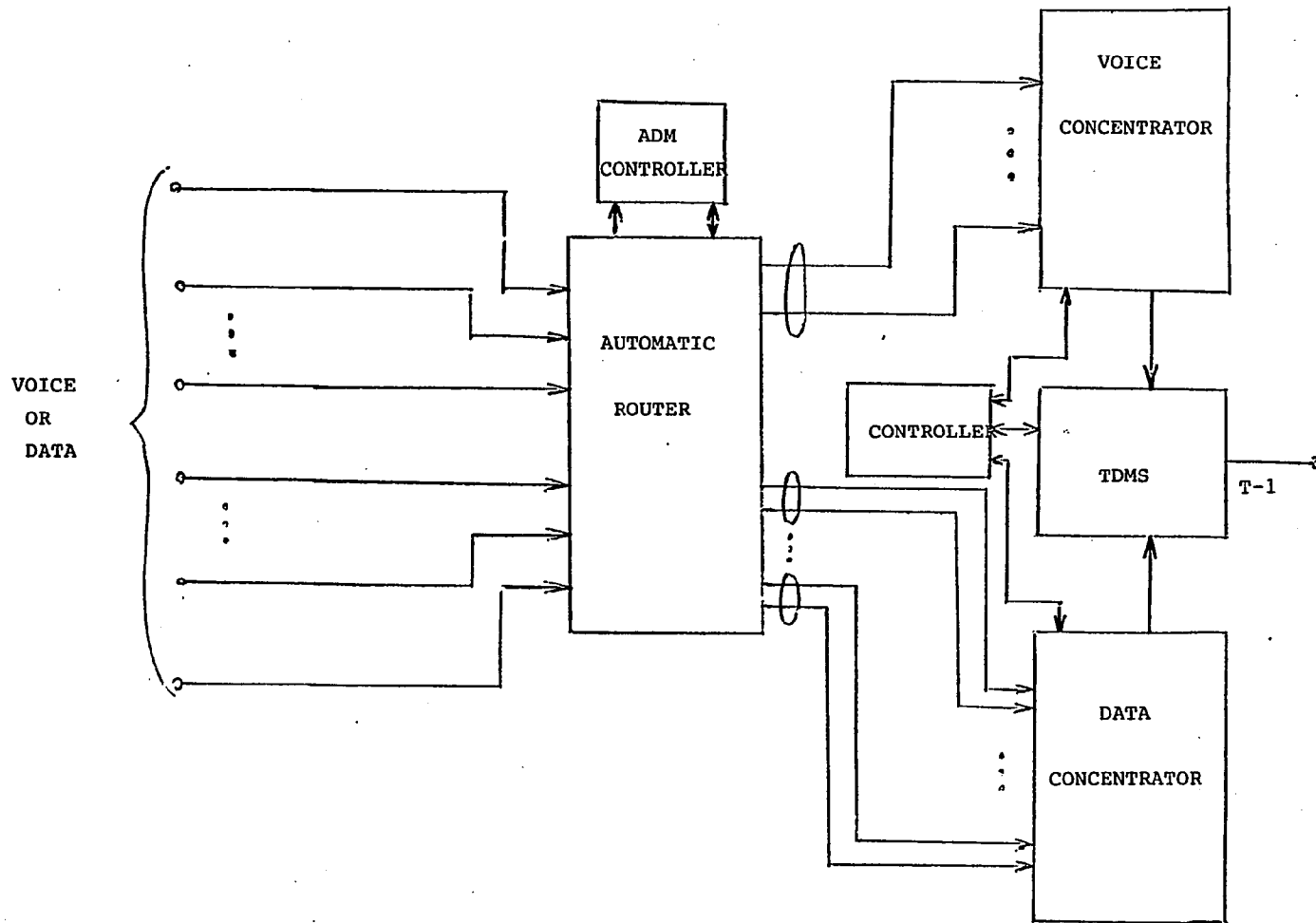
Figure 5.7.2 Proposed Automatic routing telephone system
