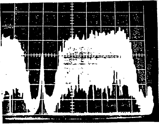
Measured Power Spectral Density of 9600 bps 16-QAM modem (500 Hz/div)
