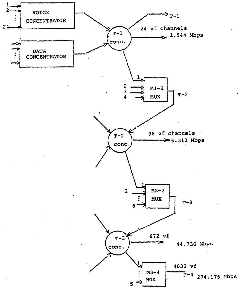
Figure 5.3.3 Hierarchy of digital telephone transmission in the USA
