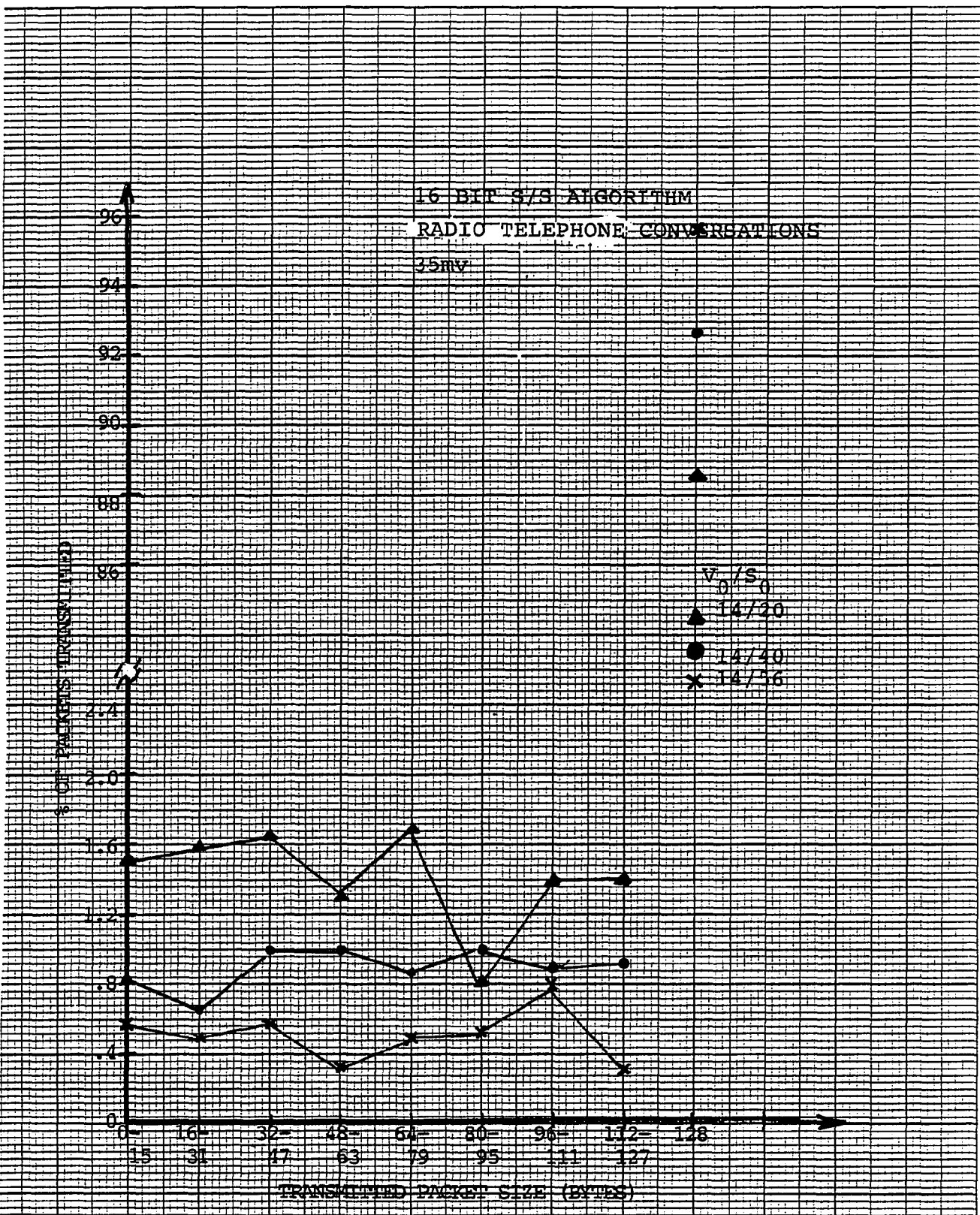
FIGURE 4.5b Transmitted packet statistics for radio telephone conversations (35mv noise)
