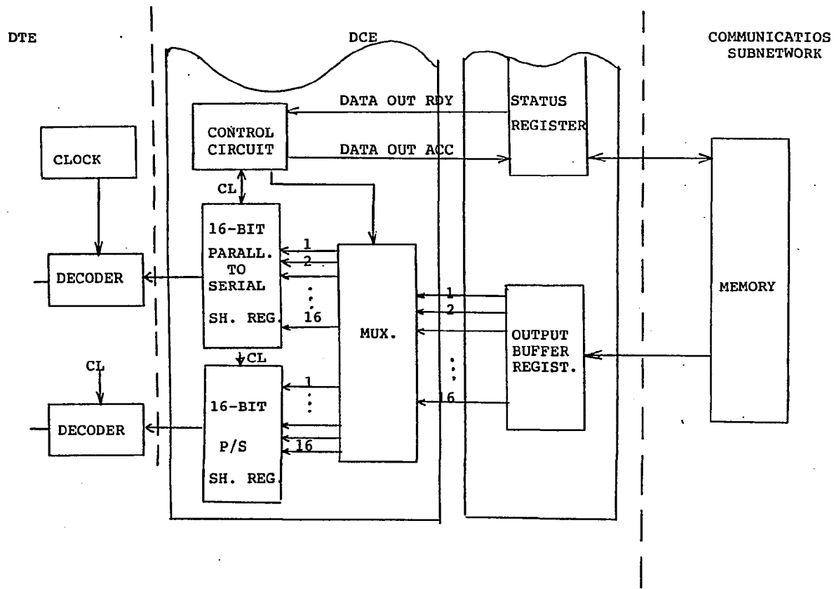
Figure 2.3.1.2 Configuration for data output from PVNS
