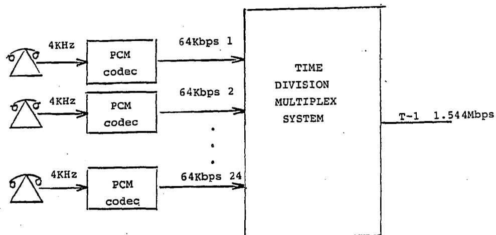
a) Voice Concentrator
