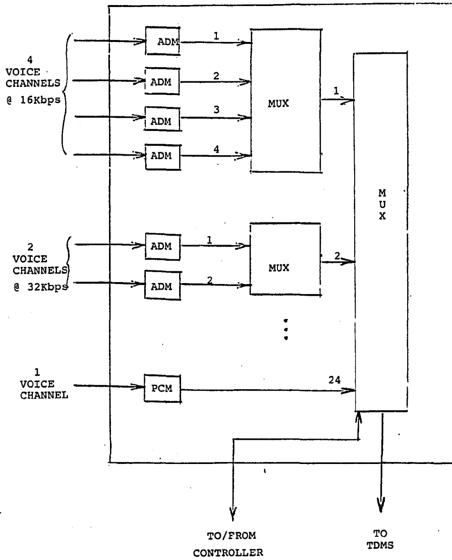
Figure 5.7.2.1 Speech concentrator
