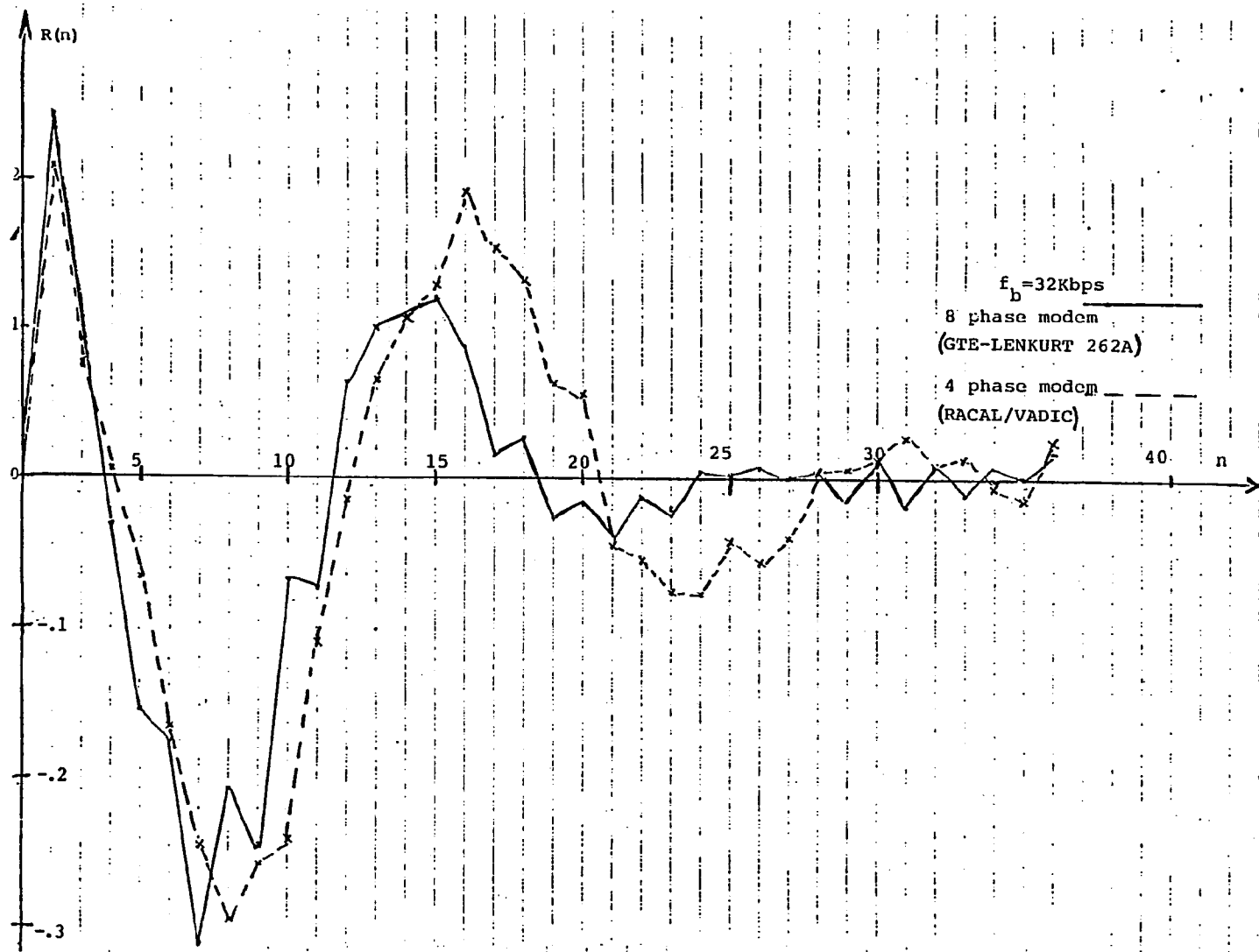
Figure 5.4.1 Autocorrelation of DM digital output sampling 4phase and an 8phase modems
