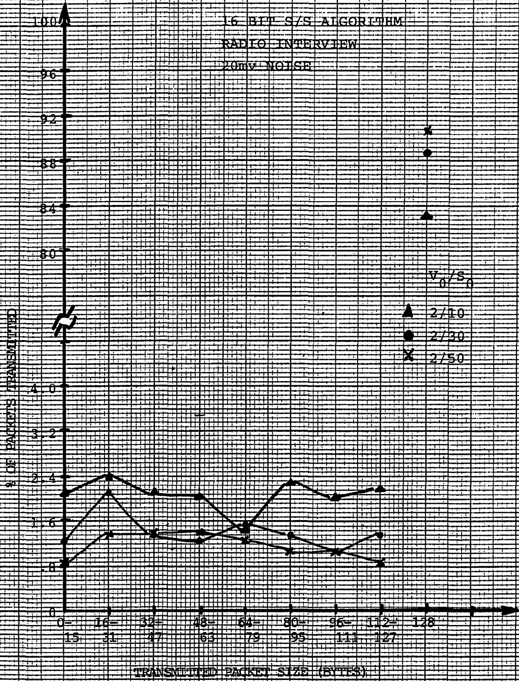
FIGURE 4.1a Transmitted packet statistics for radio interview (20mv noise)
