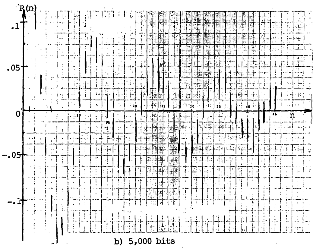
Figure 5.4.9 Autocorrelation of 9600 bps WESTERN ELECTRIC modem sampled at 32 Kbps using time averaging techniques with a) 10,000 bits and b) 5,000 bits
