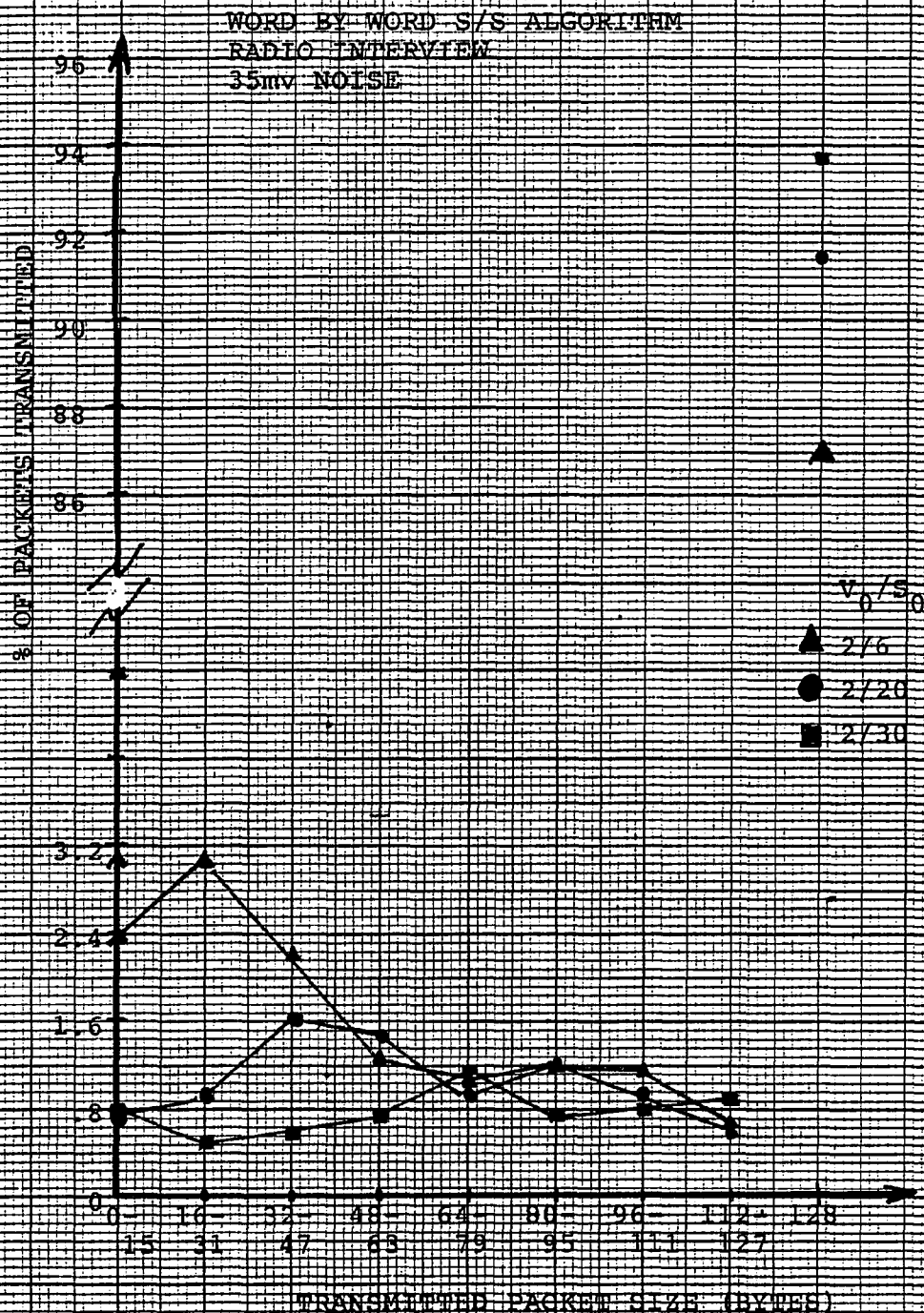
FIGURE 4.7a Transmitted packet statistics for radio interview (35mv noise) word-by-word algorithm
