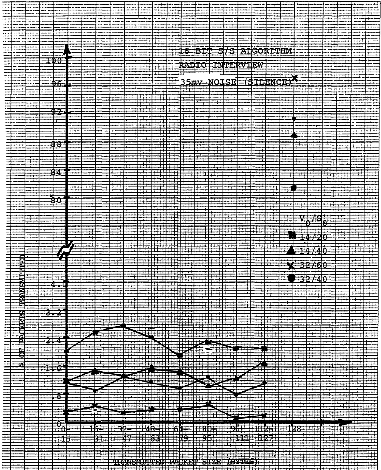
FIGURE 4.3b Transmitted packet statistics for radio interview (35mv noise)
