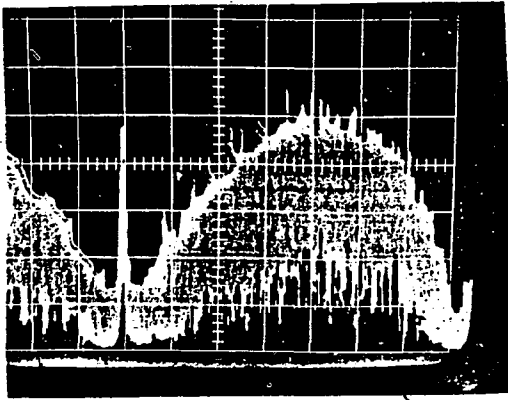
Measured Power Spectral Density of 4800 bps 8-PSK modem (500 Hz/div)
