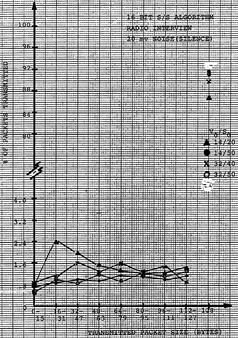
FIGURE 4.1b Transmitted packet statistics for radio interview (20mv noise)
