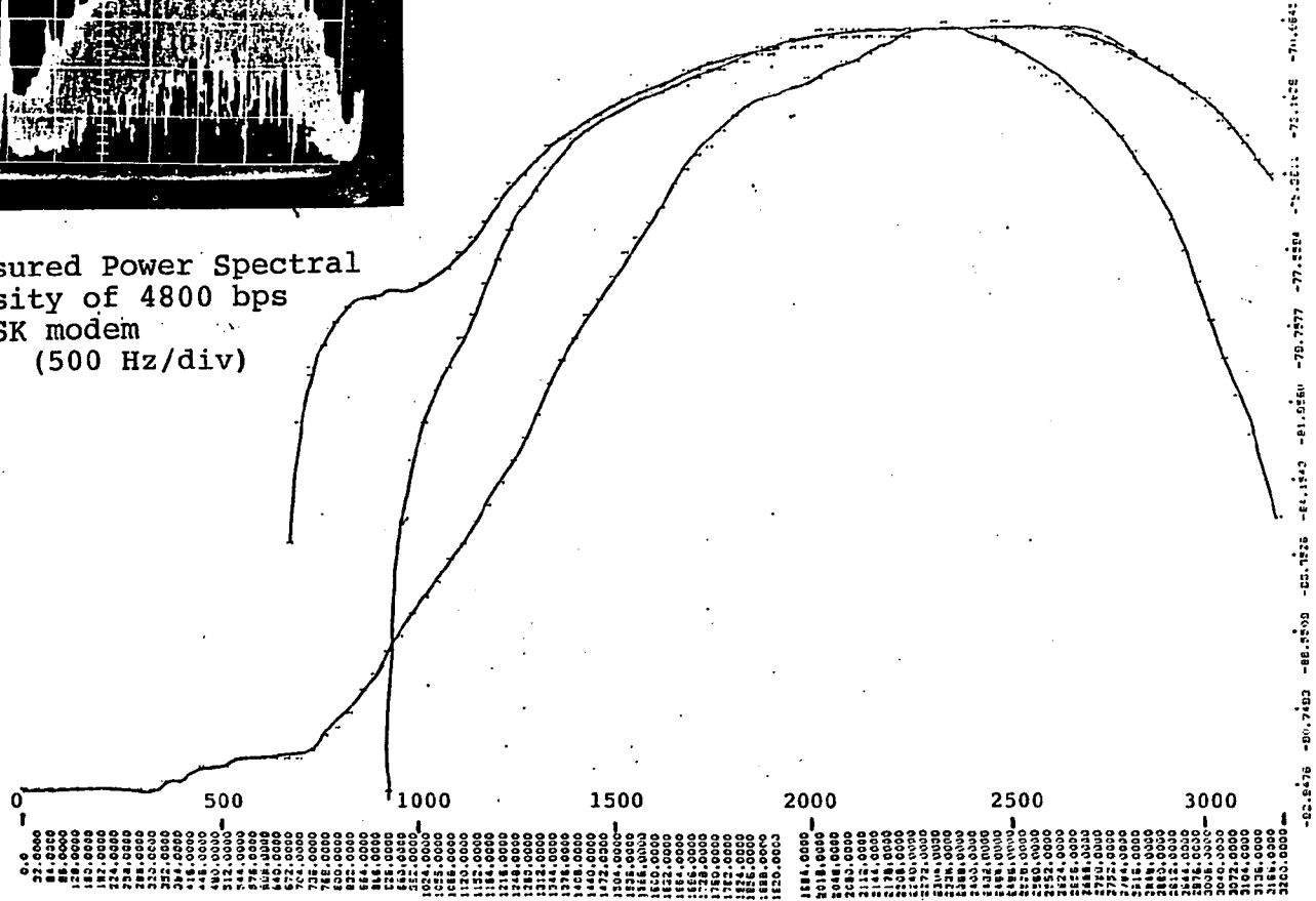
Figure 5.4.4 Calculated PSD of 4800bps 8-PSK modem
